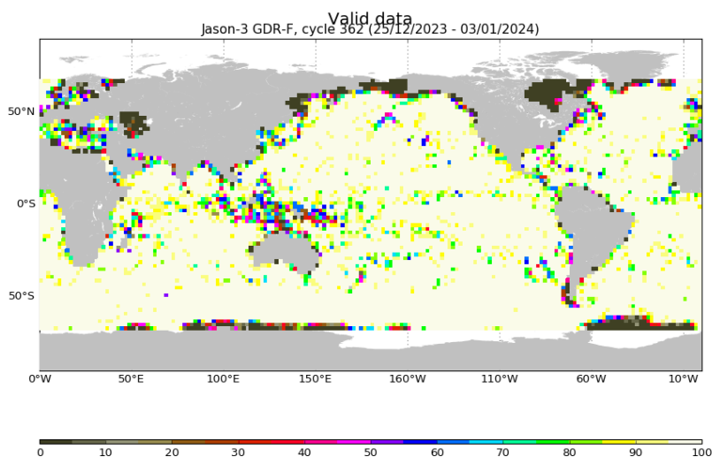
FIGURE 3 – Percentage of valid measurements for cycle 362.
