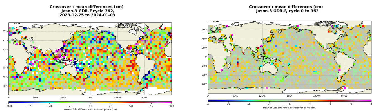
FIGURE 13 – Mean SSH at crossovers for cycle 362 (left) and over the whole Jason-3 period (right).
