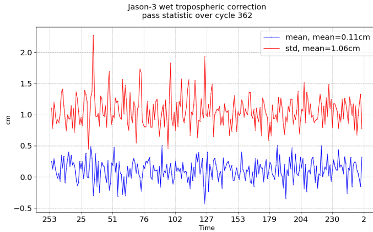
FIGURE 11 – Pass monitoring of wet troposphere differences between radiometer and ECMWF model for Jason-3 cycle 362
