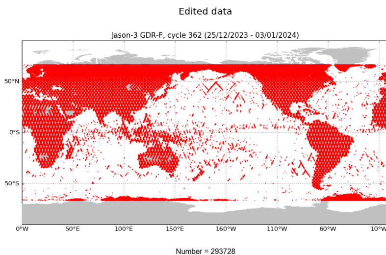
FIGURE 2 – Edited measurements for cycle 362.
