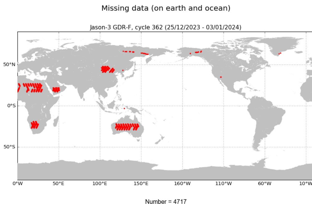
FIGURE 1 – Missing measurements for cycle 362.
