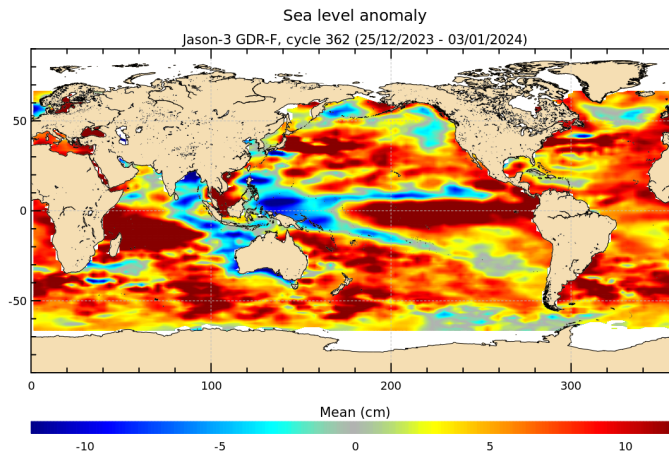
FIGURE 18 – Sea level anomaly relative to MSS for cycle 362.
