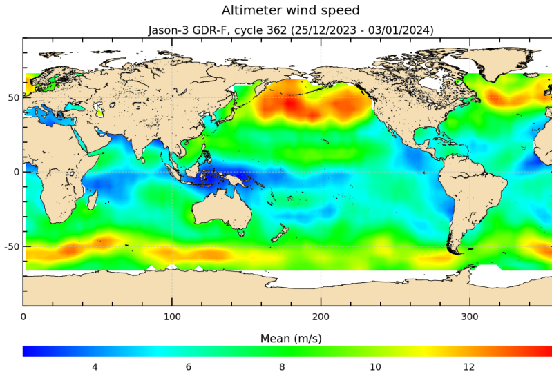
FIGURE 9 – Altimeter wind speed for cycle 362.
