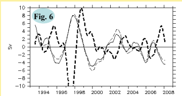
Fig.6: Thin line: Time evolution of transport anomalies entering the Solomon Sea as deduced by SLA differences between the two red points in Fig.5. Dash line: Transport anomalies estimated at both Vitiaz and Solomon straits. Thick dash line: dWWVw/dt.
