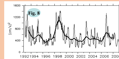
Fig. 8: Time evolution of the EKE signal averaged on the Solomon Sea. Unit in (cm/s) 2 . Thin line: raw data, Thick line: high frequencies filtered
