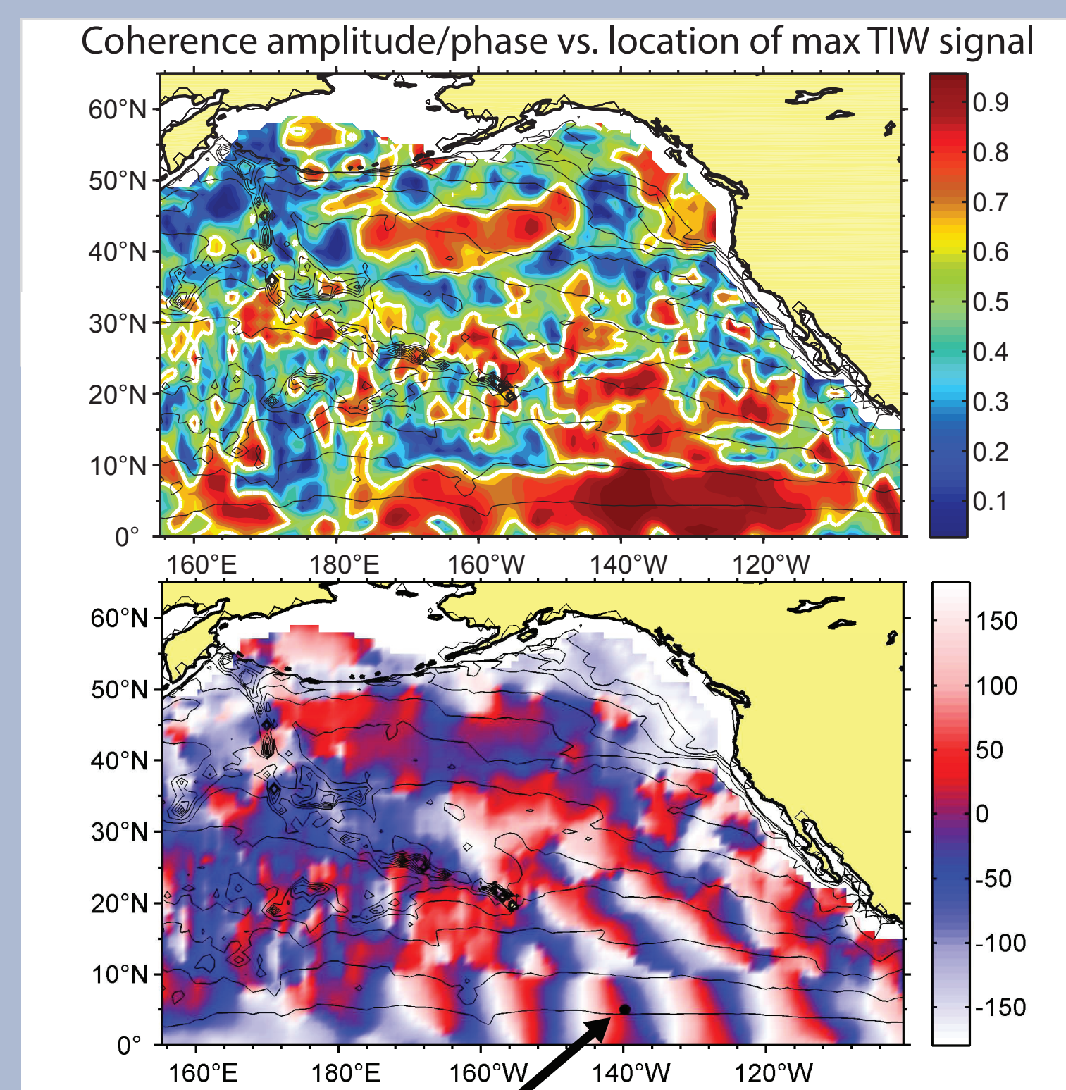
Maps of coherence amplitude (top) and phase (bottom) of SSH with the 30-day SSH signal at 5°N, 140°W (location of max TIW signal).
