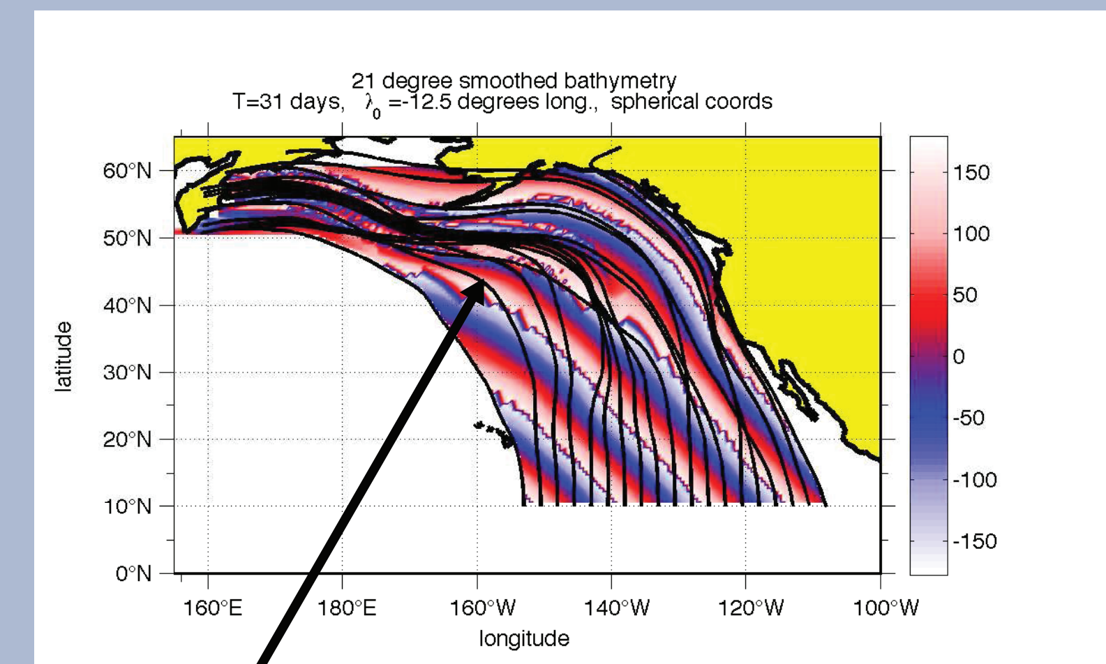
Convergence of rays, which implies increasing wave amplitude, roughly corresponds to region of elevated variance in SSH at 30-day periods (panel 2 above)
