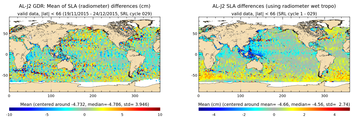
FIGURE 22 – Saral/AltiKa – Jason-2 SLA differences for cycle 029 (left) and averaged over the whole Saral/AltiKa period (right)
