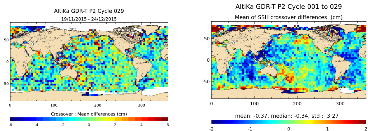
FIGURE 15 – Mean SSH at crossovers for cycle 029 (left) and over the whole Saral/AltiKa period (right).
