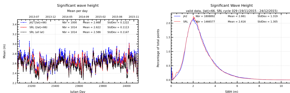
FIGURE 8 – Daily monitoring of significant wave height for AltiKa (Ka-band) and Jason-2 (Ku-band) on the left and histogram for cycle 029 on the right (limited to 66° latitude).
