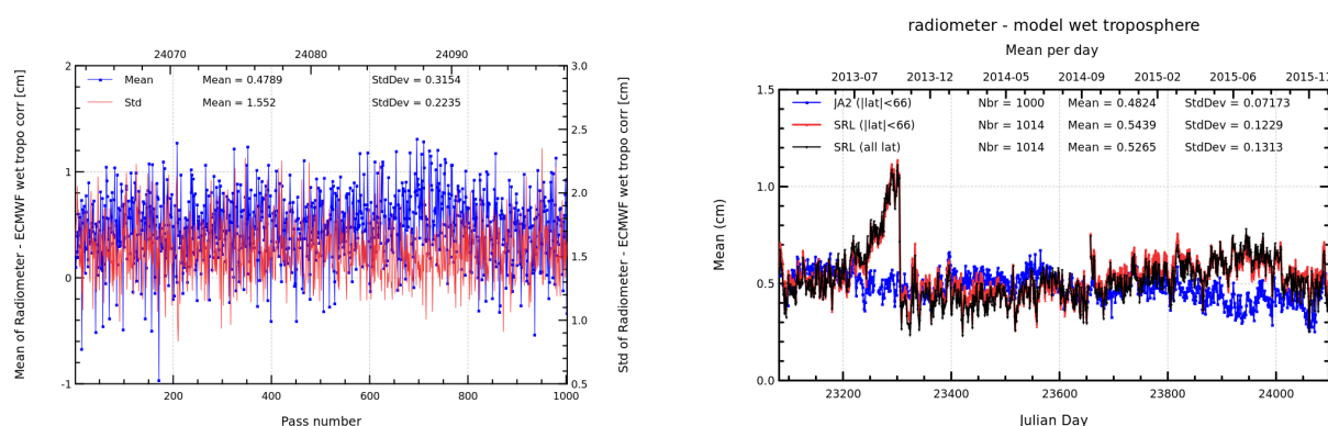
FIGURE 13 – Pass monitoring of wet troposphere differences between radiometer and ECMWF model for Saral/AltiKa cycle 029 (left) and daily monitoring of wet troposphere differences between radiometer and ECMWF model (right).
