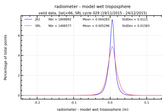
FIGURE 14 – Histogram of wet troposphere differences between radiometer and ECMWF model for cycle 029.
