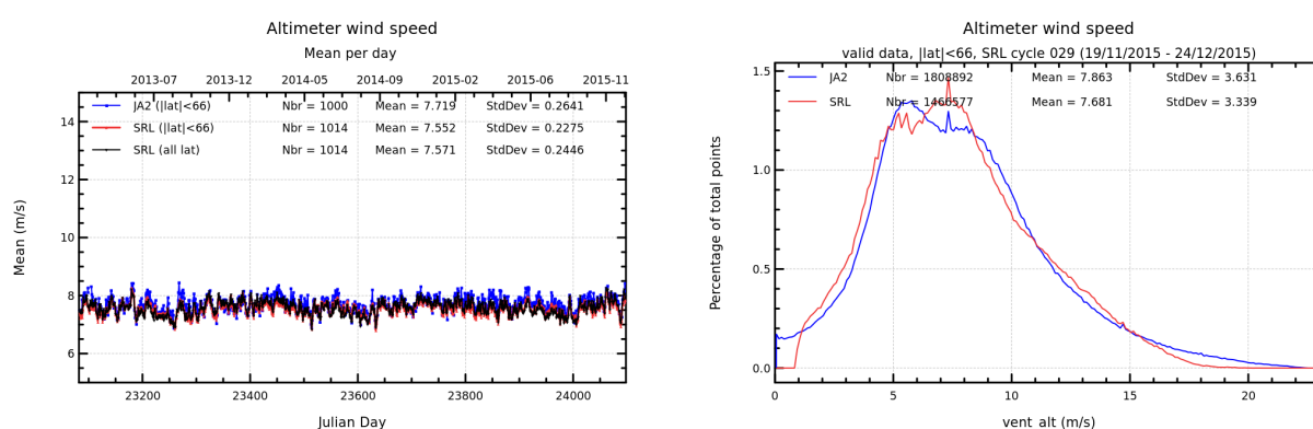
FIGURE 12 – Daily monitoring of altimeter wind speed for Saral/AltiKa and Jason-2 on the left and histogram for cycle 029 on the right (limited to 66^\circ latitude).
