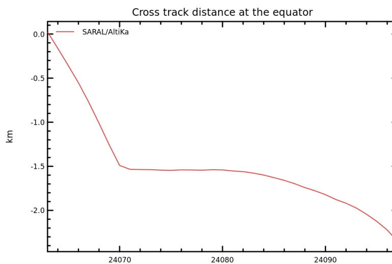
FIGURE 3 – CrossTrack distance at the equator cycle 29.
