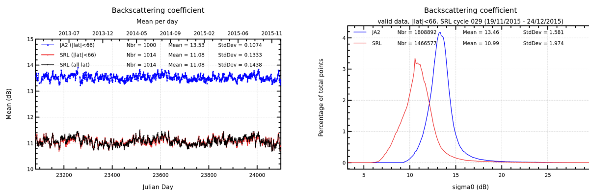
FIGURE 9 – Daily monitoring of backscattering coefficient for Saral/AltiKa and Jason-2 on the left and histogram for cycle 029 on the right (limited to 66° latitude).
