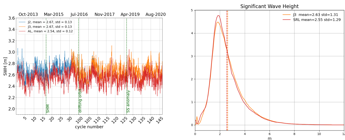
Figure 6: Daily monitoring of significant wave height for AltiKa (Ka-band) Jason-2 and Jason-3 (Ku-band) on the left and histogram for cycle 146 on the right (limited to 66^\circ latitude).
