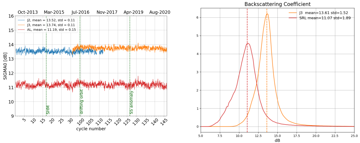
Figure 7: Daily monitoring of backscattering coefficient for Saral/AltiKa, Jason-2 and Jason-3 on the left and histogram for cycle 146 on the right (limited to 66° latitude).
