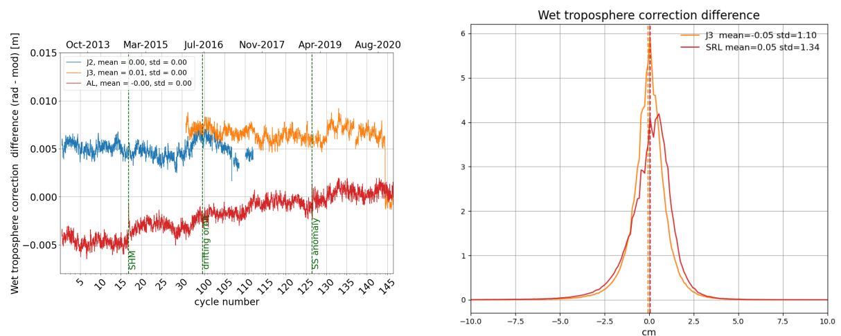
Figure 12: Daily monitoring of wet troposphere differences (Radiometer-ECMWF model) for Saral/AltiKa Jason-2 and Jason-3 (left) and histogram on the right (limited to 66° latitude) for cycle 146 .
