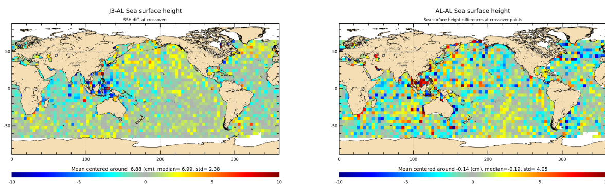
Figure 14: Mean of multi-mission SSH and mono-mission SSH differences at crossovers for cycle 146.
