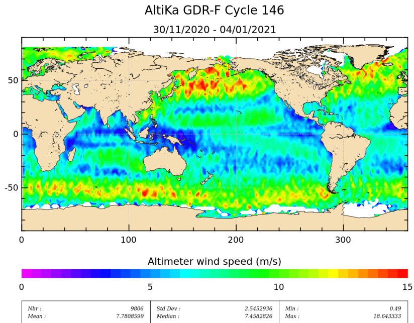
Figure 9: Altimeter wind speed for cycle 146.
