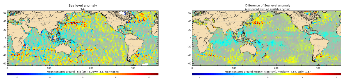
Figure 21: Jason-3 — Saral/AltiKa SLA differences for cycle 146 (left) and averaged over the whole Saral/AltiKa period (right).
