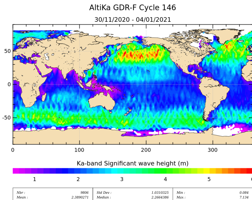
Figure 5: Significant wave height for cycle 146.
