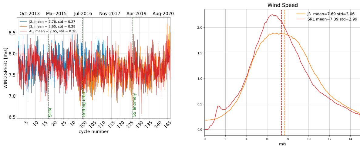
Figure 10: Daily monitoring of altimeter wind speed for Saral/AltiKa, Jason-2 and Jason-3 on the left and histogram for cycle 146 on the right (limited to 66° latitude).
