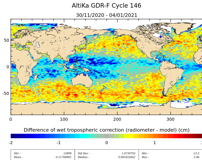
Figure 11: Mean of wet troposphere correction difference (Radiometer-ECMWF model)for cycle 146.
