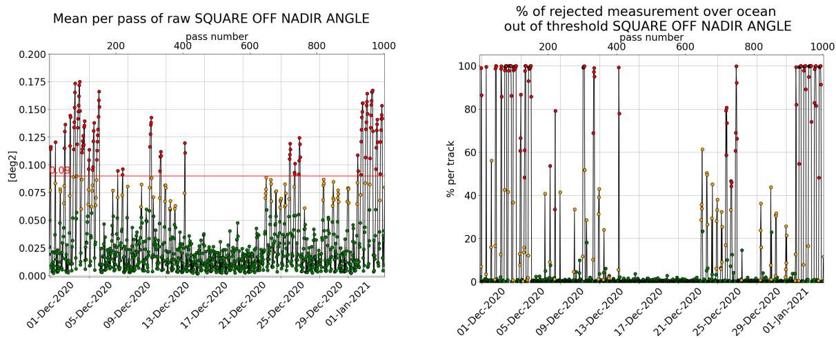
Figure 3: [left] Mispointing cycle 146, [right] Percentage of rejected measurement by threshold on square off-nadir angle.
