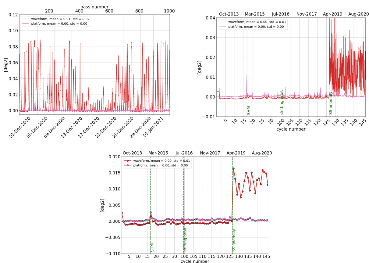
Figure 13: Monitoring per pass for cycle 146 (left), daily monitoring(right) and cyclic monitoring (bottom) of SARAL/AltiKa's mispointing angle: comparison between the one derived from waveform retracking and the one measured by platform startrackers.
