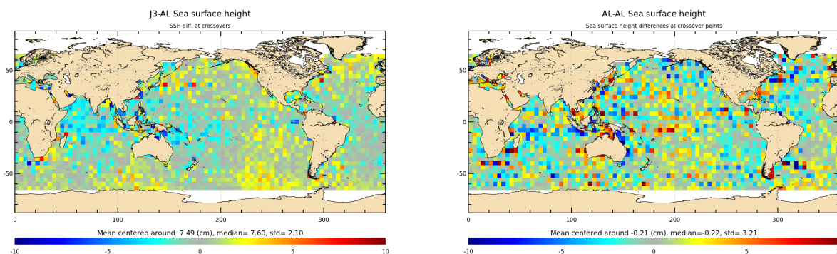
Figure 14: Mean of multi-mission SSH and mono-mission SSH differences at crossovers for cycle 190.
