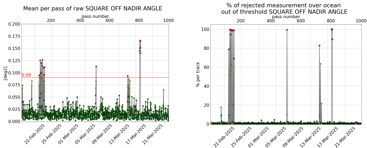
Figure 3: [left] Mispointing cycle 190, [right] Percentage of rejected measurement by threshold on square off-nadir angle.
