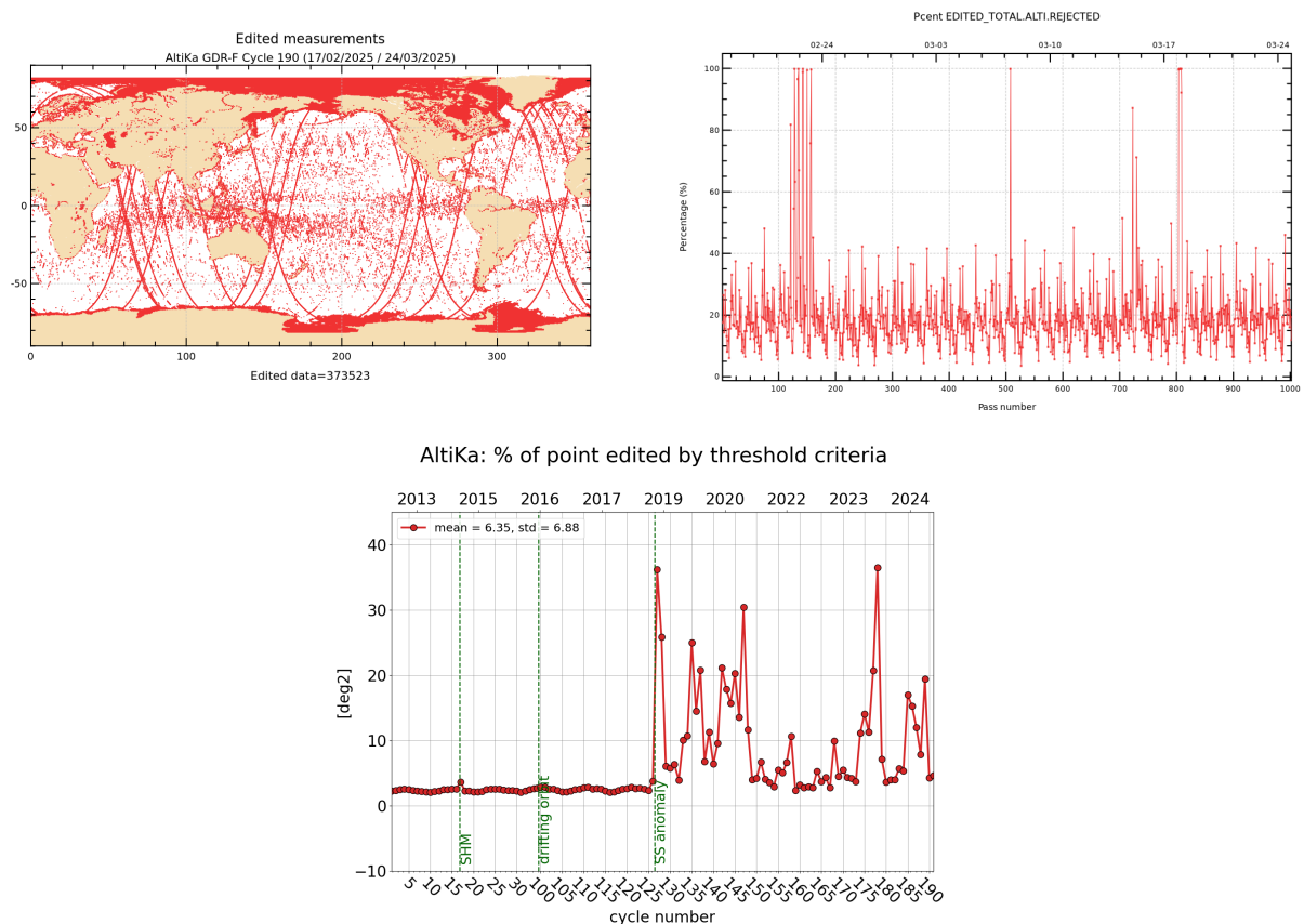
Figure 2: Rejected measurements on thresholds criteria : Cycle 190, map and monitoring of % of rejected measurements per track (top), whole time serie / % of rejected measurements per cycle (bottom).
