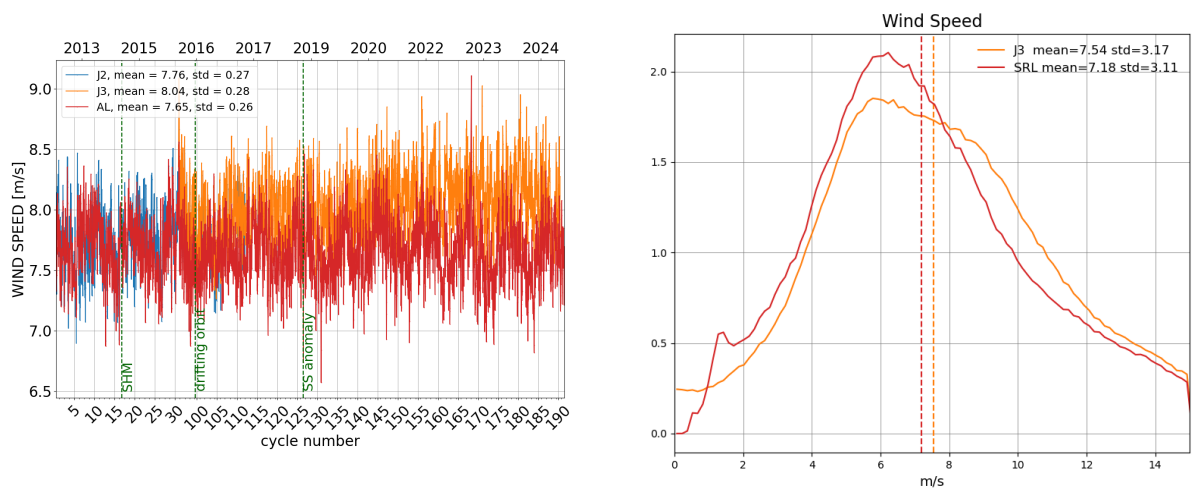
Figure 10: Daily monitoring of altimeter wind speed for Saral/AltiKa, Jason-2 and Jason-3 on the left and histogram for cycle 190 on the right (limited to 66° latitude).
