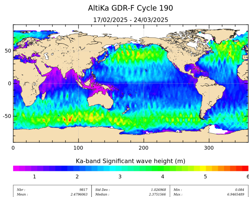
Figure 5: Significant wave height for cycle 190.
