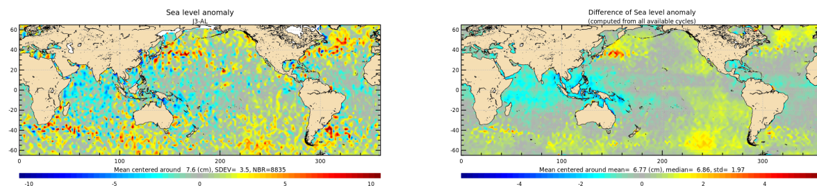
Figure 21: Jason-3 — Saral/AltiKa SLA differences for cycle 190 (left) and averaged over the whole Saral/AltiKa period (right).
