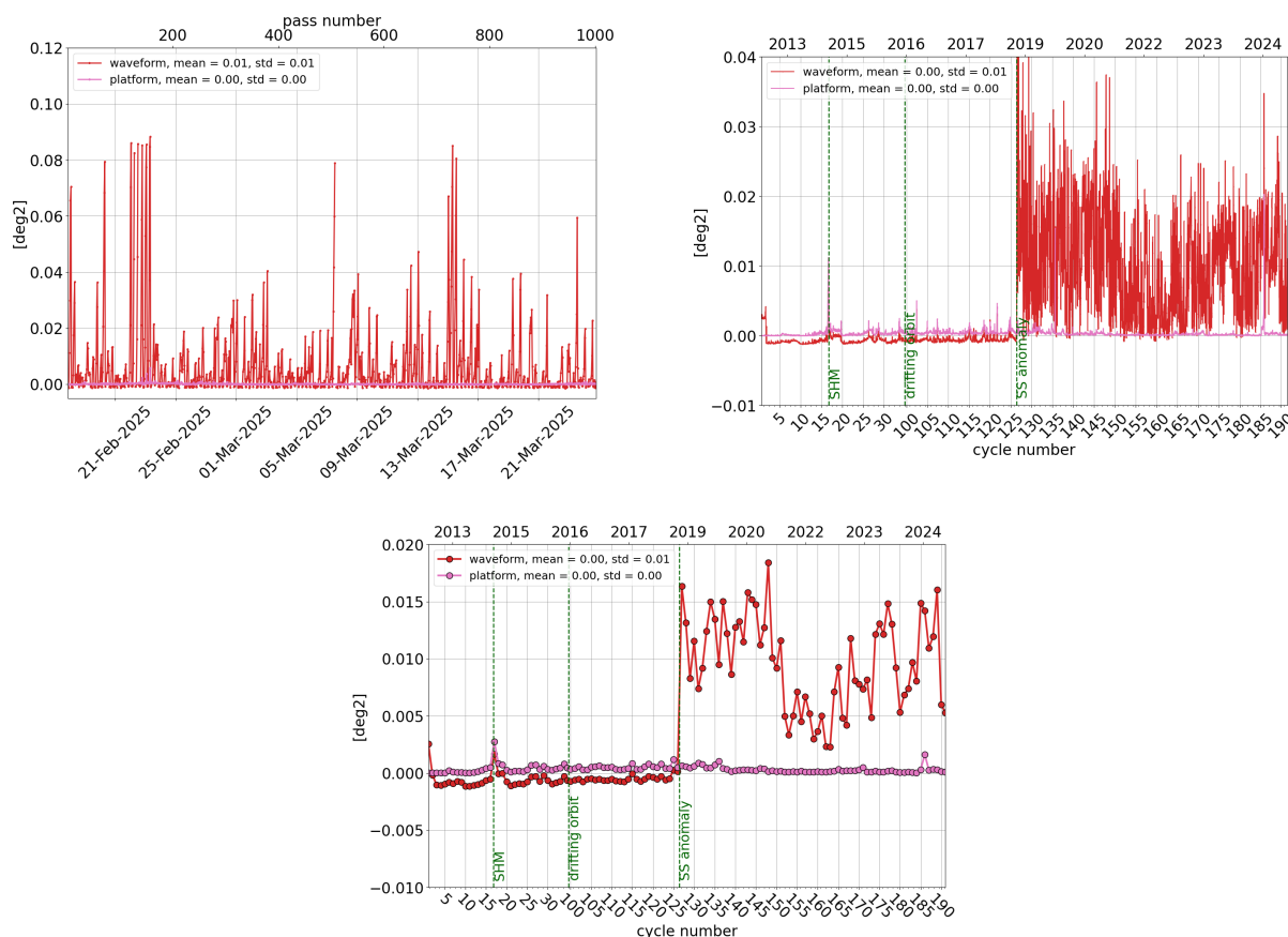
Figure 13: Monitoring per pass for cycle 190 (left), daily monitoring(right) and cyclic monitoring (bottom) of SARAL/AltiKa's mispointing angle: comparison between the one derived from waveform retracking and the one measured by platform startrackers.
