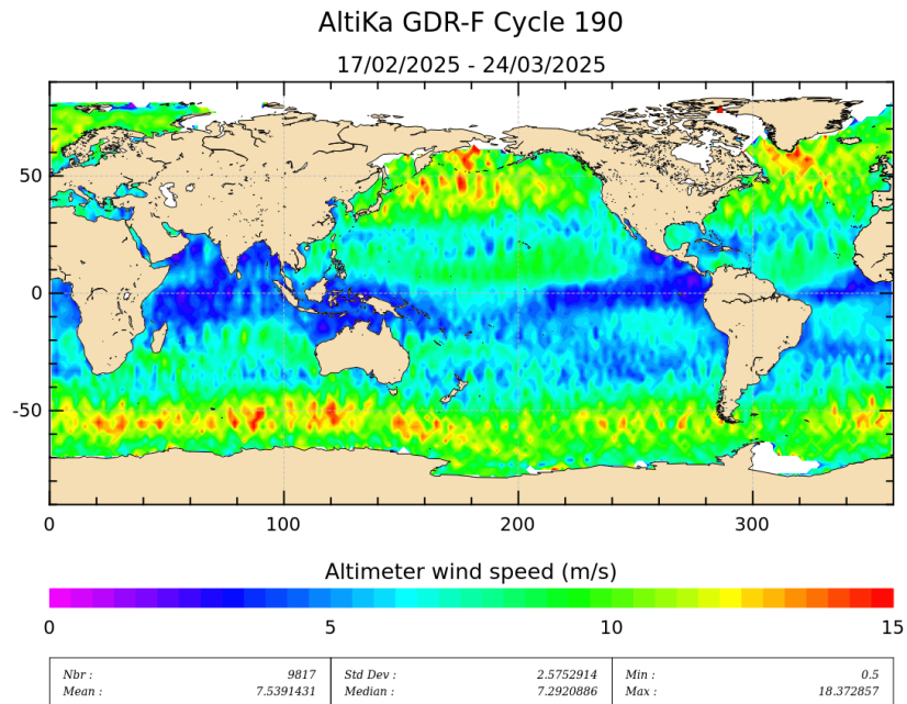
Figure 9: Altimeter wind speed for cycle 190.
