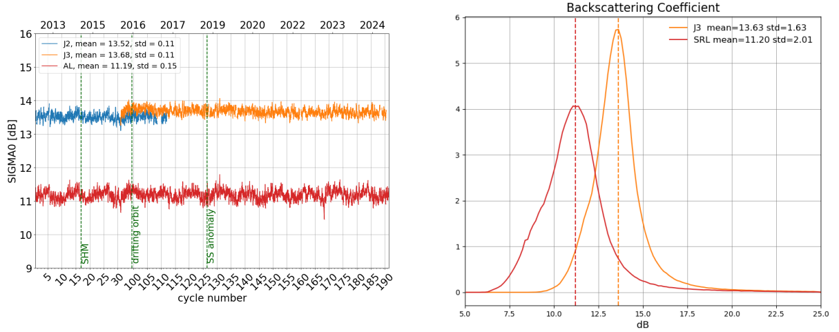
Figure 7: Daily monitoring of backscattering coefficient for Saral/AltiKa, Jason-2 and Jason-3 on the left and histogram for cycle 190 on the right (limited to 66° latitude).
