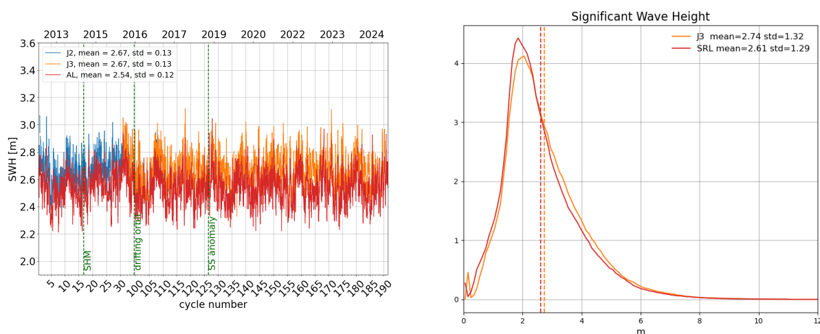
Figure 6: Daily monitoring of significant wave height for AltiKa (Ka-band) Jason-2 and Jason-3 (Ku-band) on the left and histogram for cycle 190 on the right (limited to 66^\circ latitude).
