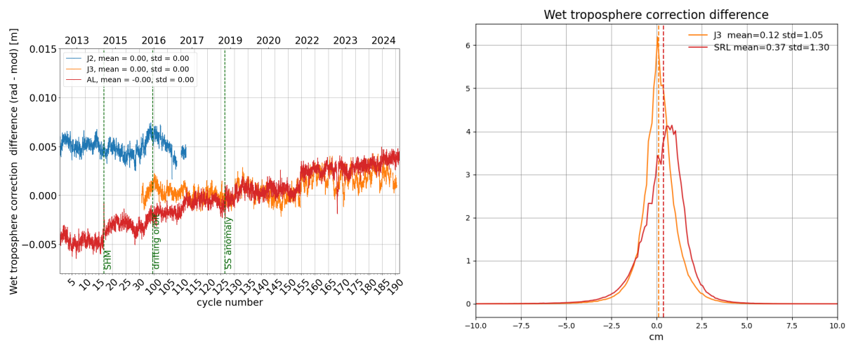
Figure 12: Daily monitoring of wet troposphere differences (Radiometer-ECMWF model) for Saral/AltiKa Jason-2 and Jason-3 (left) and histogram on the right (limited to 66° latitude) for cycle 190 .
