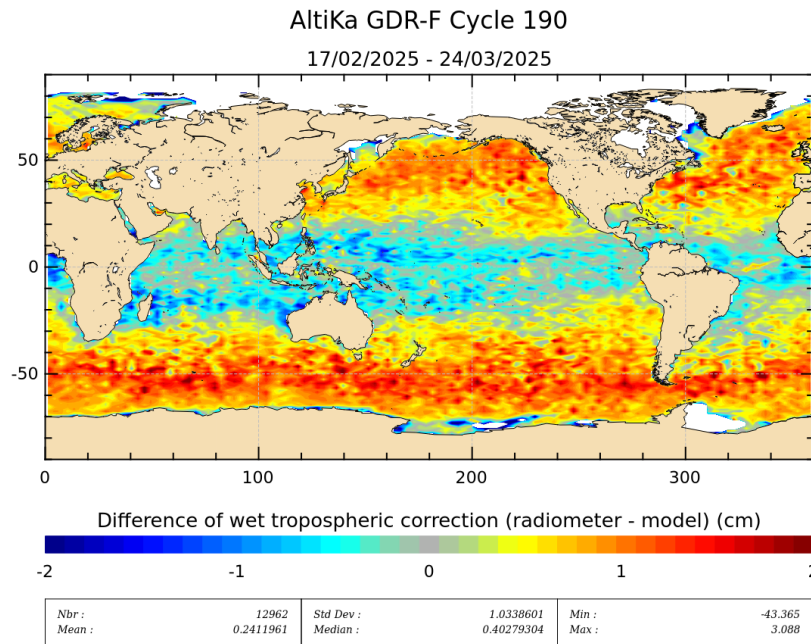
Figure 11: Mean of wet troposphere correction difference (Radiometer-ECMWF model)for cycle 190.
