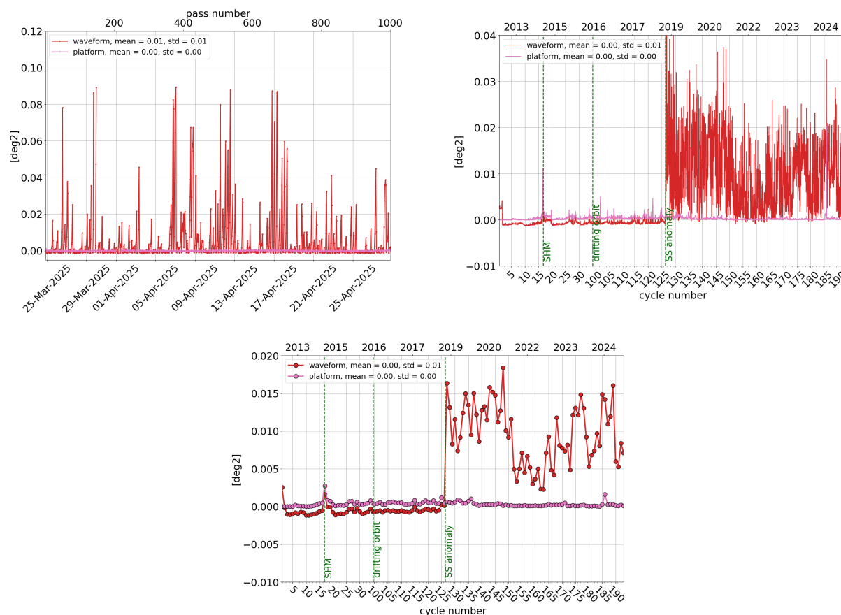
Figure 13: Monitoring per pass for cycle 191 (left), daily monitoring(right) and cyclic monitoring (bottom) of SARAL/AltiKa's mispointing angle: comparison between the one derived from waveform retracking and the one measured by platform startrackers.
