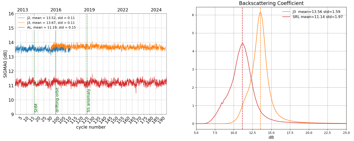
Figure 7: Daily monitoring of backscattering coefficient for Saral/AltiKa, Jason-2 and Jason-3 on the left and histogram for cycle 192 on the right (limited to 66° latitude).
