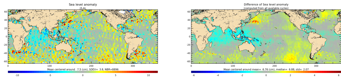
Figure 21: Jason-3 — Saral/AltiKa SLA differences for cycle 192 (left) and averaged over the whole Saral/AltiKa period (right).
