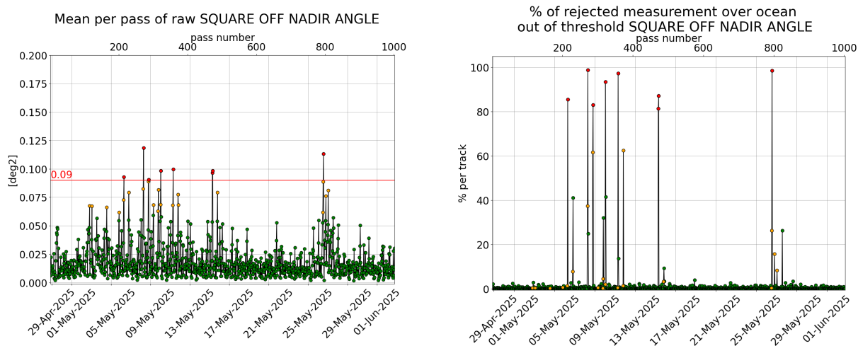
Figure 3: [left] Mispointing cycle 192, [right] Percentage of rejected measurement by threshold on square off-nadir angle.
