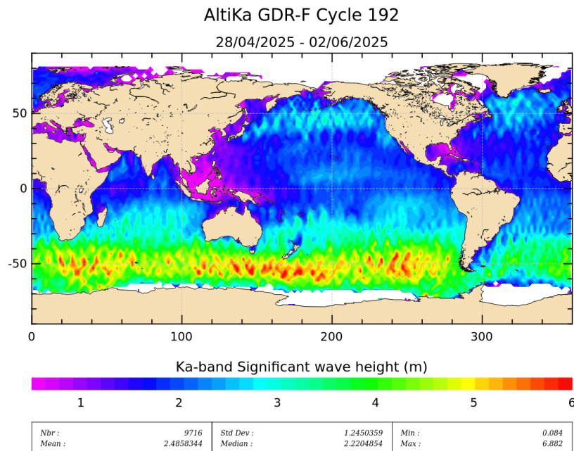
Figure 5: Significant wave height for cycle 192.
