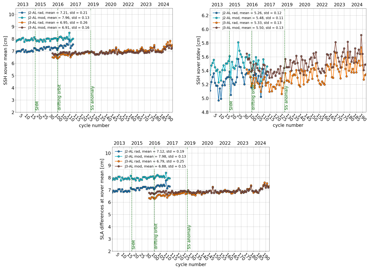
Figure 16: Cyclic monitoring of mean (left) and standard deviation (right) of Jason-2 / AltiKa & Jason-3 / AltiKa SSH differences at crossovers using geographical selections. Box-averaged SLA differences at crossovers (bottom).
