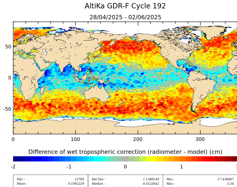
Figure 11: Mean of wet troposphere correction difference (Radiometer-ECMWF model)for cycle 192.
