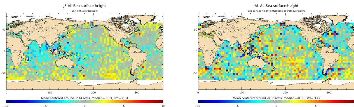
Figure 14: Mean of multi-mission SSH and mono-mission SSH differences at crossovers for cycle 192.
