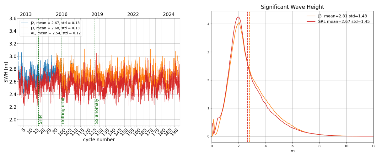
Figure 6: Daily monitoring of significant wave height for AltiKa (Ka-band) Jason-2 and Jason-3 (Ku-band) on the left and histogram for cycle 192 on the right (limited to 66^\circ latitude).
