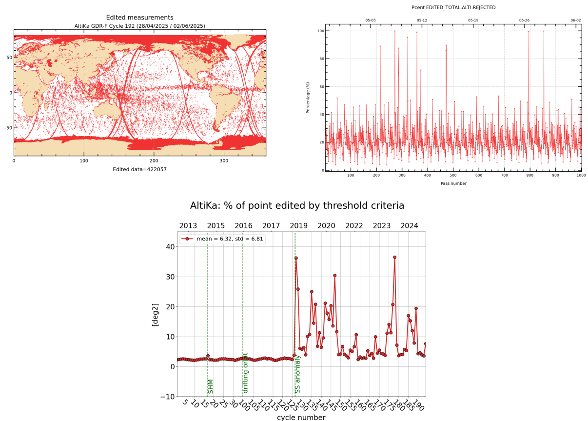
Figure 2: Rejected measurements on thresholds criteria : Cycle 192, map and monitoring of % of rejected measurements per track (top), whole time serie / % of rejected measurements per cycle (bottom).
