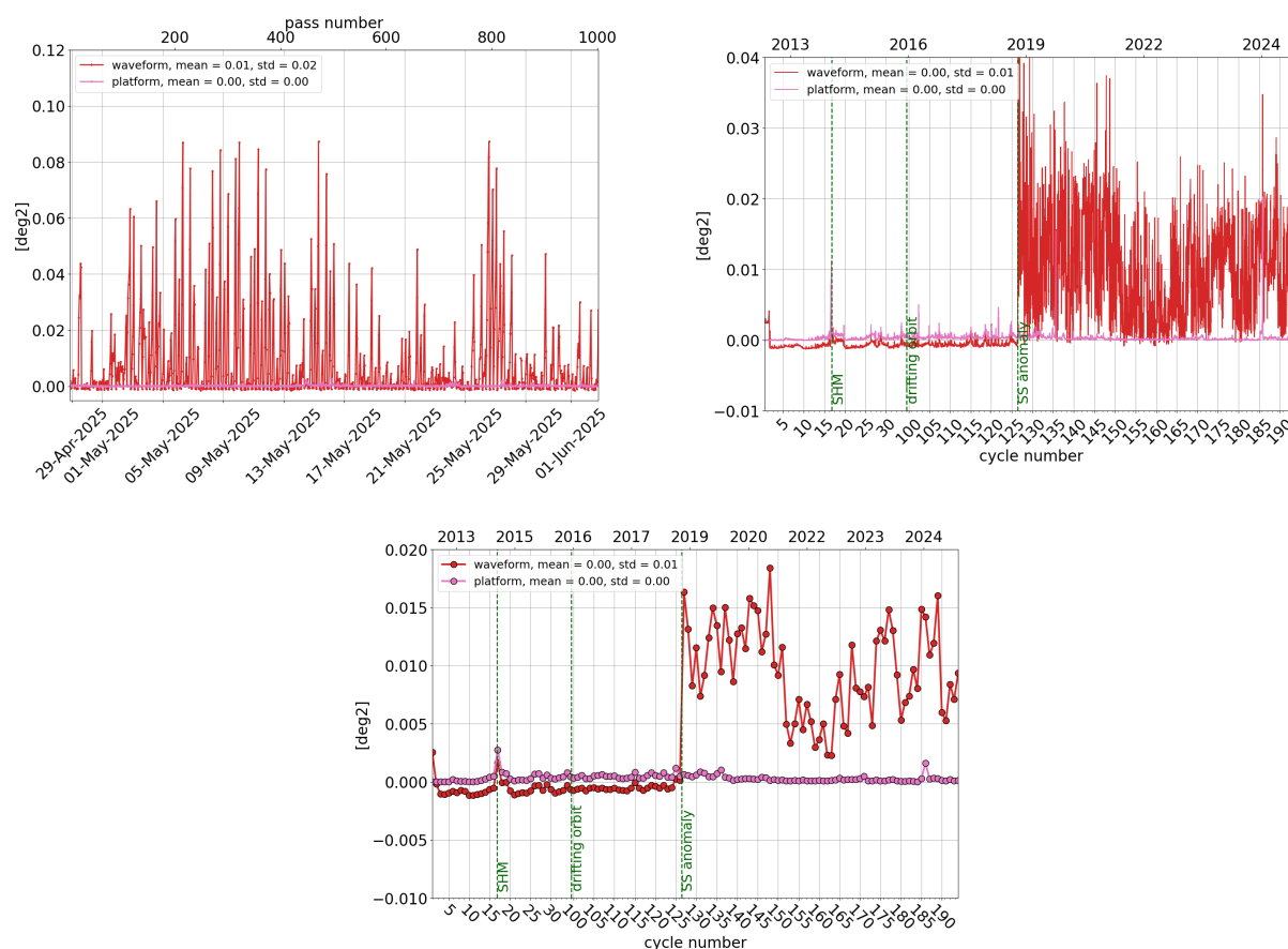
Figure 13: Monitoring per pass for cycle 192 (left), daily monitoring(right) and cyclic monitoring (bottom) of SARAL/AltiKa's mispointing angle: comparison between the one derived from waveform retracking and the one measured by platform startrackers.
