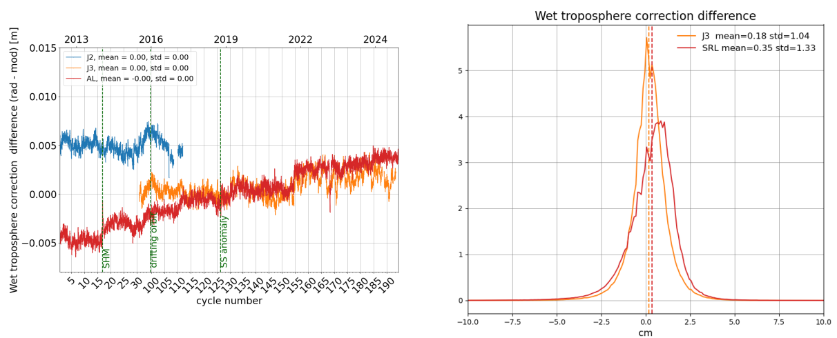
Figure 12: Daily monitoring of wet troposphere differences (Radiometer-ECMWF model) for Saral/AltiKa Jason-2 and Jason-3 (left) and histogram on the right (limited to 66° latitude) for cycle 192 .
