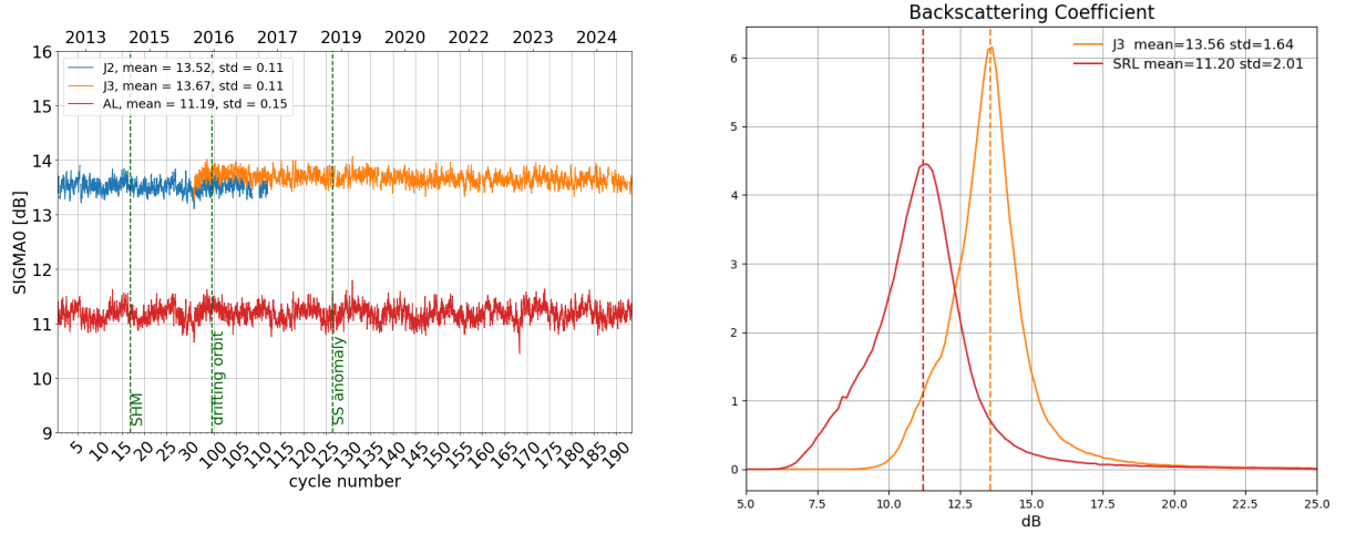
Figure 7: Daily monitoring of backscattering coefficient for Saral/AltiKa, Jason-2 and Jason-3 on the left and histogram for cycle 193 on the right (limited to 66° latitude).
