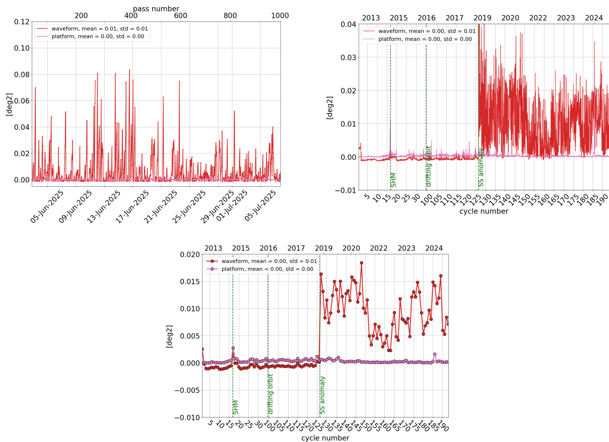
Figure 13: Monitoring per pass for cycle 193 (left), daily monitoring(right) and cyclic monitoring (bottom) of SARAL/AltiKa's mispointing angle: comparison between the one derived from waveform retracking and the one measured by platform startrackers.
