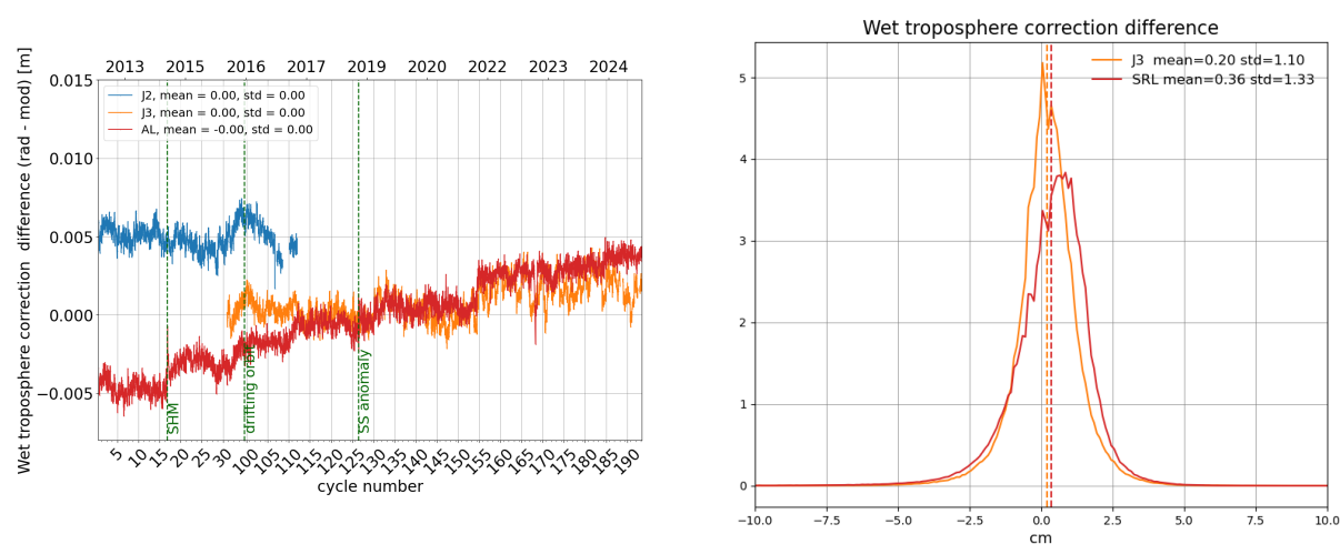
Figure 12: Daily monitoring of wet troposphere differences (Radiometer-ECMWF model) for Saral/AltiKa Jason-2 and Jason-3 (left) and histogram on the right (limited to 66° latitude) for cycle 193 .
