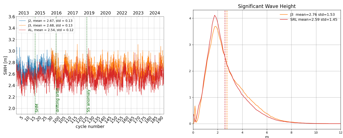
Figure 6: Daily monitoring of significant wave height for AltiKa (Ka-band) Jason-2 and Jason-3 (Ku-band) on the left and histogram for cycle 193 on the right (limited to 66^\circ latitude).
