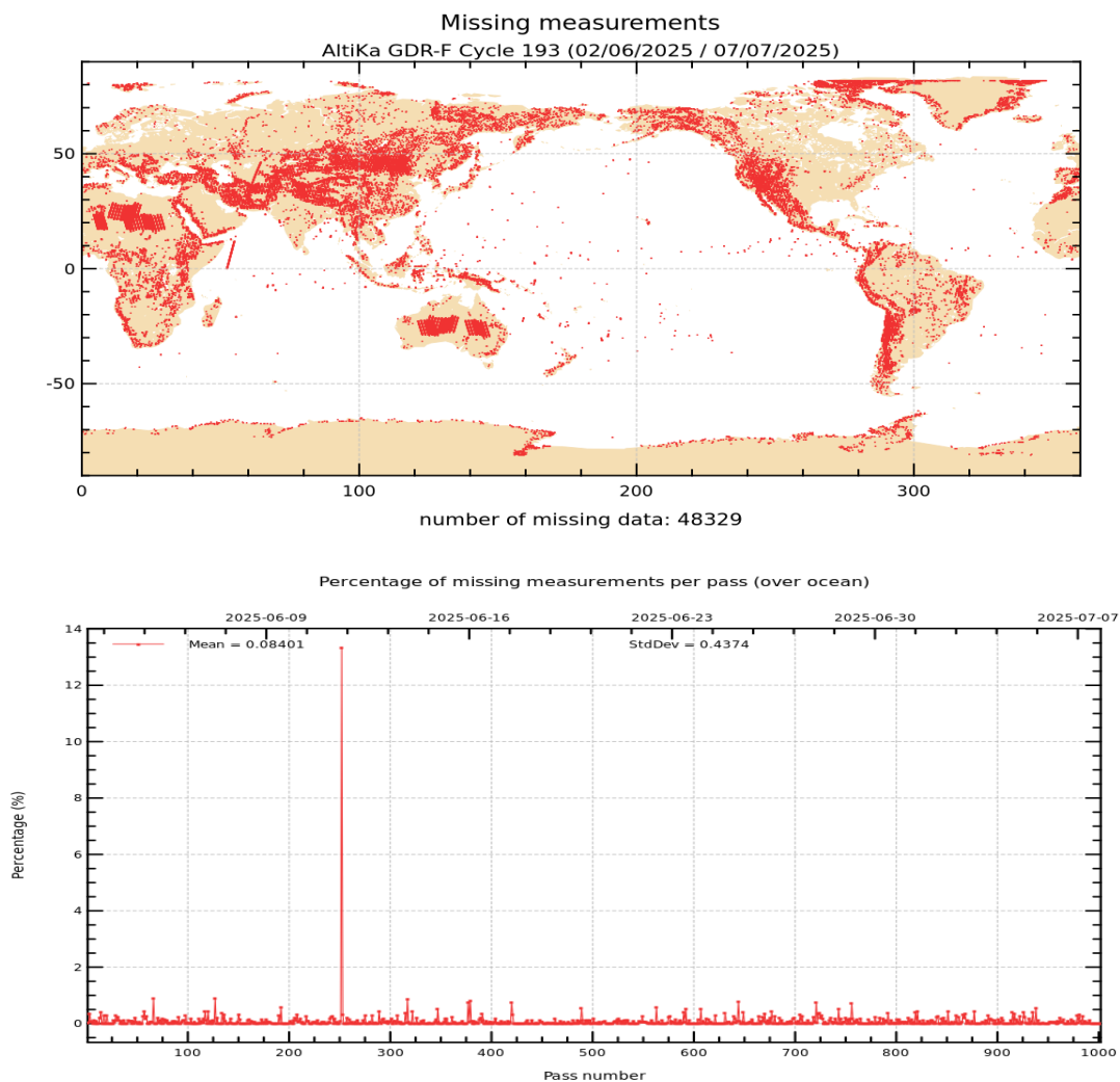
Figure 1: Map of missing measurements for cycle 193 on top. Monitoring of percentage of missing ocean measurements per pass on bottom.
