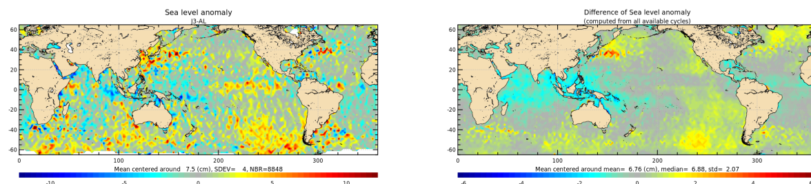
Figure 21: Jason-3 — Saral/AltiKa SLA differences for cycle 193 (left) and averaged over the whole Saral/AltiKa period (right).
