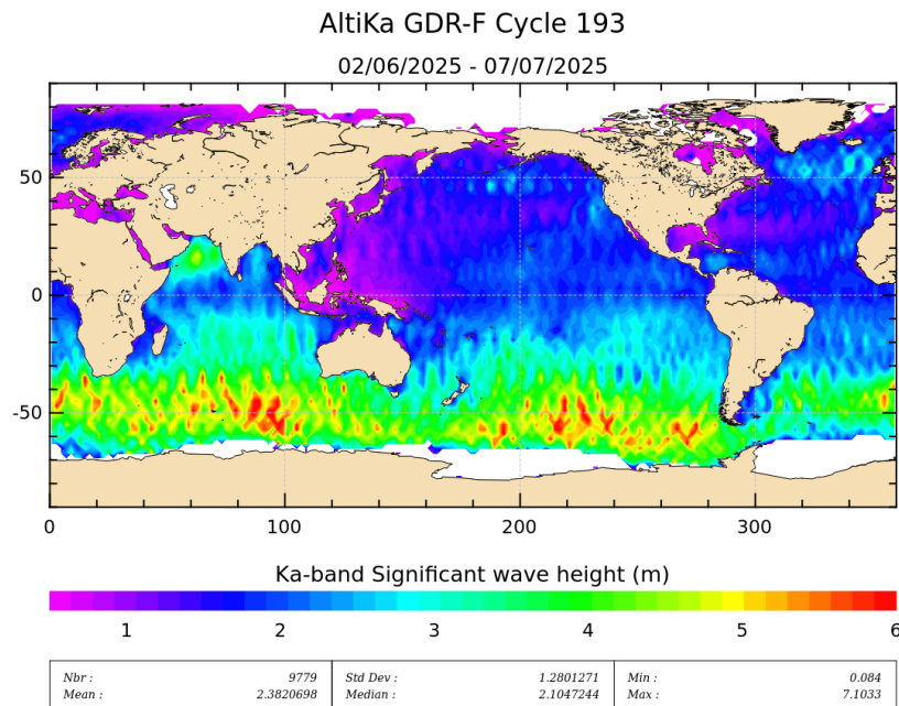
Figure 5: Significant wave height for cycle 193.
