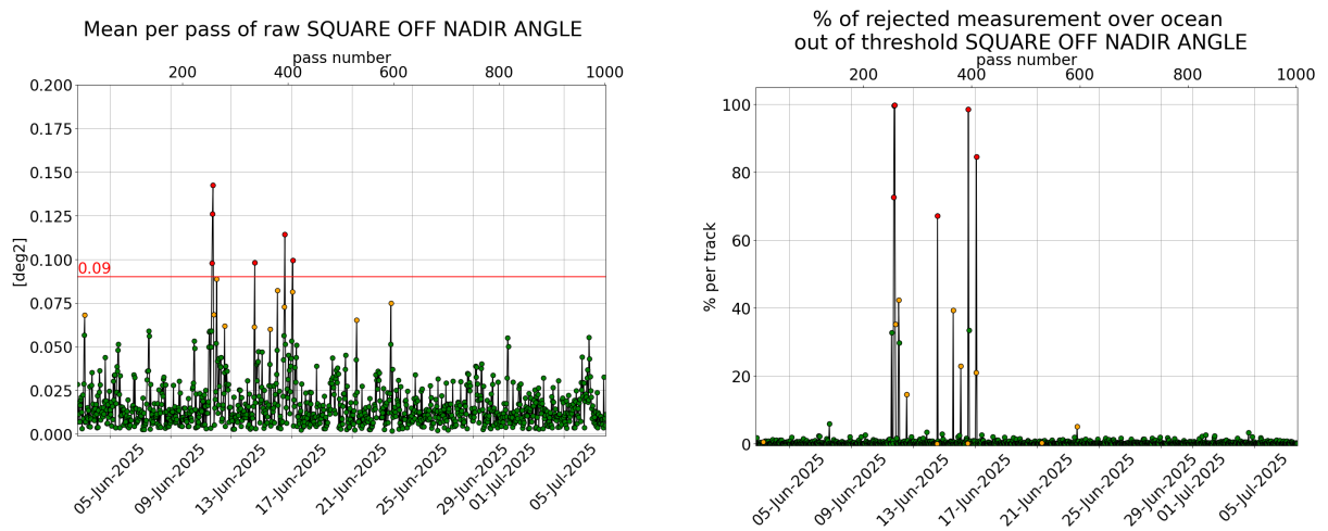
Figure 3: [left] Mispointing cycle 193, [right] Percentage of rejected measurement by threshold on square off-nadir angle.
