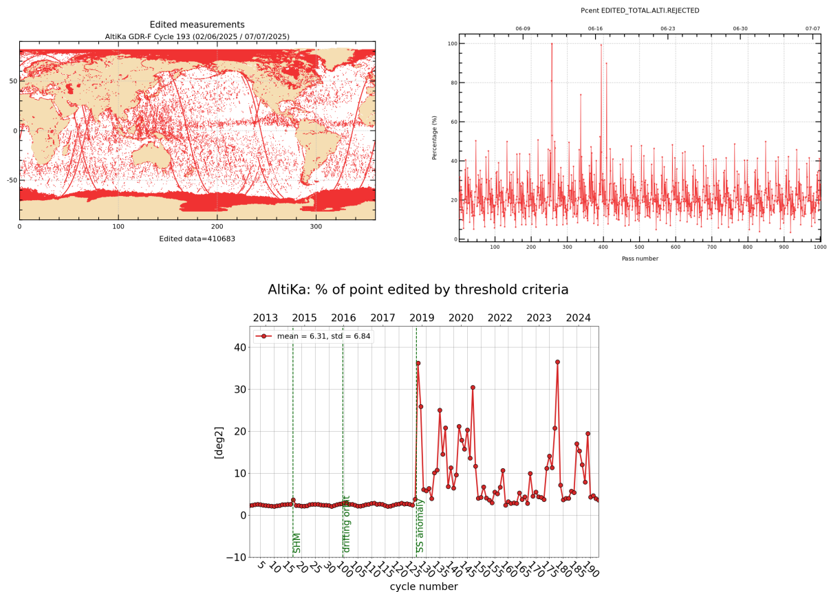
Figure 2: Rejected measurements on thresholds criteria : Cycle 193, map and monitoring of % of rejected measurements per track (top), whole time serie / % of rejected measurements per cycle (bottom).
