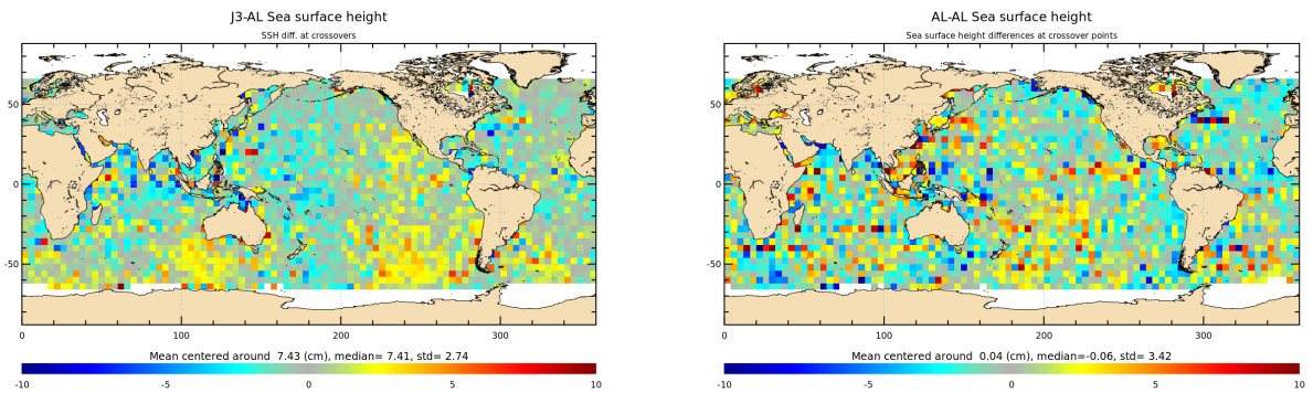
Figure 14: Mean of multi-mission SSH and mono-mission SSH differences at crossovers for cycle 193.
