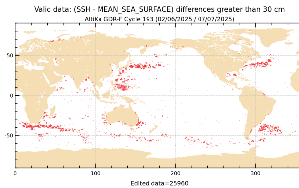
Figure 20: SLA higher than 30 cm for cycle 193.
