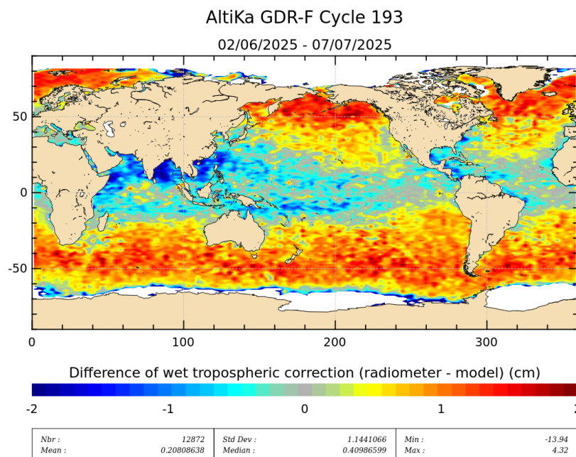
Figure 11: Mean of wet troposphere correction difference (Radiometer-ECMWF model)for cycle 193.
