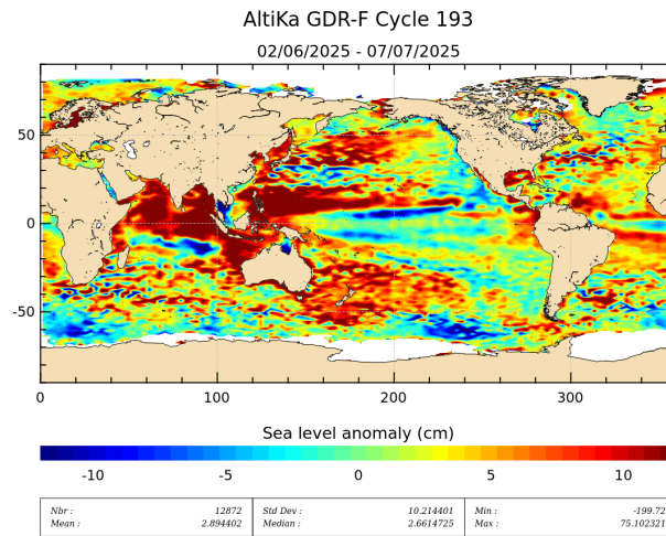
Figure 19: Sea level anomaly relative to MSS for cycle 193.
