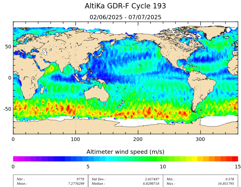
Figure 9: Altimeter wind speed for cycle 193.
