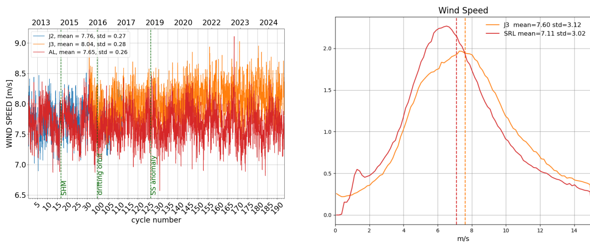
Figure 10: Daily monitoring of altimeter wind speed for Saral/AltiKa, Jason-2 and Jason-3 on the left and histogram for cycle 193 on the right (limited to 66° latitude).
