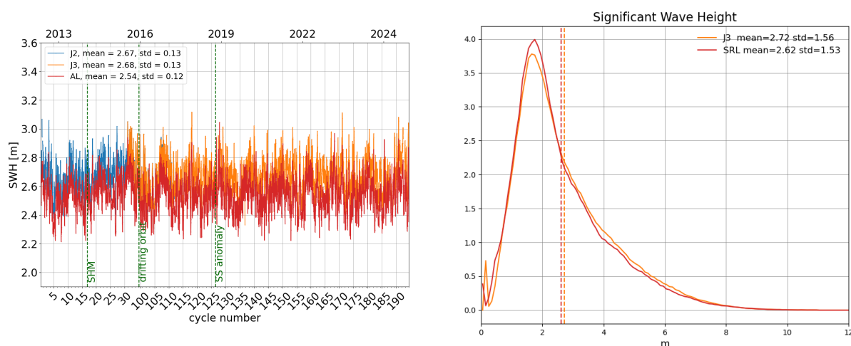
Figure 6: Daily monitoring of significant wave height for AltiKa (Ka-band) Jason-2 and Jason-3 (Ku-band) on the left and histogram for cycle 194 on the right (limited to 66^\circ latitude).
