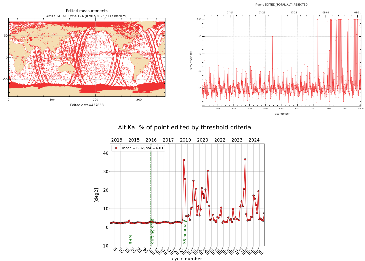
Figure 2: Rejected measurements on thresholds criteria : Cycle 194, map and monitoring of % of rejected measurements per track (top), whole time serie / % of rejected measurements per cycle (bottom).
