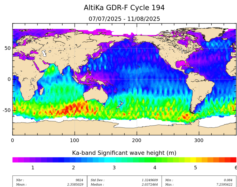
Figure 5: Significant wave height for cycle 194.
