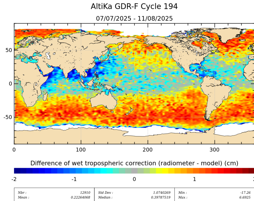
Figure 11: Mean of wet troposphere correction difference (Radiometer-ECMWF model)for cycle 194.
