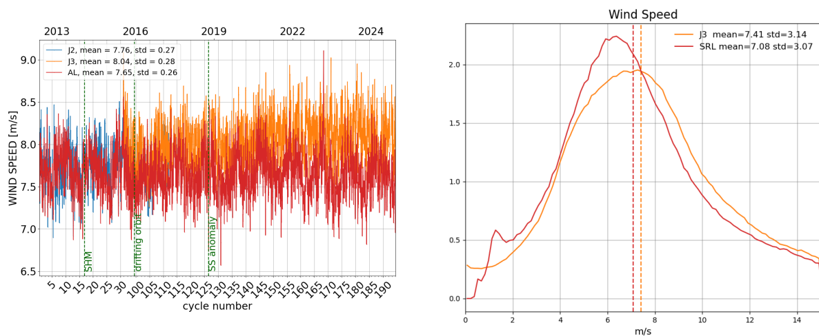
Figure 10: Daily monitoring of altimeter wind speed for Saral/AltiKa, Jason-2 and Jason-3 on the left and histogram for cycle 194 on the right (limited to 66° latitude).
