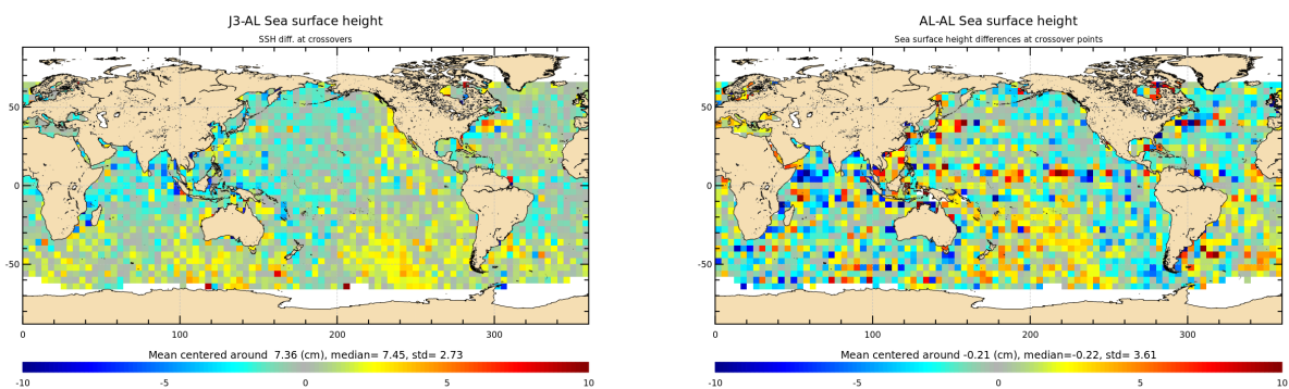
Figure 14: Mean of multi-mission SSH and mono-mission SSH differences at crossovers for cycle 194.
