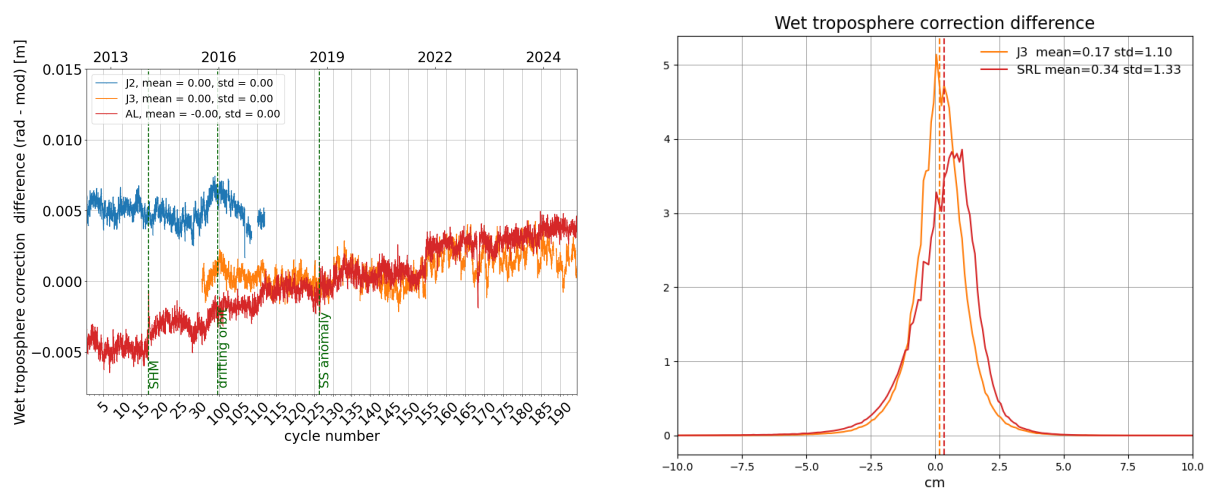
Figure 12: Daily monitoring of wet troposphere differences (Radiometer-ECMWF model) for Saral/AltiKa Jason-2 and Jason-3 (left) and histogram on the right (limited to 66° latitude) for cycle 194 .
