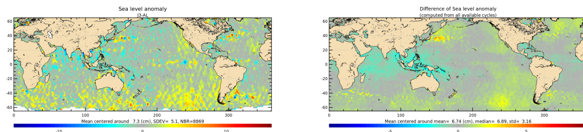
Figure 21: Jason-3 — Saral/AltiKa SLA differences for cycle 194 (left) and averaged over the whole Saral/AltiKa period (right).
