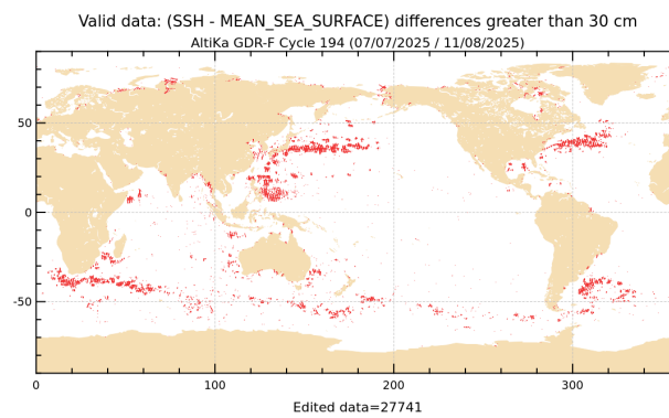
Figure 20: SLA higher than 30 cm for cycle 194.
