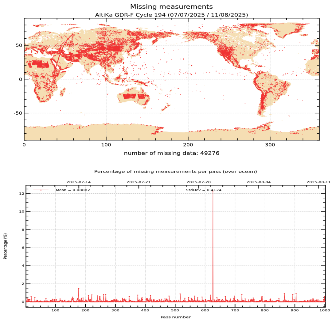
Figure 1: Map of missing measurements for cycle 194 on top. Monitoring of percentage of missing ocean measurements per pass on bottom.
