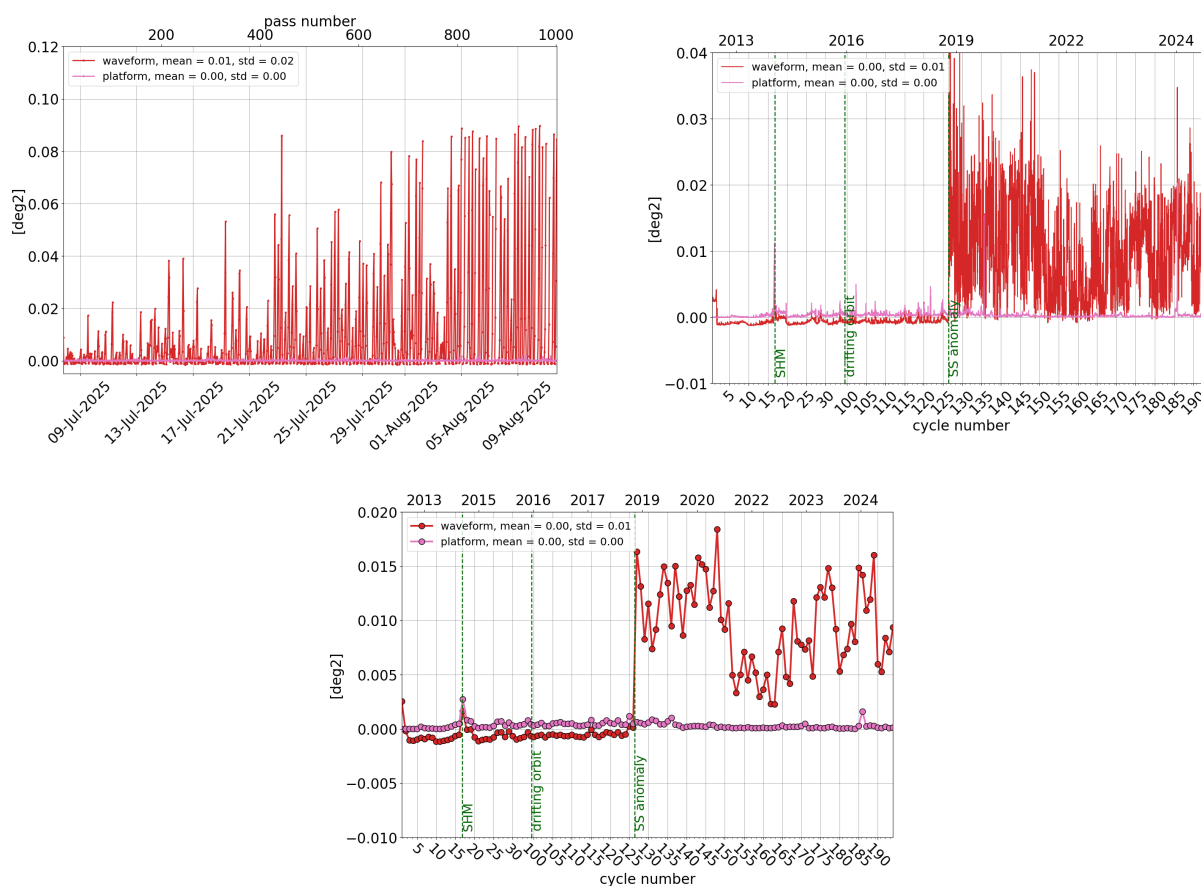
Figure 13: Monitoring per pass for cycle 194 (left), daily monitoring(right) and cyclic monitoring (bottom) of SARAL/AltiKa's mispointing angle: comparison between the one derived from waveform retracking and the one measured by platform startrackers.
