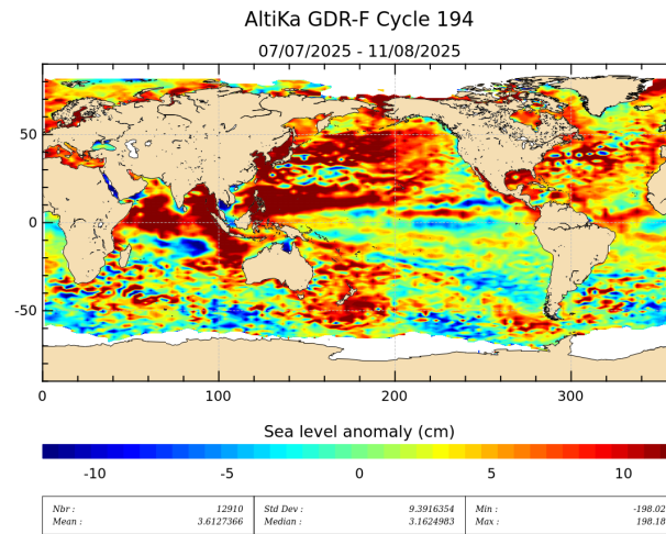
Figure 19: Sea level anomaly relative to MSS for cycle 194.
