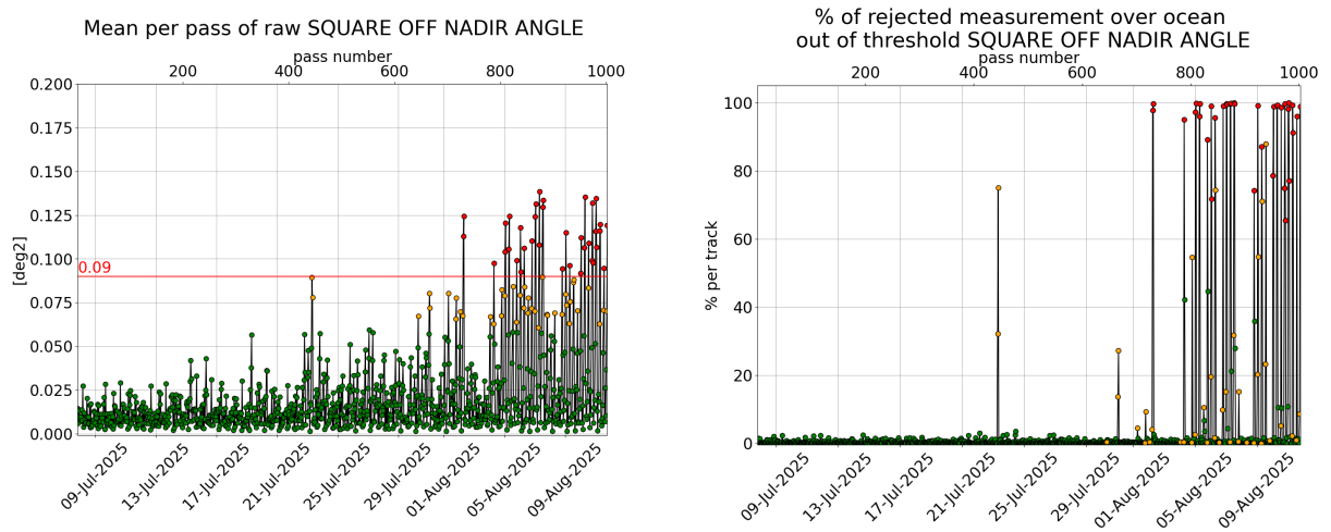
Figure 3: [left] Mispointing cycle 194, [right] Percentage of rejected measurement by threshold on square off-nadir angle.
