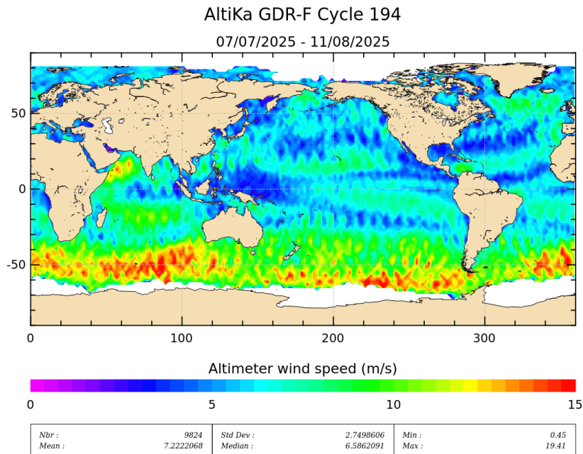
Figure 9: Altimeter wind speed for cycle 194.
