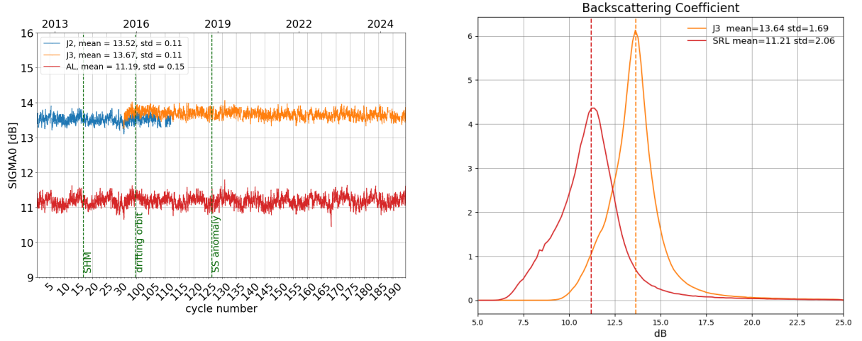
Figure 7: Daily monitoring of backscattering coefficient for Saral/AltiKa, Jason-2 and Jason-3 on the left and histogram for cycle 194 on the right (limited to 66° latitude).
