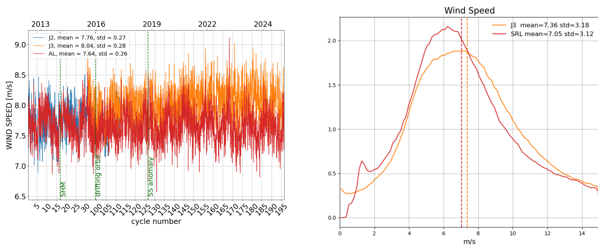
Figure 10: Daily monitoring of altimeter wind speed for Saral/AltiKa, Jason-2 and Jason-3 on the left and histogram for cycle 195 on the right (limited to 66° latitude).
