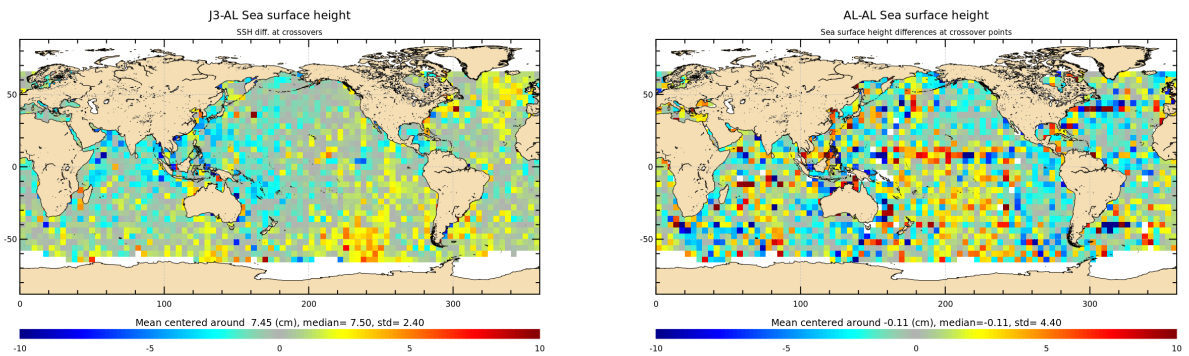
Figure 14: Mean of multi-mission SSH and mono-mission SSH differences at crossovers for cycle 195.
