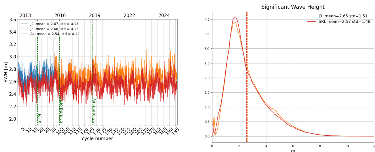
Figure 6: Daily monitoring of significant wave height for AltiKa (Ka-band) Jason-2 and Jason-3 (Ku-band) on the left and histogram for cycle 195 on the right (limited to 66^\circ latitude).
