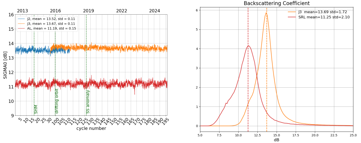
Figure 7: Daily monitoring of backscattering coefficient for Saral/AltiKa, Jason-2 and Jason-3 on the left and histogram for cycle 195 on the right (limited to 66° latitude).
