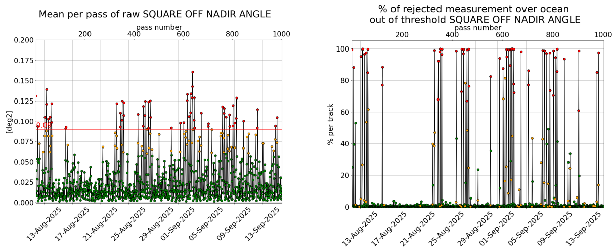
Figure 3: [left] Mispointing cycle 195, [right] Percentage of rejected measurement by threshold on square off-nadir angle.
