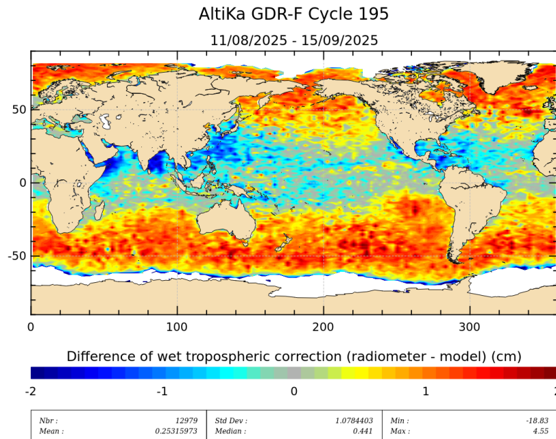
Figure 11: Mean of wet troposphere correction difference (Radiometer-ECMWF model)for cycle 195.
