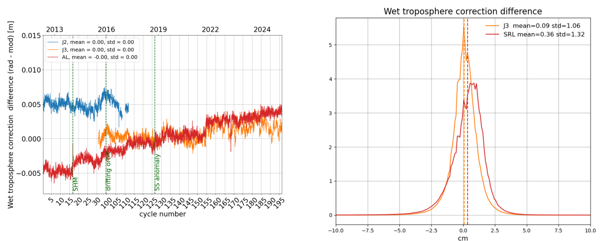
Figure 12: Daily monitoring of wet troposphere differences (Radiometer-ECMWF model) for Saral/AltiKa Jason-2 and Jason-3 (left) and histogram on the right (limited to 66° latitude) for cycle 195 .
