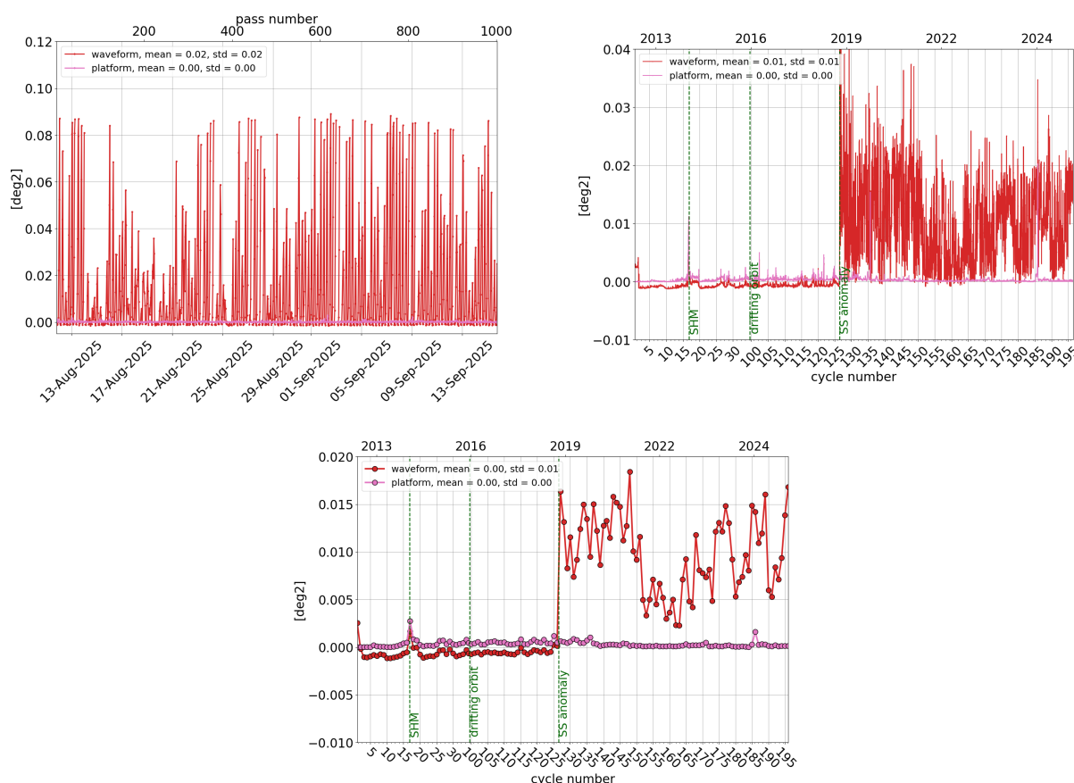
Figure 13: Monitoring per pass for cycle 195 (left), daily monitoring(right) and cyclic monitoring (bottom) of SARAL/AltiKa's mispointing angle: comparison between the one derived from waveform retracking and the one measured by platform startrackers.
