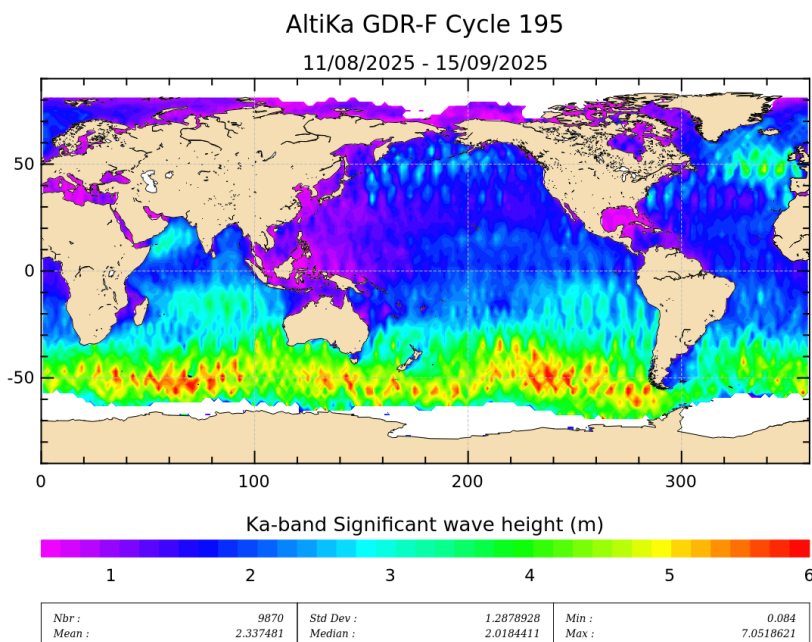
Figure 5: Significant wave height for cycle 195.
