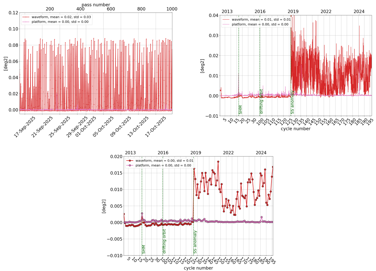
Figure 13: Monitoring per pass for cycle 196 (left), daily monitoring(right) and cyclic monitoring (bottom) of SARAL/AltiKa's mispointing angle: comparison between the one derived from waveform retracking and the one measured by platform startrackers.
