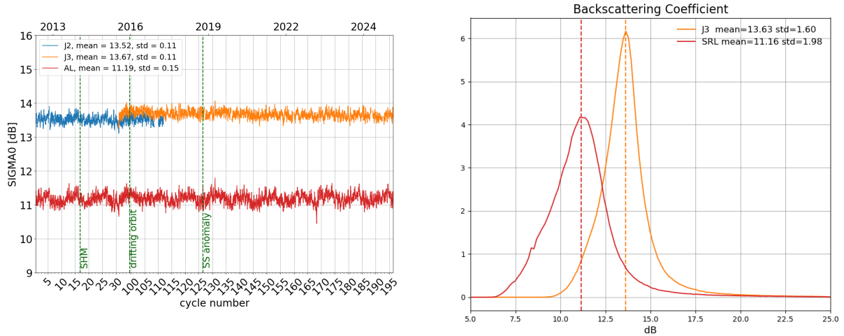
Figure 7: Daily monitoring of backscattering coefficient for Saral/AltiKa, Jason-2 and Jason-3 on the left and histogram for cycle 196 on the right (limited to 66° latitude).
