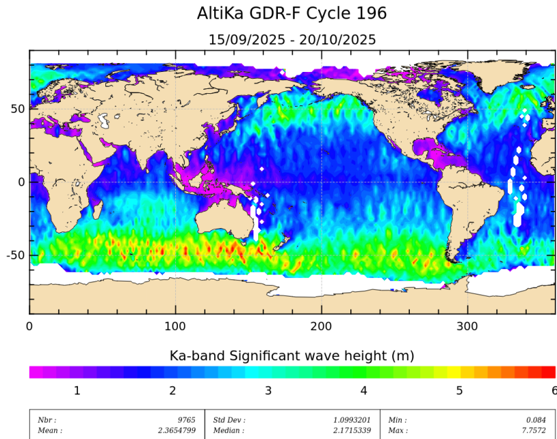
Figure 5: Significant wave height for cycle 196.
