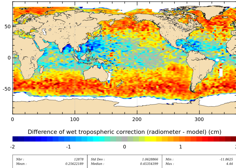
Figure 11: Mean of wet troposphere correction difference (Radiometer-ECMWF model) for cycle 196.
