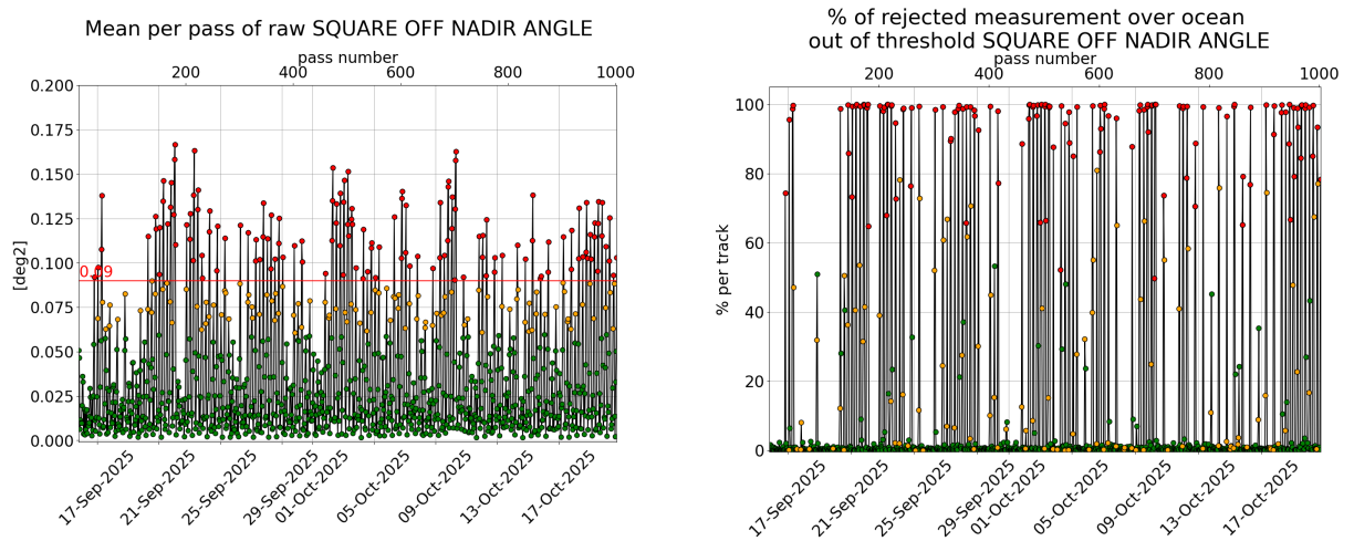
Figure 3: [left] Mispointing cycle 196, [right] Percentage of rejected measurement by threshold on square off-nadir angle.
