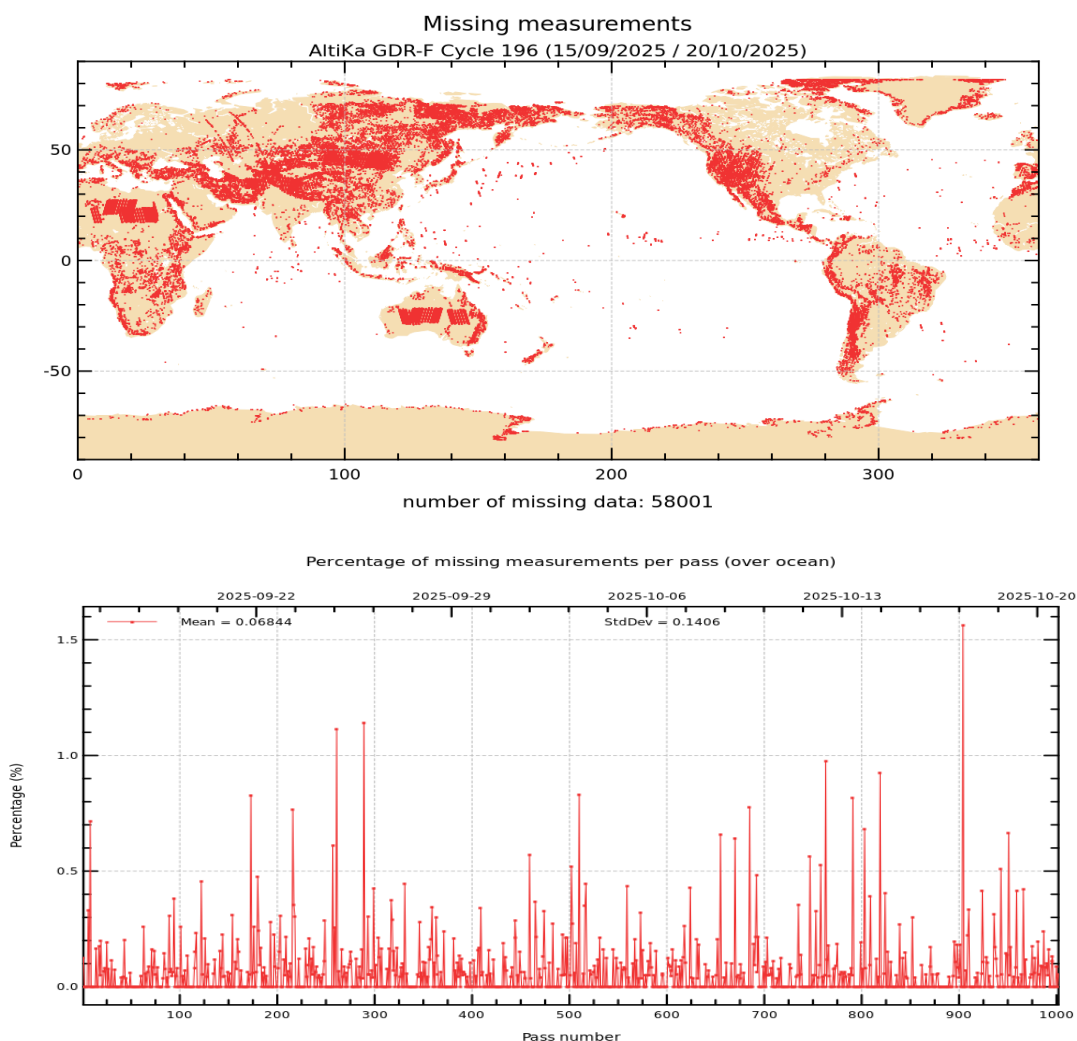
Figure 1: Map of missing measurements for cycle 196 on top. Monitoring of percentage of missing ocean measurements per pass on bottom.
