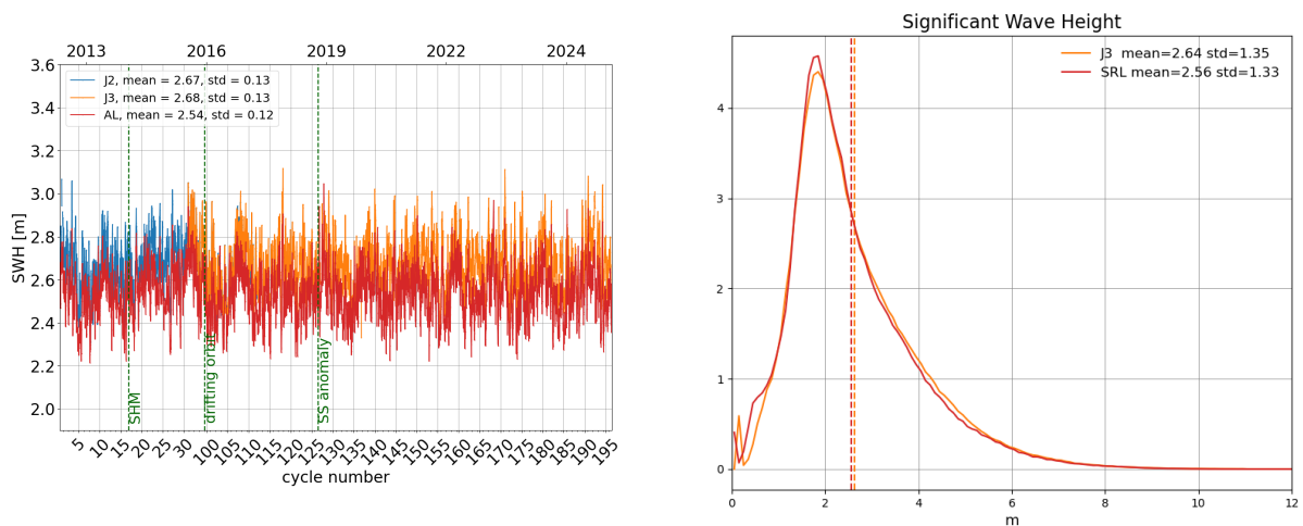
Figure 6: Daily monitoring of significant wave height for AltiKa (Ka-band) Jason-2 and Jason-3 (Ku-band) on the left and histogram for cycle 196 on the right (limited to 66^\circ latitude).
