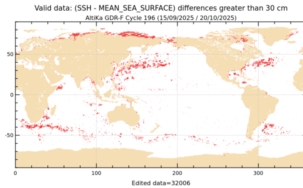
Figure 20: SLA higher than 30 cm for cycle 196.
