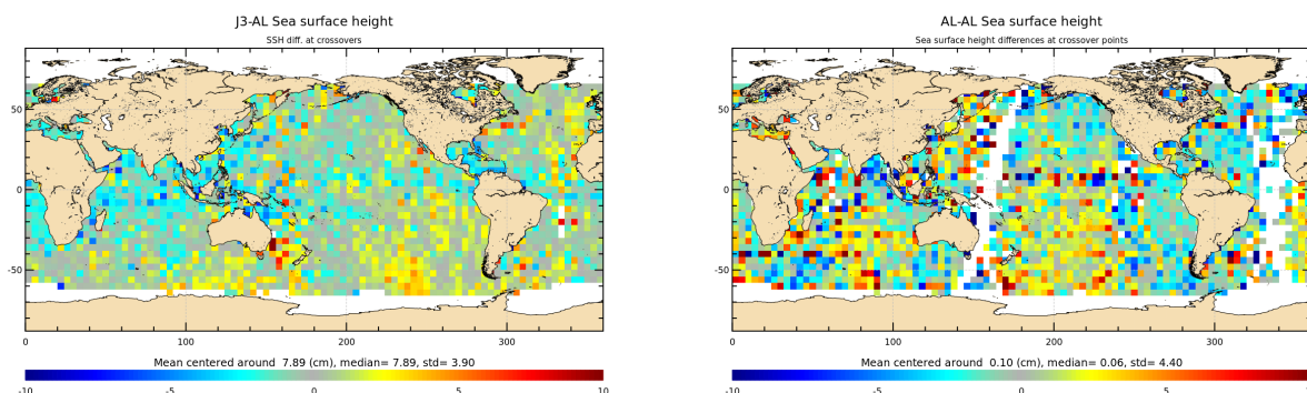
Figure 14: Mean of multi-mission SSH and mono-mission SSH differences at crossovers for cycle 196.
