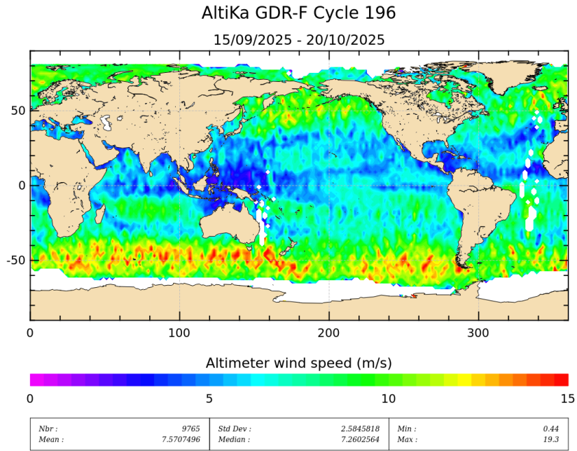
Figure 9: Altimeter wind speed for cycle 196.
