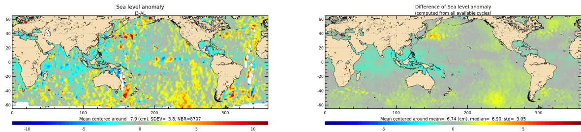
Figure 21: Jason-3 – Saral/AltiKa SLA differences for cycle 196 (left) and averaged over the whole Saral/AltiKa period (right).
