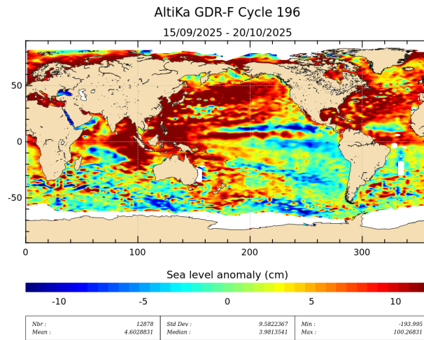
Figure 19: Sea level anomaly relative to MSS for cycle 196.
