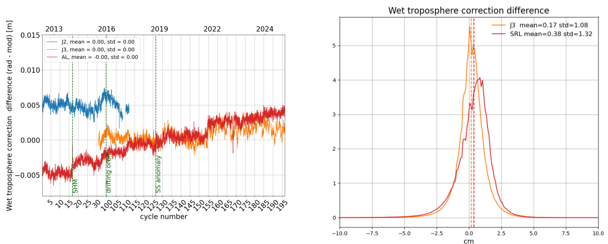
Figure 12: Daily monitoring of wet troposphere differences (Radiometer-ECMWF model) for Saral/AltiKa Jason-2 and Jason-3 (left) and histogram on the right (limited to 66° latitude) for cycle 196 .
