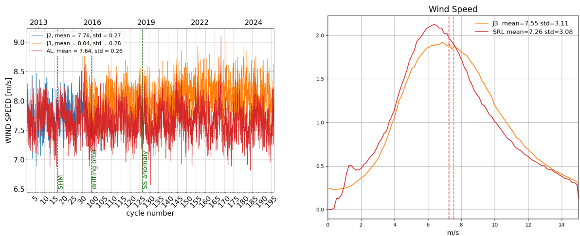
Figure 10: Daily monitoring of altimeter wind speed for Saral/AltiKa, Jason-2 and Jason-3 on the left and histogram for cycle 196 on the right (limited to 66° latitude).
