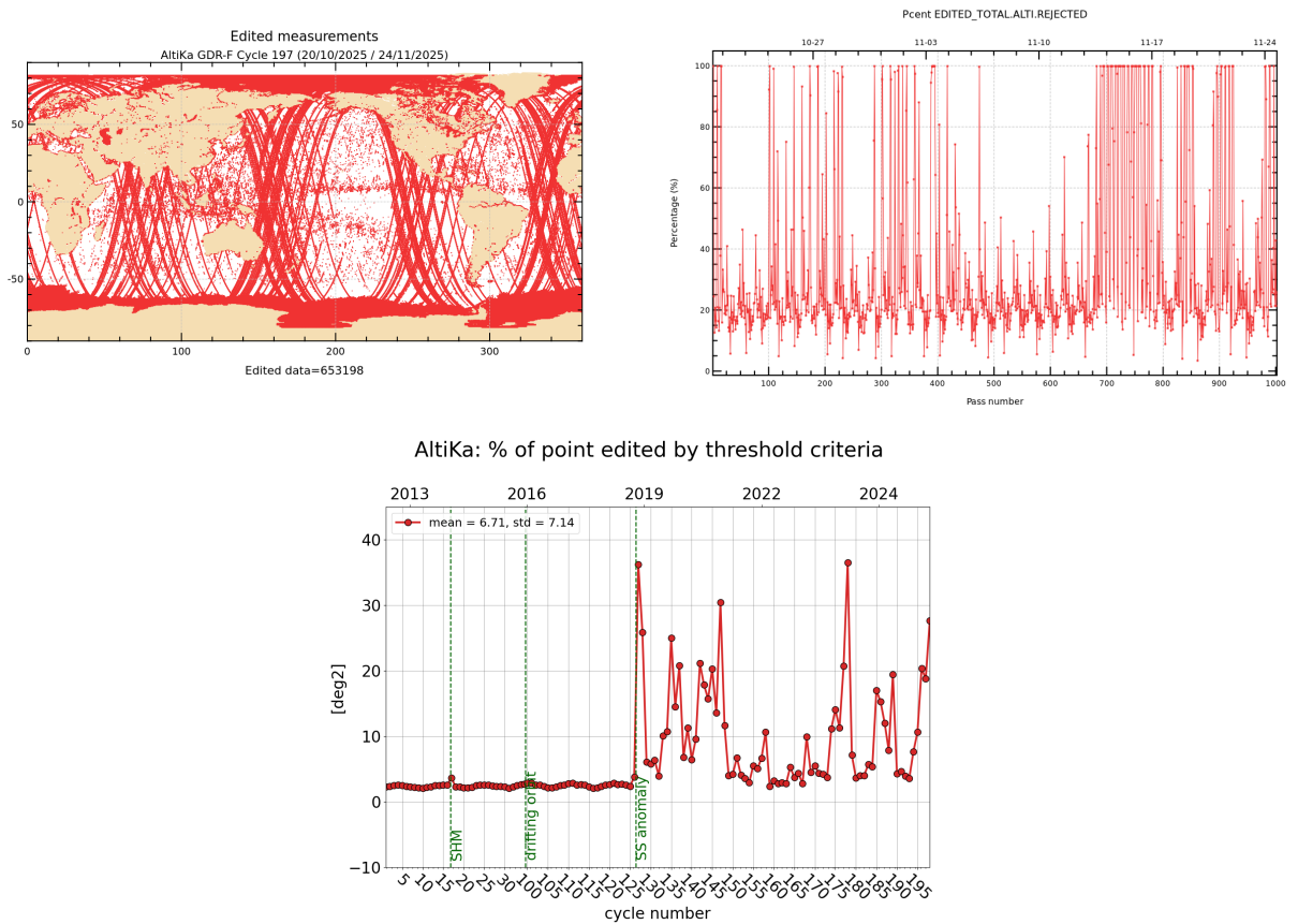
Figure 2: Rejected measurements on thresholds criteria : Cycle 197, map and monitoring of % of rejected measurements per track (top), whole time serie / % of rejected measurements per cycle (bottom).
