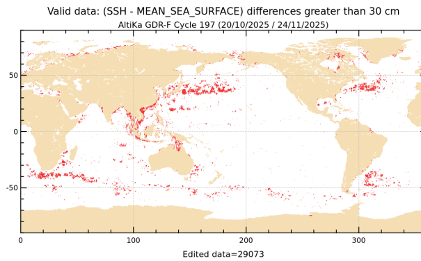
Figure 20: SLA higher than 30 cm for cycle 197.
