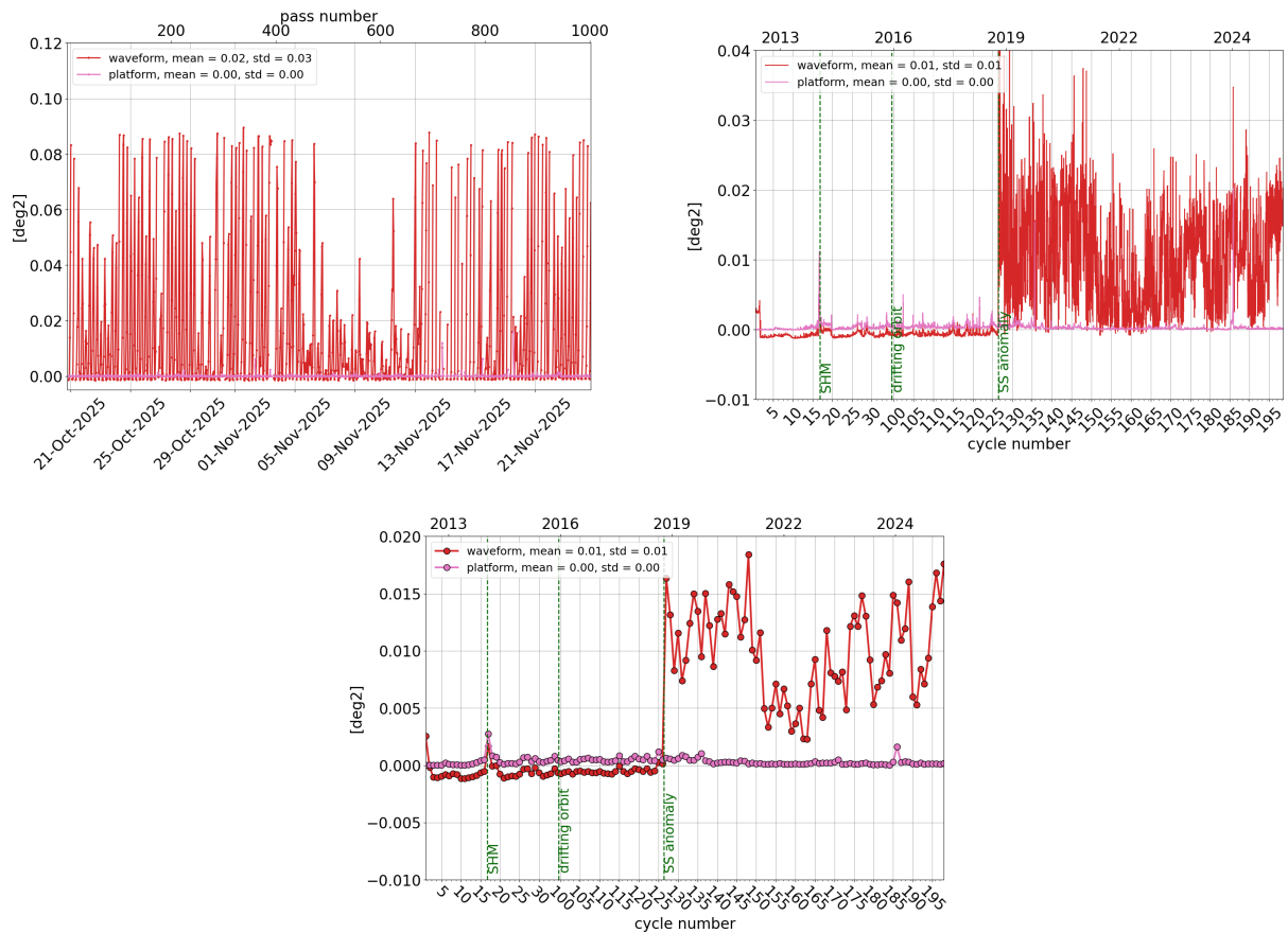
Figure 13: Monitoring per pass for cycle 197 (left), daily monitoring(right) and cyclic monitoring (bottom) of SARAL/AltiKa's mispointing angle: comparison between the one derived from waveform retracking and the one measured by platform startrackers.
