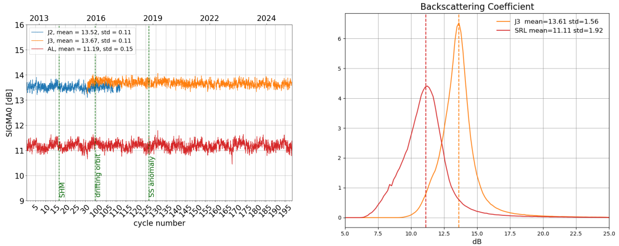
Figure 7: Daily monitoring of backscattering coefficient for Saral/AltiKa, Jason-2 and Jason-3 on the left and histogram for cycle 197 on the right (limited to 66° latitude).
