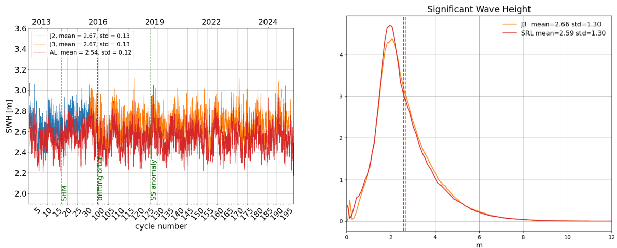
Figure 6: Daily monitoring of significant wave height for AltiKa (Ka-band) Jason-2 and Jason-3 (Ku-band) on the left and histogram for cycle 197 on the right (limited to 66^\circ latitude).
