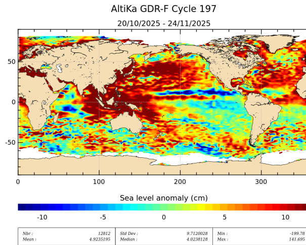
Figure 19: Sea level anomaly relative to MSS for cycle 197.
