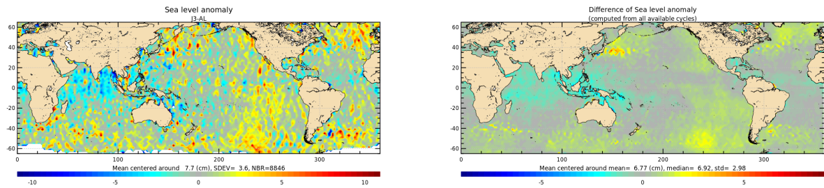
Figure 21: Jason-3 – Saral/AltiKa SLA differences for cycle 197 (left) and averaged over the whole Saral/AltiKa period (right).
