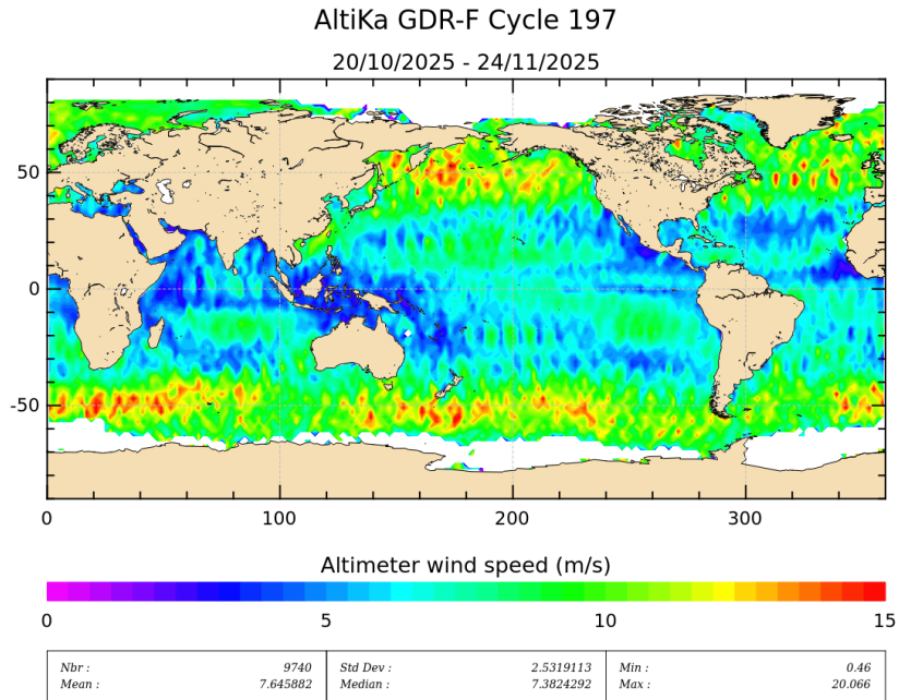
Figure 9: Altimeter wind speed for cycle 197.
