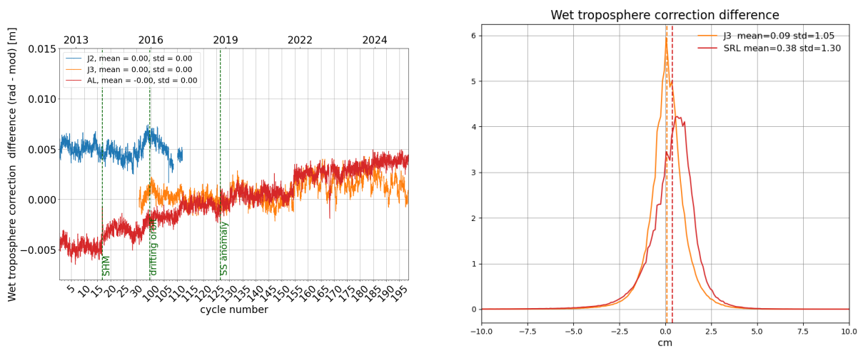
Figure 12: Daily monitoring of wet troposphere differences (Radiometer-ECMWF model) for Saral/AltiKa Jason-2 and Jason-3 (left) and histogram on the right (limited to 66° latitude) for cycle 197 .
