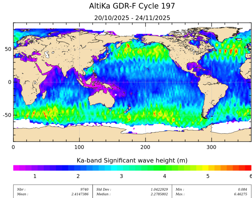
Figure 5: Significant wave height for cycle 197.
