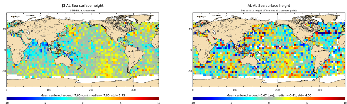
Figure 14: Mean of multi-mission SSH and mono-mission SSH differences at crossovers for cycle 197.
