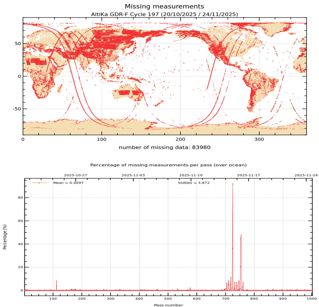
Figure 1: Map of missing measurements for cycle 197 on top. Monitoring of percentage of missing ocean measurements per pass on bottom.
