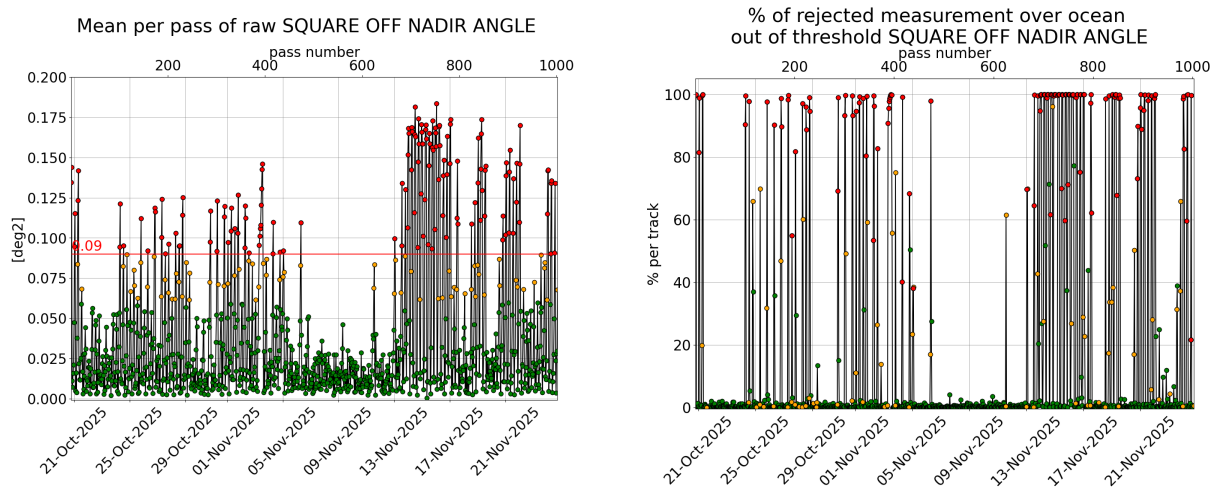
Figure 3: [left] Mispointing cycle 197, [right] Percentage of rejected measurement by threshold on square off-nadir angle.
