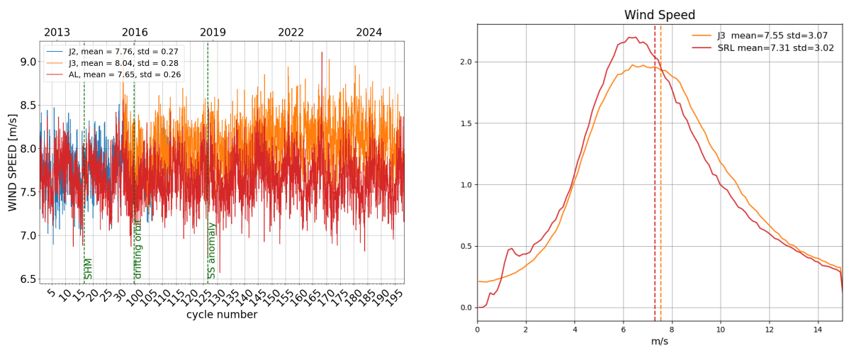
Figure 10: Daily monitoring of altimeter wind speed for Saral/AltiKa, Jason-2 and Jason-3 on the left and histogram for cycle 197 on the right (limited to 66° latitude).
