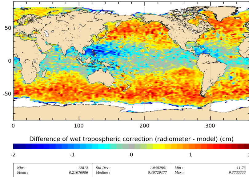
Figure 11: Mean of wet troposphere correction difference (Radiometer-ECMWF model) for cycle 197.
