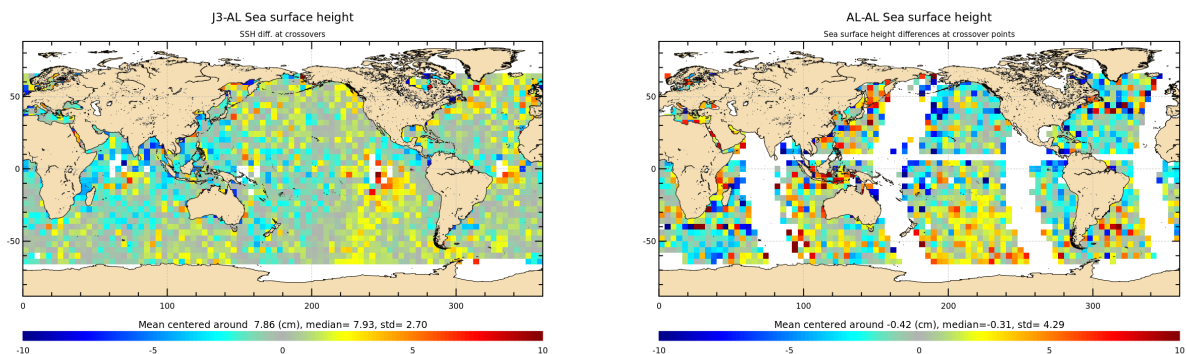
Figure 14: Mean of multi-mission SSH and mono-mission SSH differences at crossovers for cycle 198.
