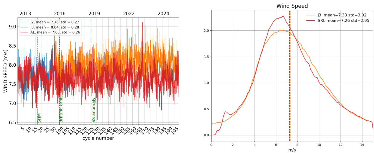
Figure 10: Daily monitoring of altimeter wind speed for Saral/AltiKa, Jason-2 and Jason-3 on the left and histogram for cycle 198 on the right (limited to 66° latitude).
