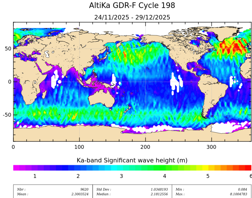
Figure 5: Significant wave height for cycle 198.
