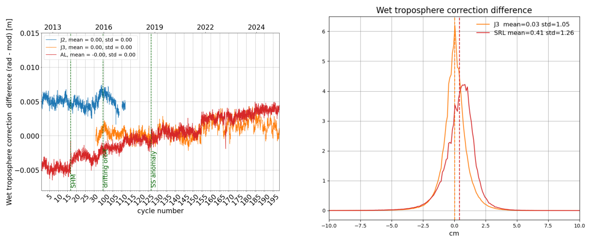
Figure 12: Daily monitoring of wet troposphere differences (Radiometer-ECMWF model) for Saral/AltiKa Jason-2 and Jason-3 (left) and histogram on the right (limited to 66° latitude) for cycle 198 .
