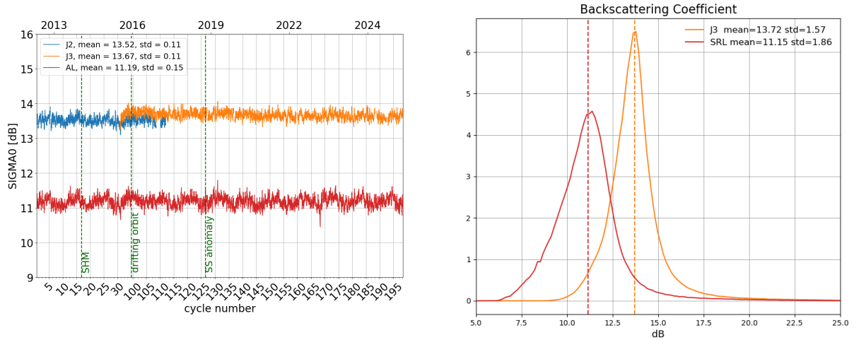
Figure 7: Daily monitoring of backscattering coefficient for Saral/AltiKa, Jason-2 and Jason-3 on the left and histogram for cycle 198 on the right (limited to 66° latitude).
