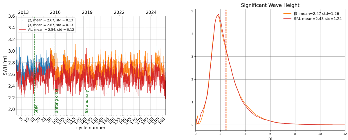
Figure 6: Daily monitoring of significant wave height for AltiKa (Ka-band) Jason-2 and Jason-3 (Ku-band) on the left and histogram for cycle 198 on the right (limited to 66^\circ latitude).
