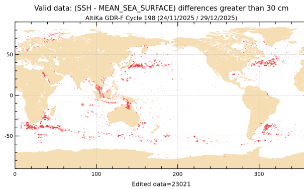
Figure 20: SLA higher than 30 cm for cycle 198.
