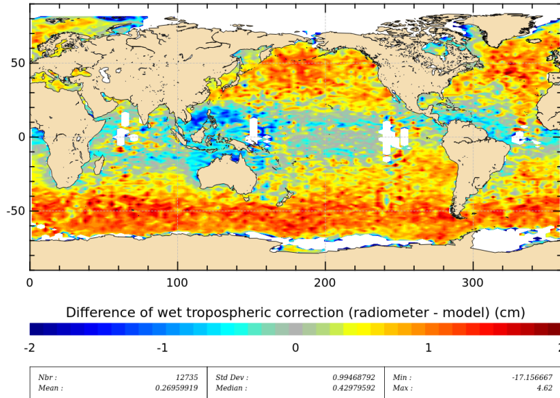
Figure 11: Mean of wet troposphere correction difference (Radiometer-ECMWF model) for cycle 198.
