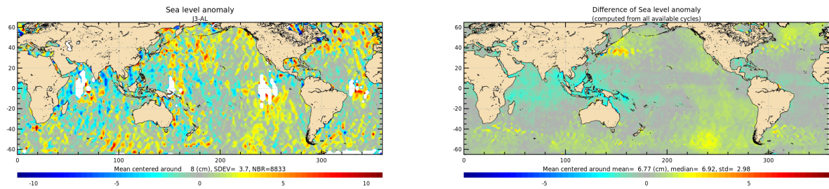
Figure 21: Jason-3 – Saral/AltiKa SLA differences for cycle 198 (left) and averaged over the whole Saral/AltiKa period (right).
