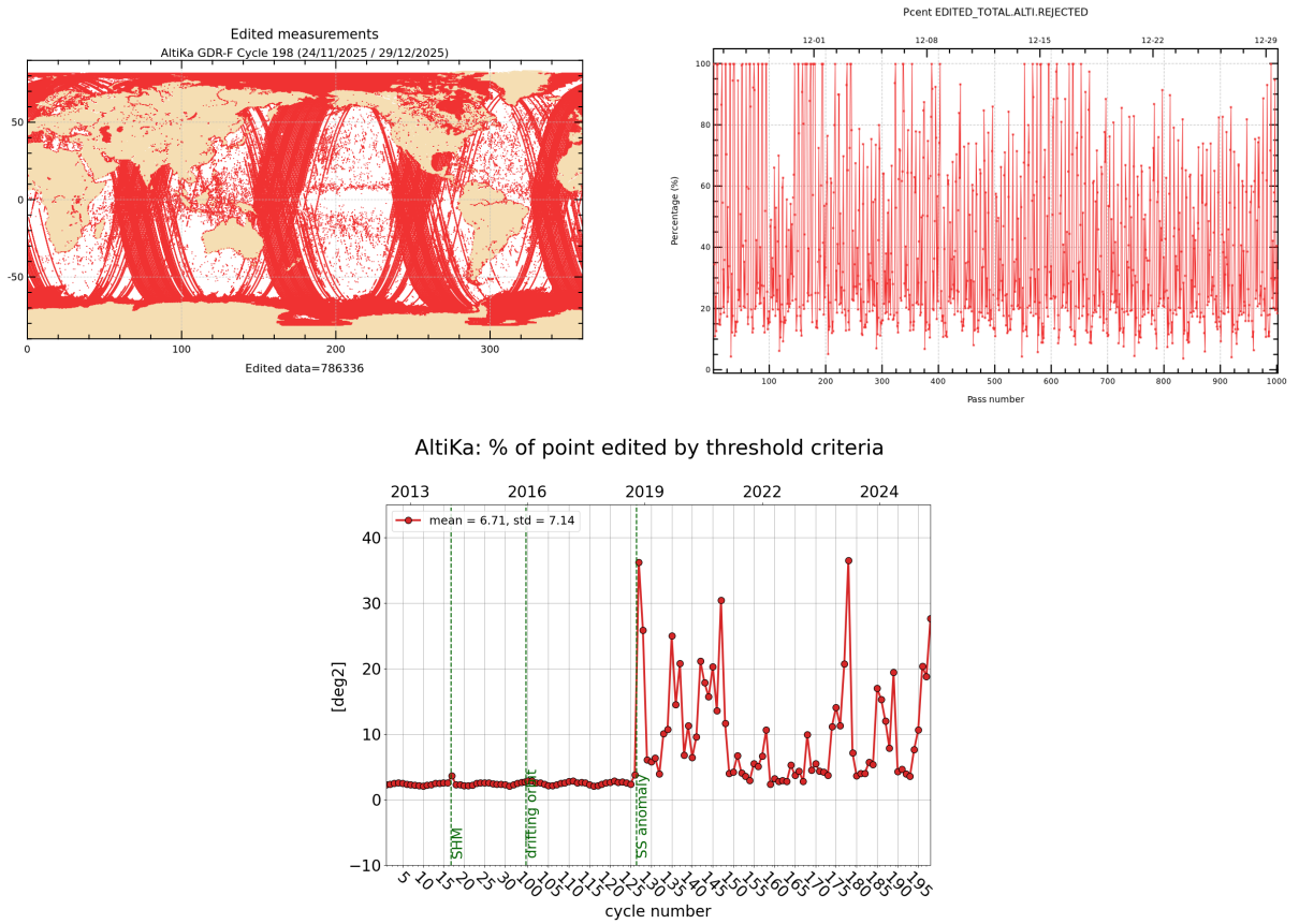
Figure 2: Rejected measurements on thresholds criteria : Cycle 198, map and monitoring of % of rejected measurements per track (top), whole time serie / % of rejected measurements per cycle (bottom).
