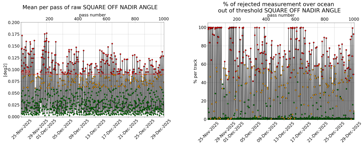
Figure 3: [left] Mispointing cycle 198, [right] Percentage of rejected measurement by threshold on square off-nadir angle.
