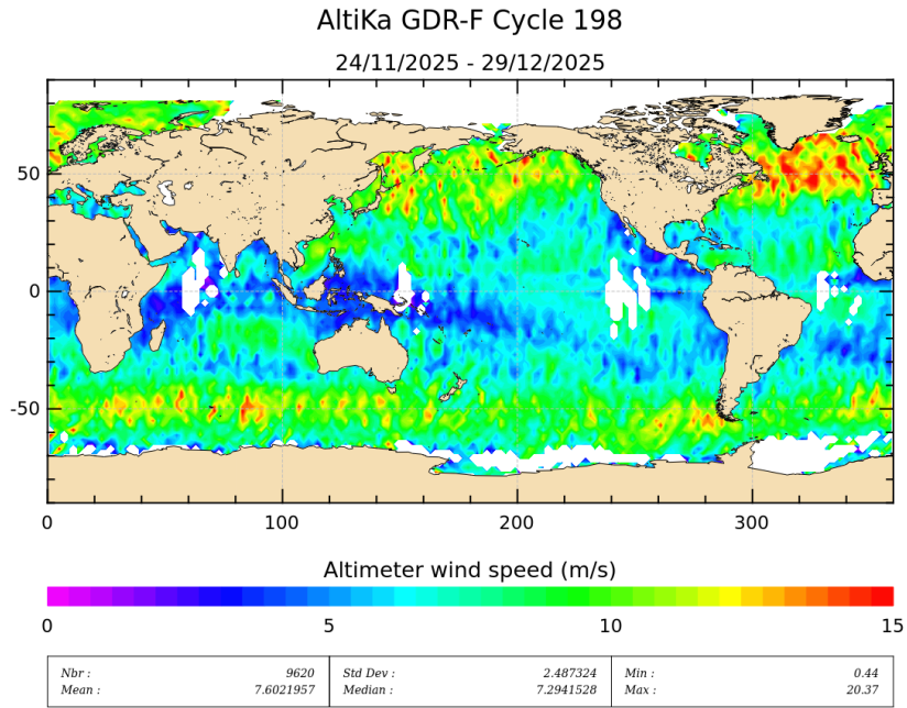
Figure 9: Altimeter wind speed for cycle 198.
