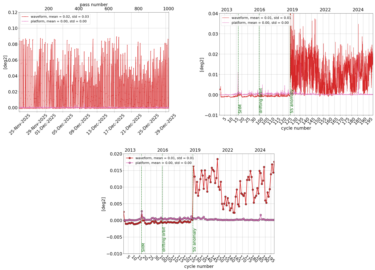
Figure 13: Monitoring per pass for cycle 198 (left), daily monitoring(right) and cyclic monitoring (bottom) of SARAL/AltiKa's mispointing angle: comparison between the one derived from waveform retracking and the one measured by platform startrackers.
