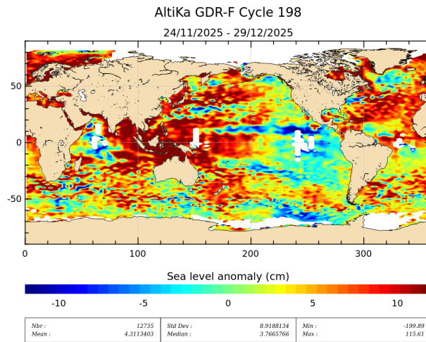
Figure 19: Sea level anomaly relative to MSS for cycle 198.
