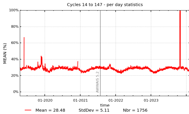
Total invalid data from beam 10 (non continental)
