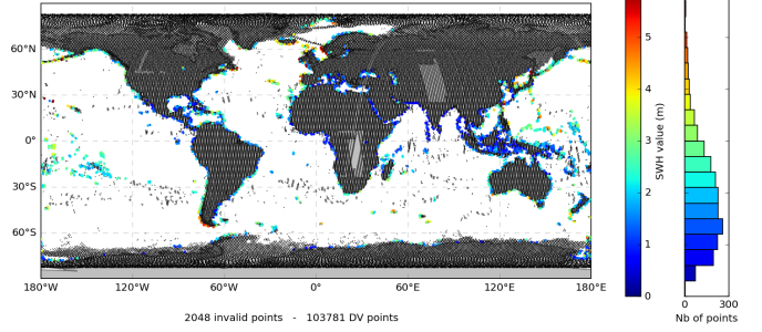
SWH 10 (colors) edited from thresholds and quality flags (Black = default Values)
