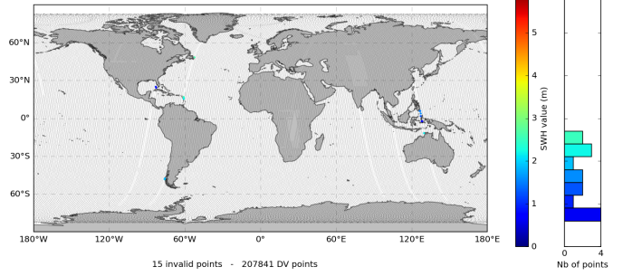
SWH 08 (colors) edited from thresholds and quality flags (Black = default Values)
