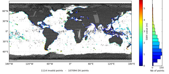
SWH 10 (colors) edited from thresholds and quality flags (Black = default Values)
