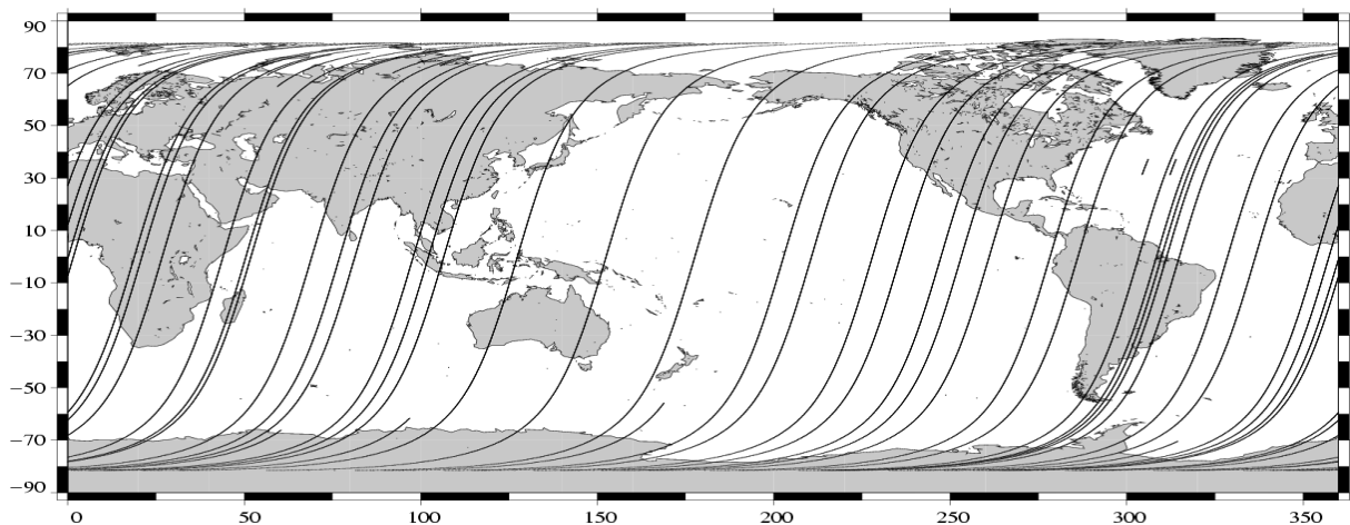
Missing measurements (Descending passes) Envisat Cycle 011 (04/11/2002 / 09/12/2002)
