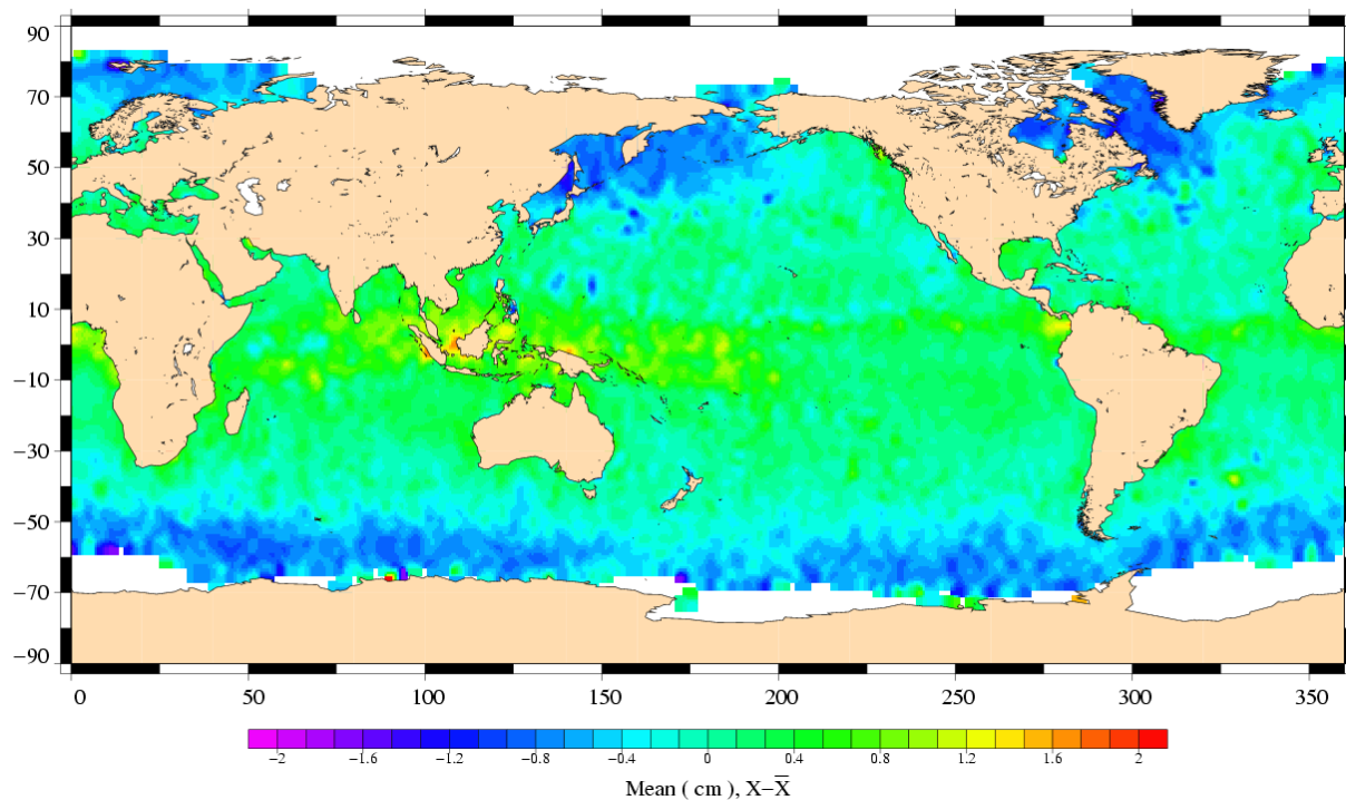
Radiometer correction differences ERS-2 (Cycle 079) – Envisat (Cycle 011)
