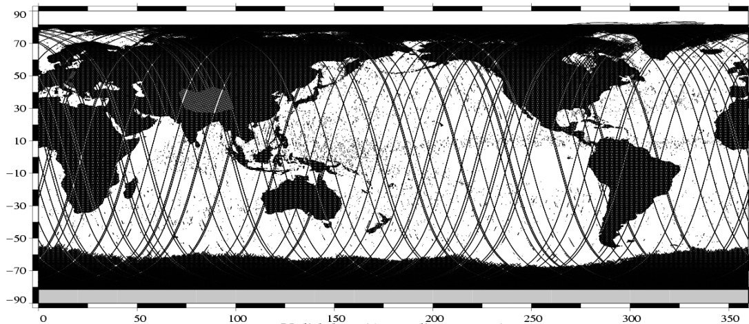
Valid data (Ascending passes) Envisat Cycle 018 (07/07/2003 / 11/08/2003)
