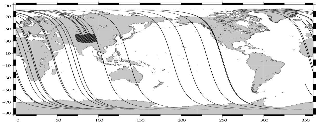
Missing measurements (Descending passes) Envisat Cycle 018 (07/07/2003 / 11/08/2003)
