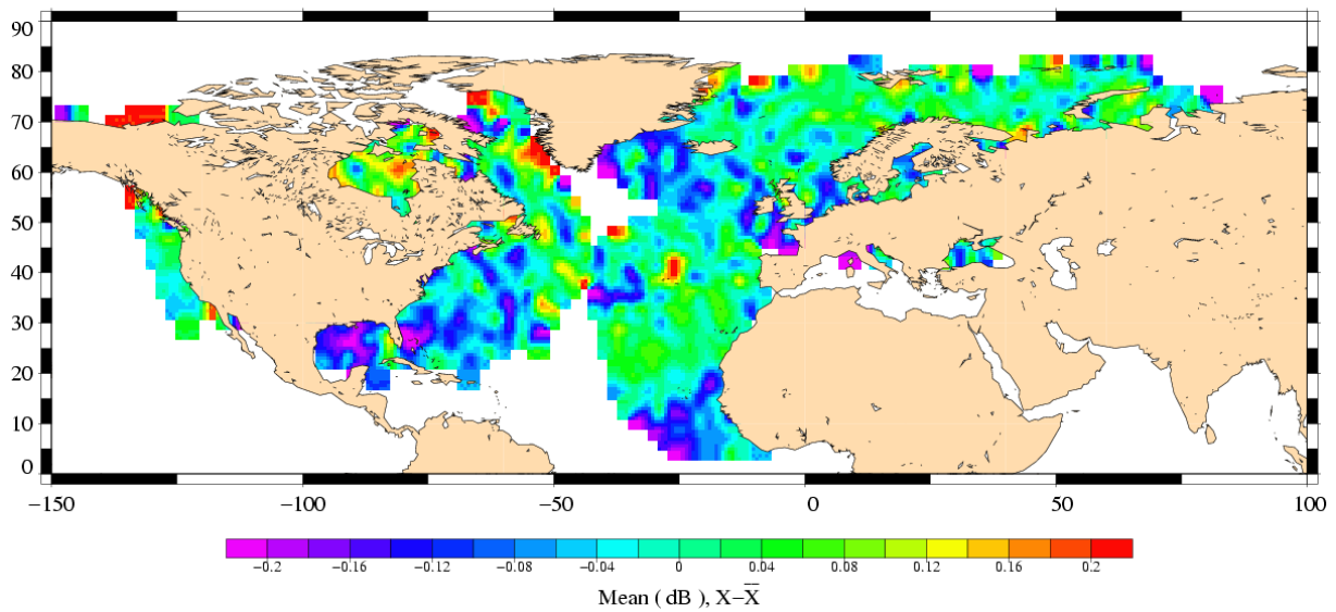
Sigma0 differences ERS-2 (Cycle 086) – Envisat (Cycle 018)
