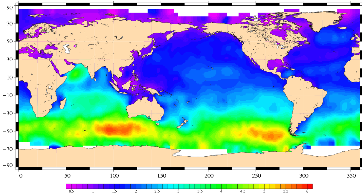
Significant Wave Height (m) Envisat Cycle 018 07/07/2003 – 11/08/2003
