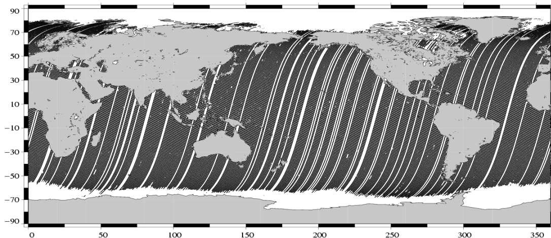
Valid data (Descending passes) Envisat Cycle 018 (07/07/2003 / 11/08/2003)
