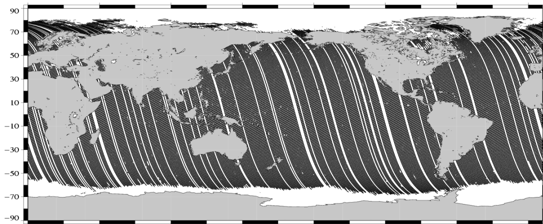
Valid data (Descending passes) Envisat Cycle 018 (07/07/2003 / 11/08/2003)
