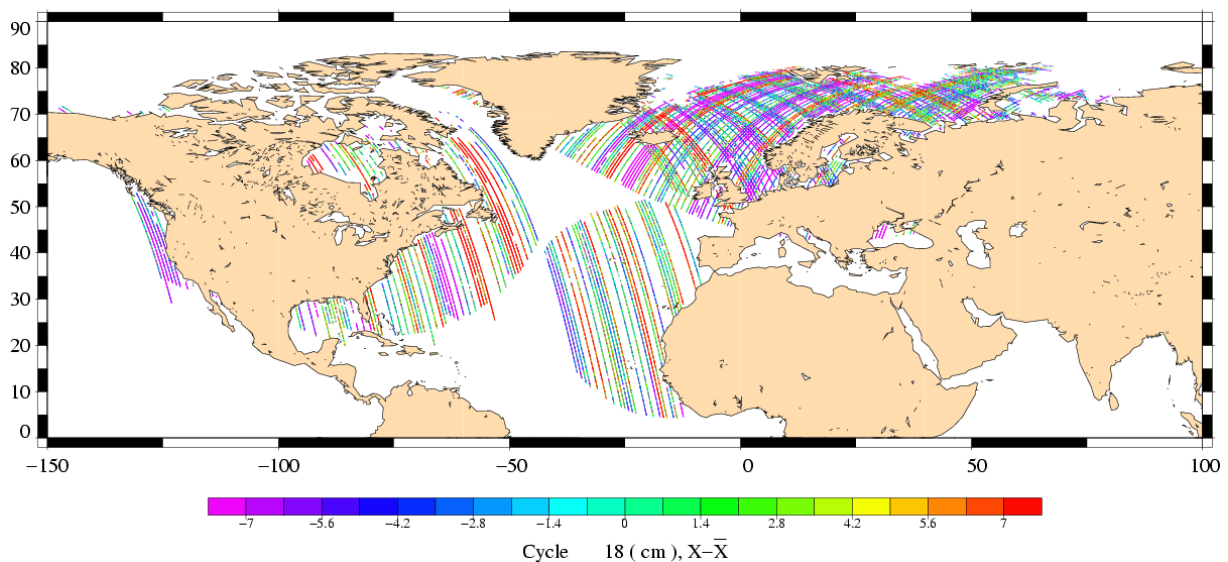
Corrected SLA (model configuration) ERS-2 (Cycle 086) – Envisat (Cycle 018)
