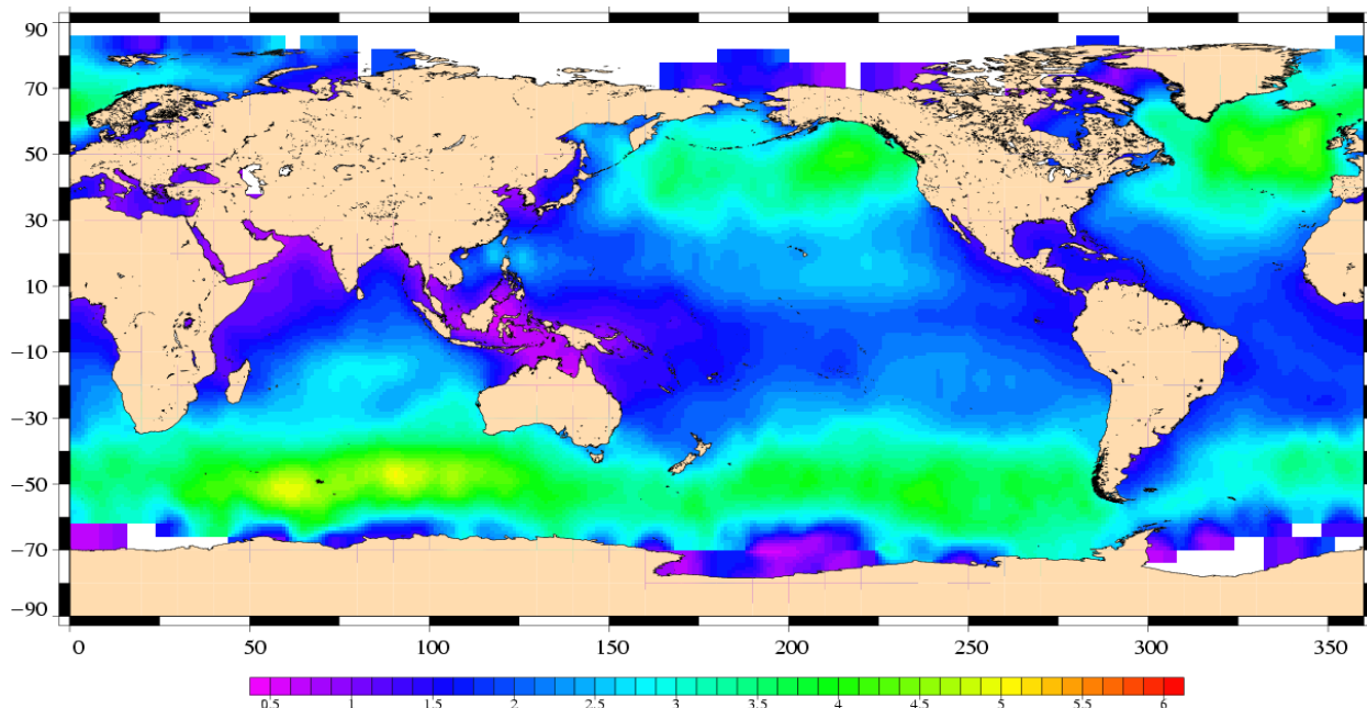
Significant Wave Height (m) Envisat Cycle 042 24/10/2005 – 28/11/2005
