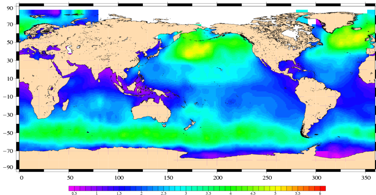
Significant Wave Height (m) Envisat Cycle 065 07/01/2008 – 11/02/2008
