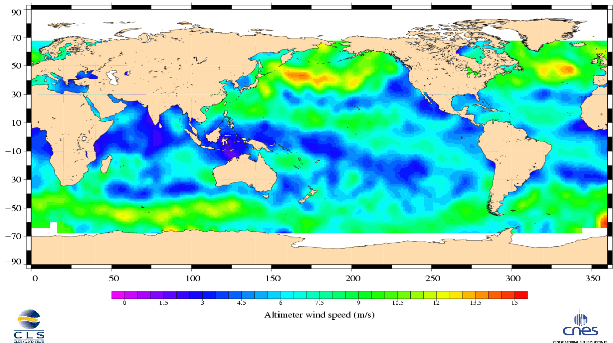
Jason-1 Cycle 032 18/11/2002 – 28/11/2002
