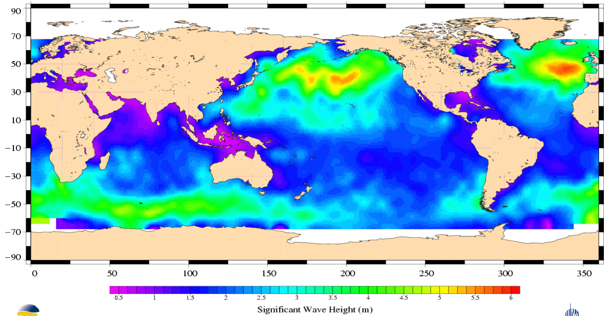
Jason-1 Cycle 032 18/11/2002 – 28/11/2002
