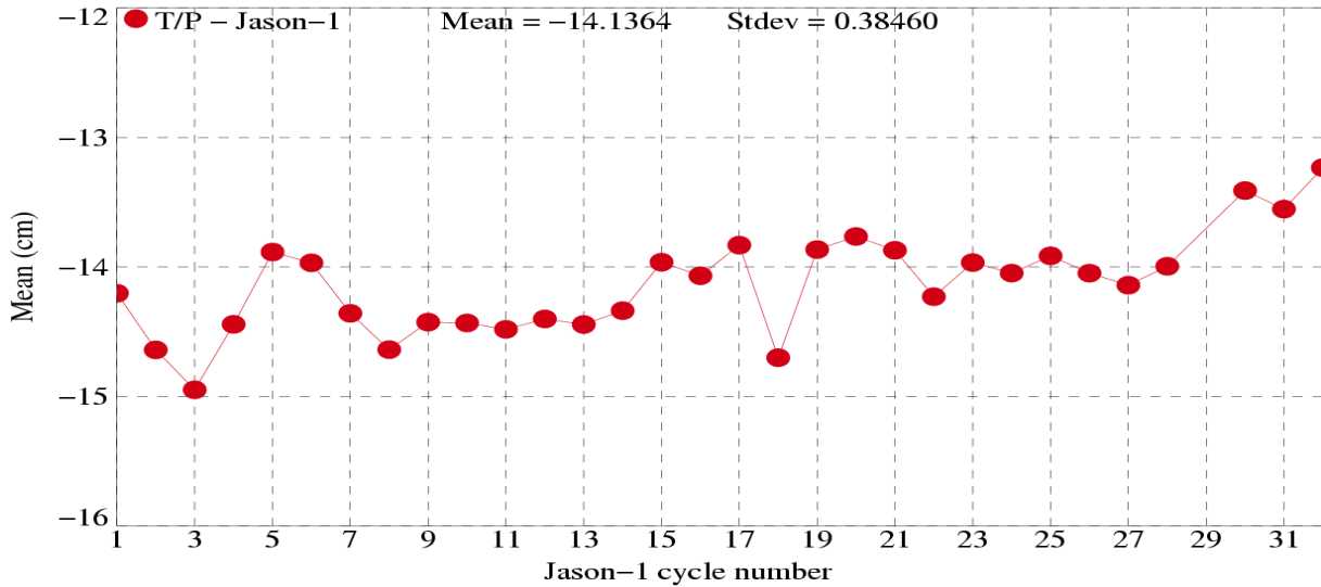
Crossover mean
