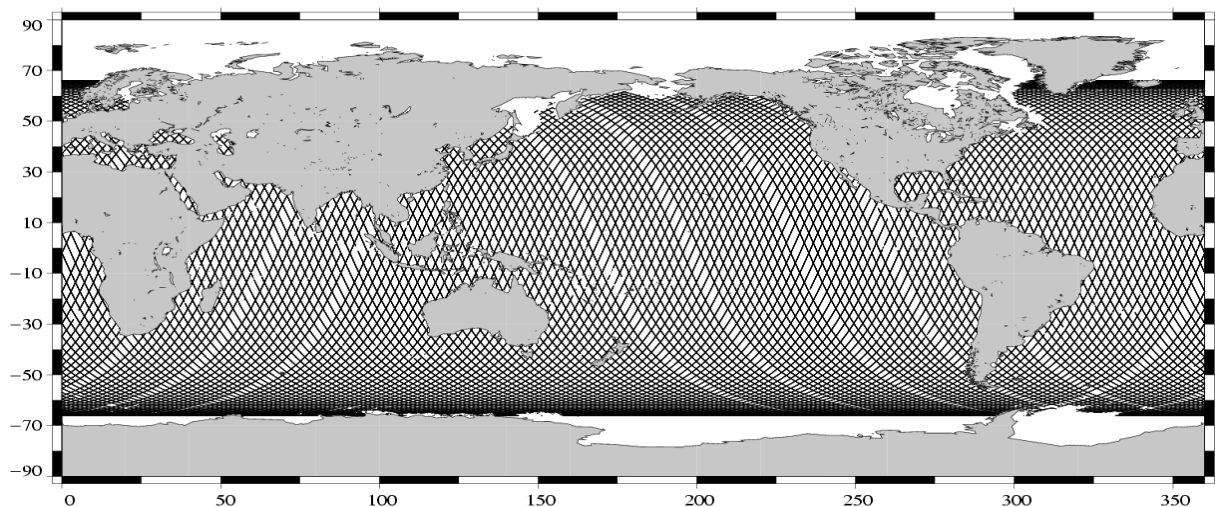
Valid data Jason-1 Cycle 042 (25/02/2003 / 07/03/2003)
