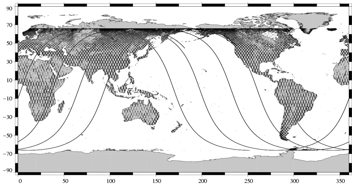
Missing measurements Jason-1 Cycle 042 (25/02/2003 / 07/03/2003)
