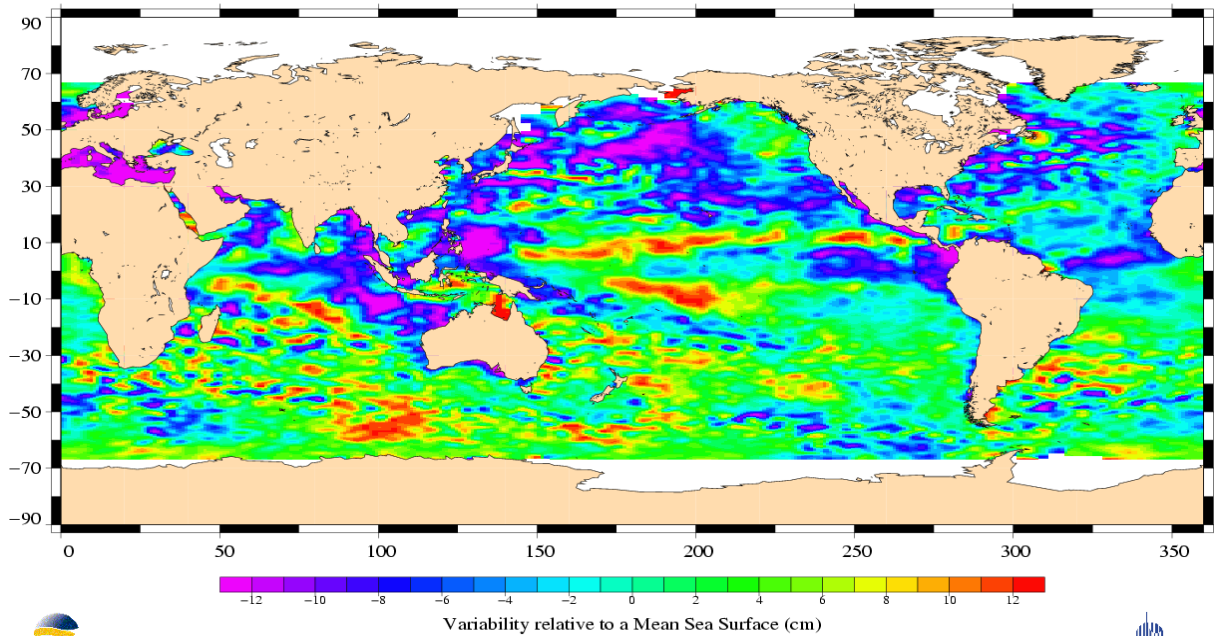
(SSH – MSS) differences greater than 30 cm Jason / Cycle 042
