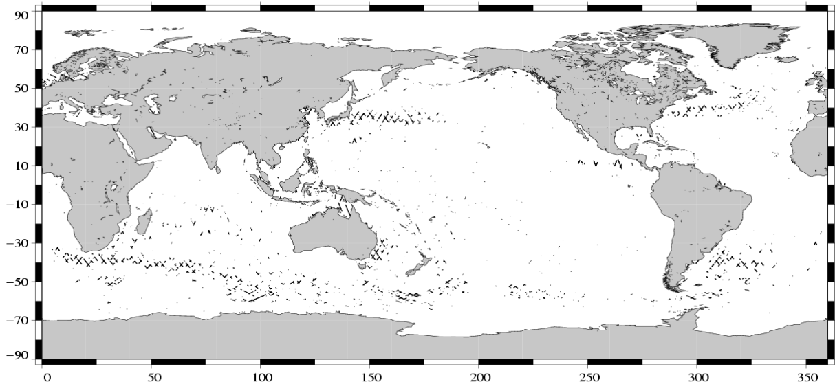
(SSH – MSS) differences greater than 30 cm Jason / Cycle 042
