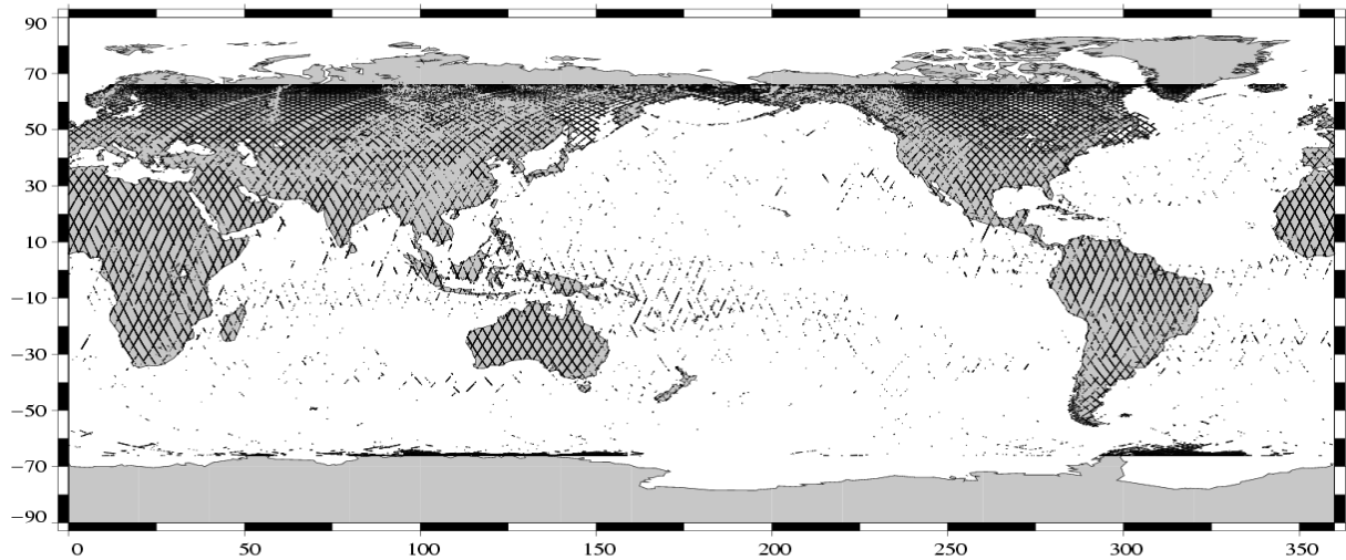
Edited measurements Jason-1 Cycle 042 (25/02/2003 / 07/03/2003)
