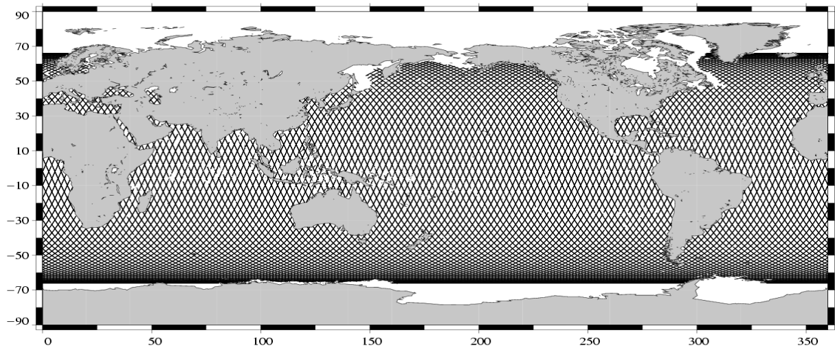
Valid data Jason-1 Cycle 044 (17/03/2003 / 27/03/2003)
