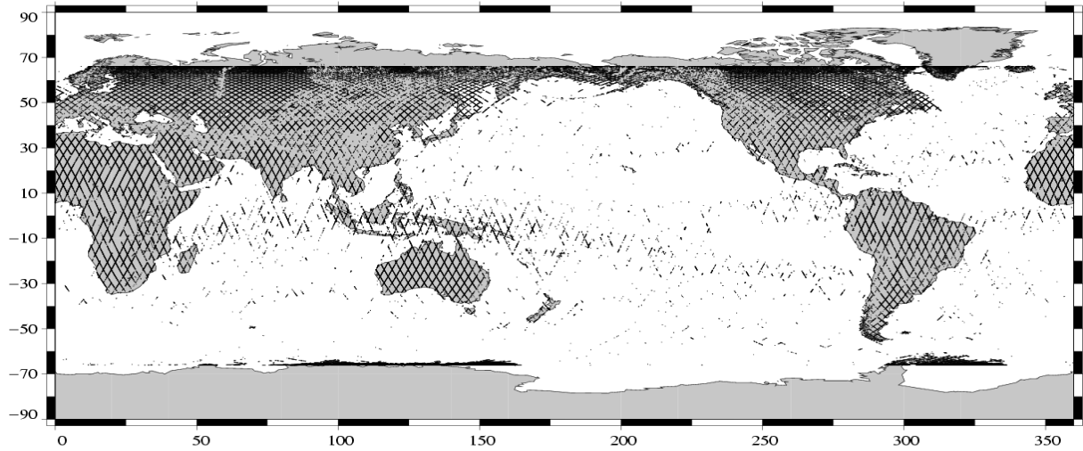
Edited measurements Jason-1 Cycle 044 (17/03/2003 / 27/03/2003)
