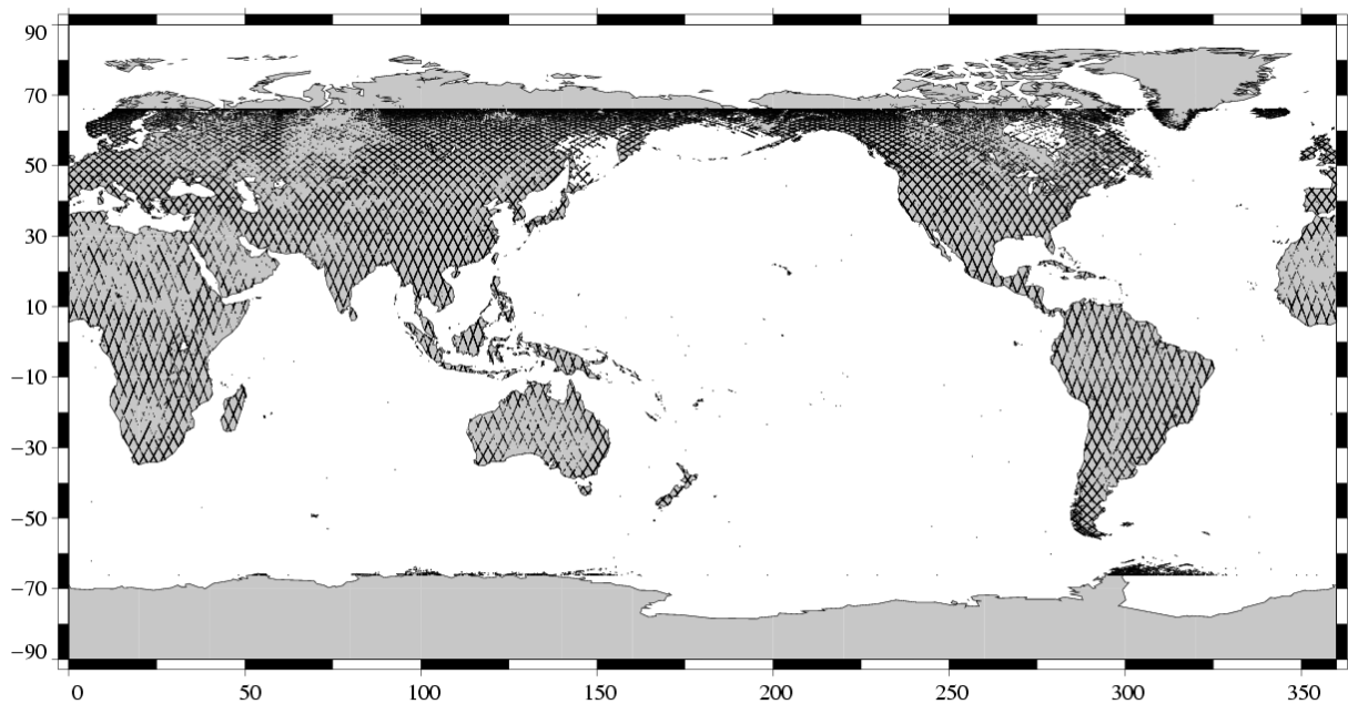
Missing measurements Jason-1 Cycle 044 (17/03/2003 / 27/03/2003)
