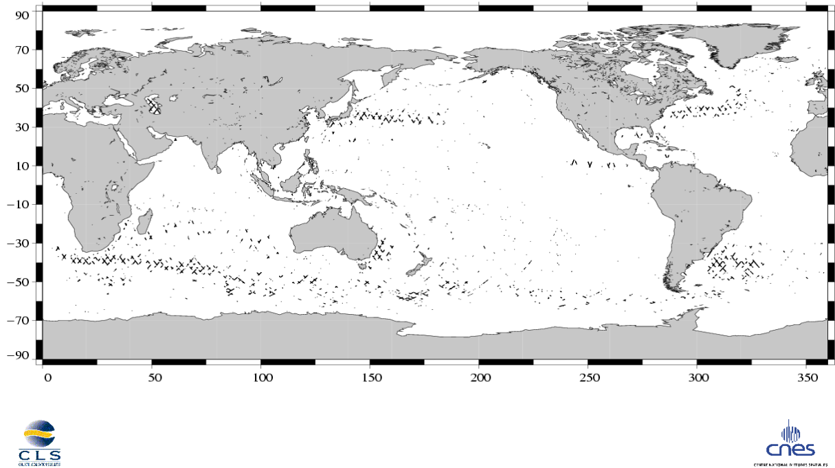
(SSH – MSS) differences greater than 30 cm Jason / Cycle 044
