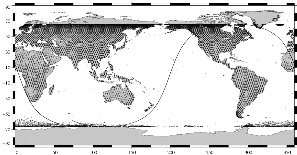
Missing measurements Jason-1 Cycle 062 (12/09/2003 / 21/09/2003)
