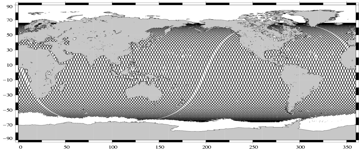
Valid data Jason-1 Cycle 062 (12/09/2003 / 21/09/2003)
