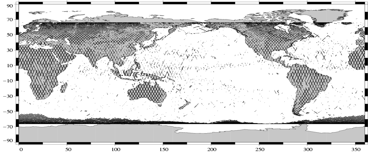
Edited measurements Jason-1 Cycle 062 (12/09/2003 / 21/09/2003)
