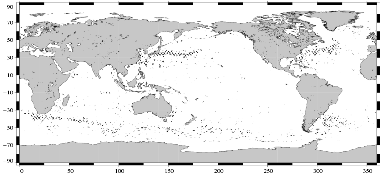
(SSH – MSS) differences greater than 30 cm Jason / Cycle 062
