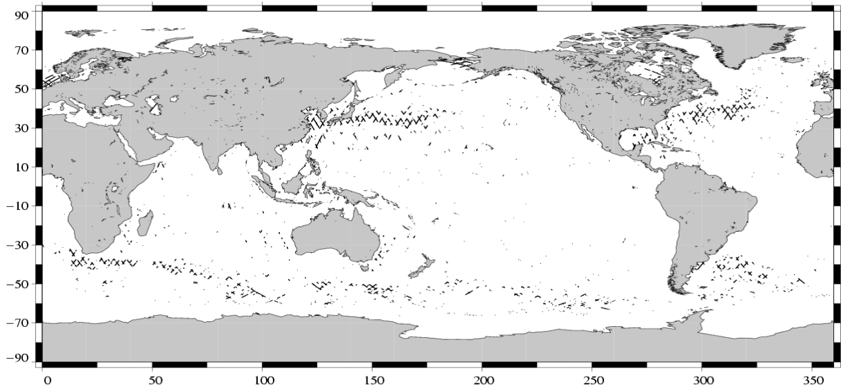
(SSH – MSS) differences greater than 30 cm Jason / Cycle 064
