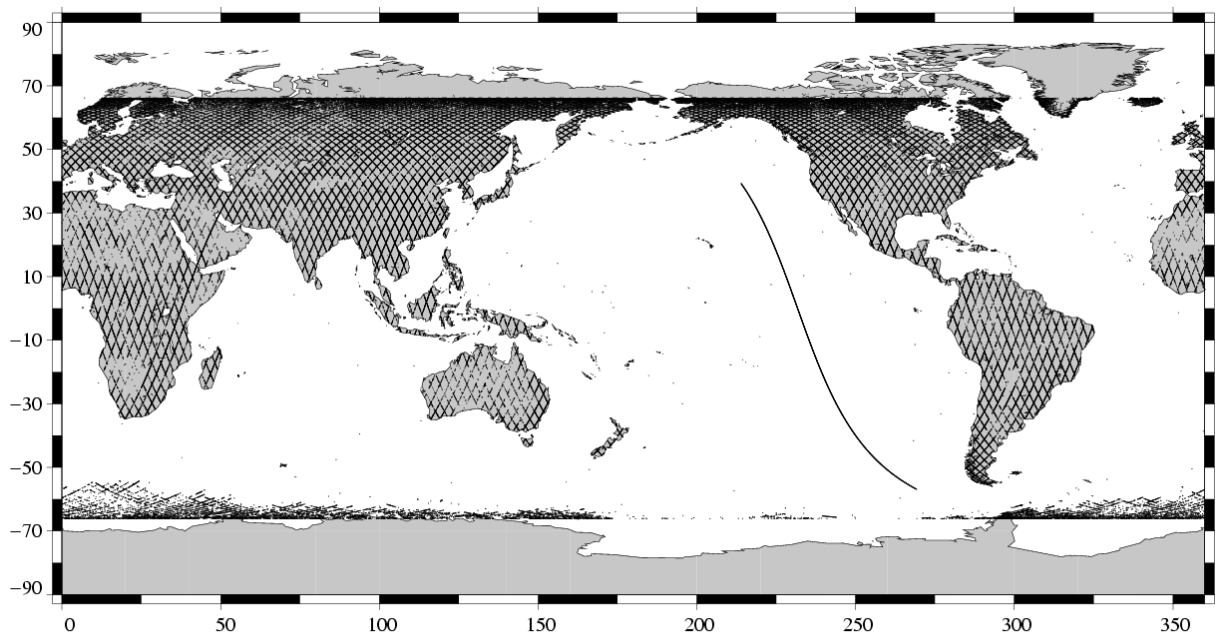
Missing measurements Jason-1 Cycle 064 (01/10/2003 / 11/10/2003)
