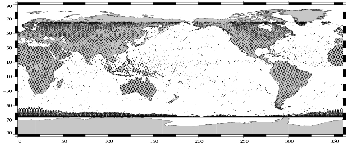
Edited measurements Jason-1 Cycle 064 (01/10/2003 / 11/10/2003)
