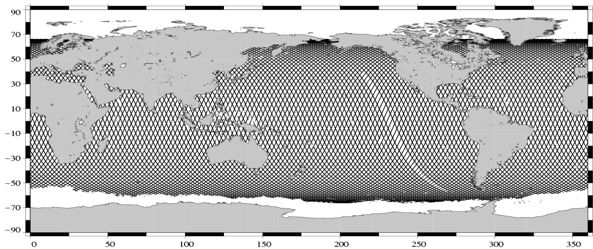
Valid data Jason-1 Cycle 064 (01/10/2003 / 11/10/2003)
