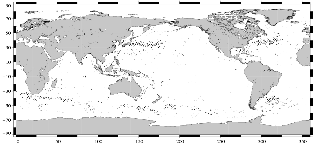
(SSH – MSS) differences greater than 30 cm Jason / Cycle 065
