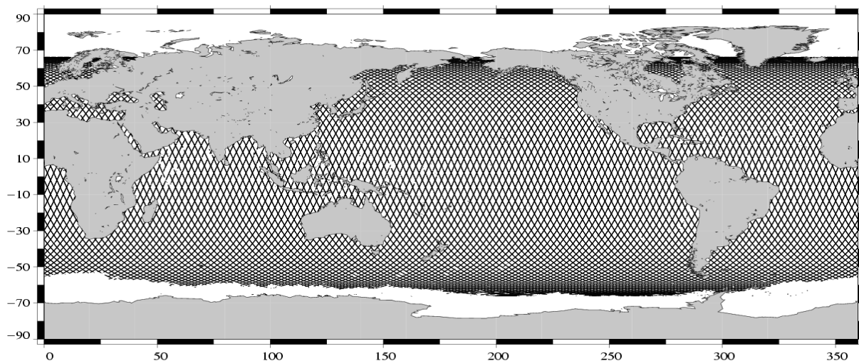
Valid data Jason-1 Cycle 065 (11/10/2003 / 21/10/2003)
