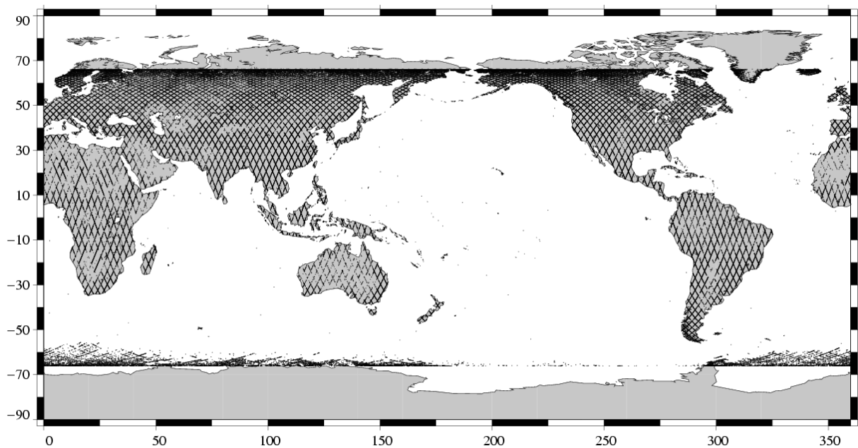
Missing measurements Jason-1 Cycle 065 (11/10/2003 / 21/10/2003)
