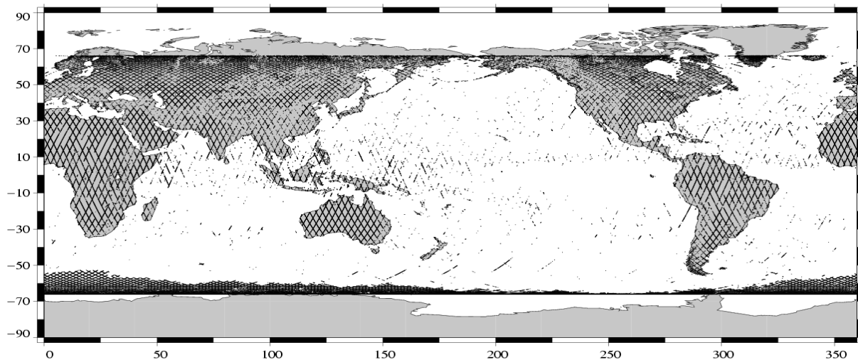
Edited measurements Jason-1 Cycle 065 (11/10/2003 / 21/10/2003)
