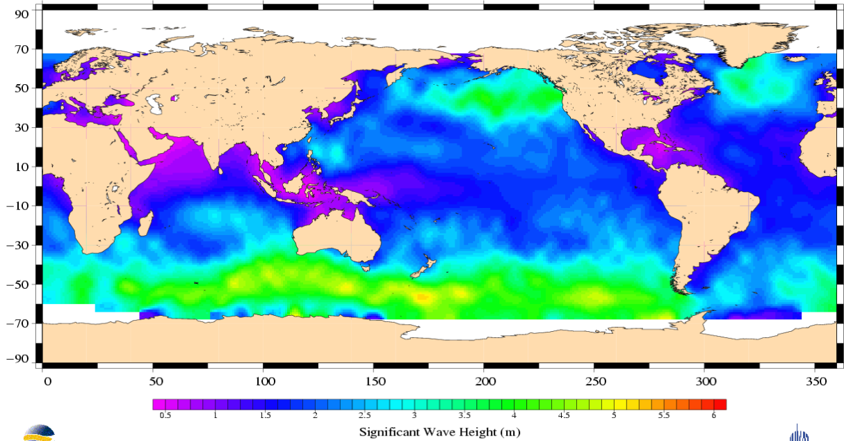
Jason-1 Cycle 065 11/10/2003 – 21/10/2003
