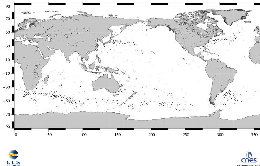
(SSH – MSS) differences greater than 30 cm Jason / Cycle 082
