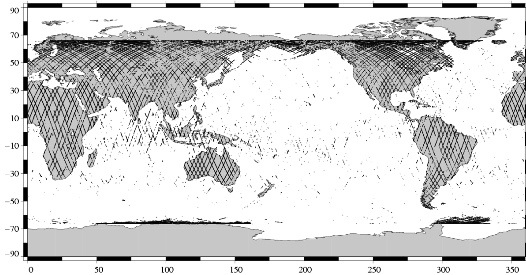
Edited measurements Jason-1 Cycle 082 (28/03/2004 / 07/04/2004)
