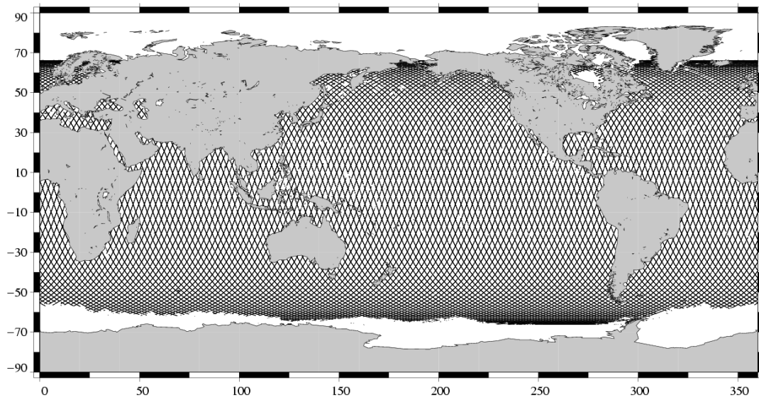
Valid data Jason-1 Cycle 093 (15/07/2004 / 25/07/2004)
