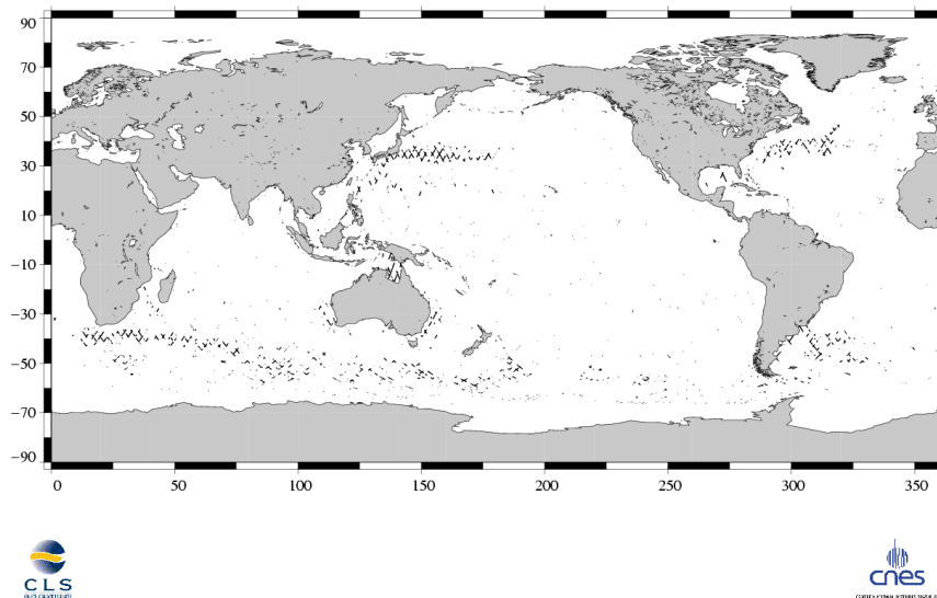
(SSH - MSS) differences greater than 30 cm Jason / Cycle 093
