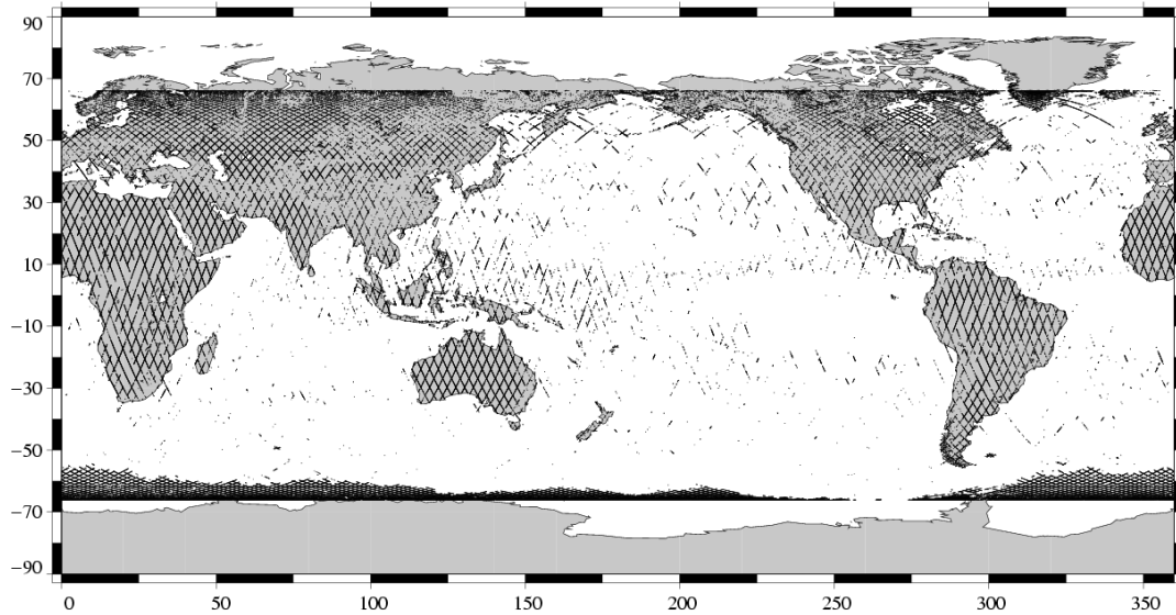
Edited measurements Jason-1 Cycle 093 (15/07/2004 / 25/07/2004)
