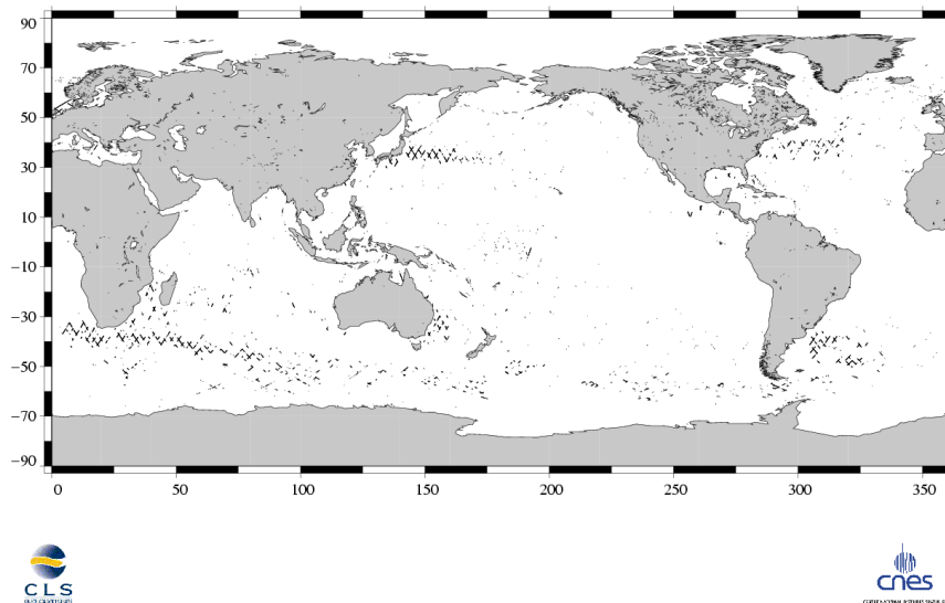
(SSH - MSS) differences greater than 30 cm Jason / Cycle 114
