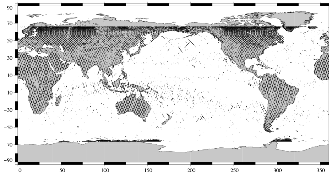
Edited measurements Jason-1 Cycle 114 (08/02/2005 / 18/02/2005)
