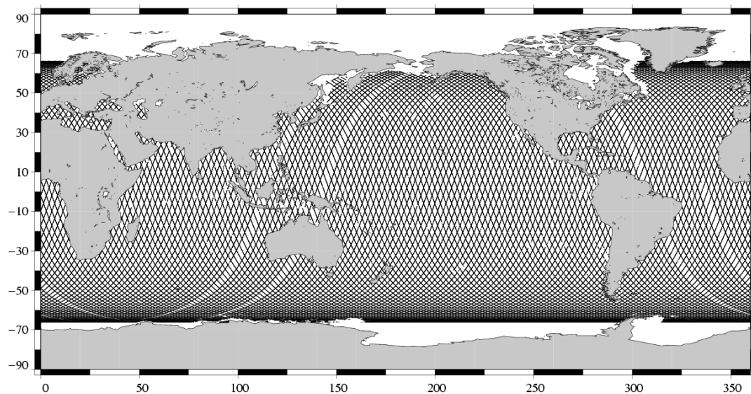
Valid data Jason-1 Cycle 114 (08/02/2005 / 18/02/2005)
