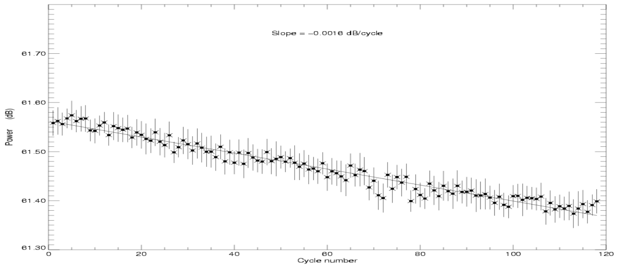
POSEIDON2 – Cycle 118
