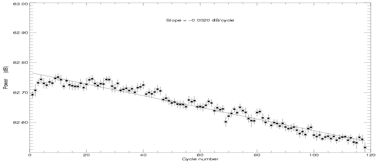
POSEIDON2 – Cycle 118
