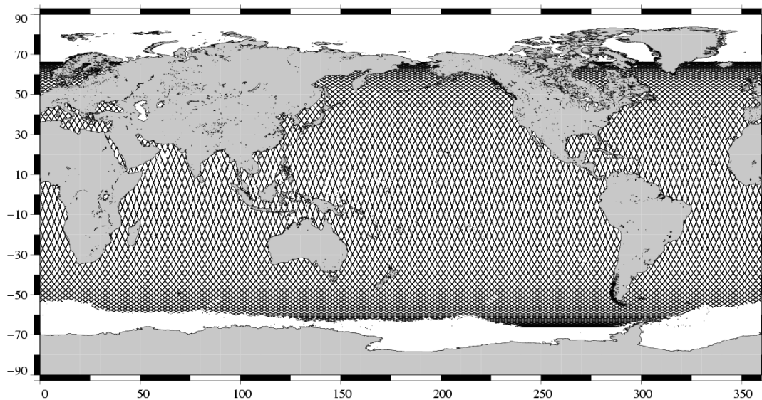
Valid data Jason-1 Cycle 138 (04/10/2005 / 14/10/2005)
