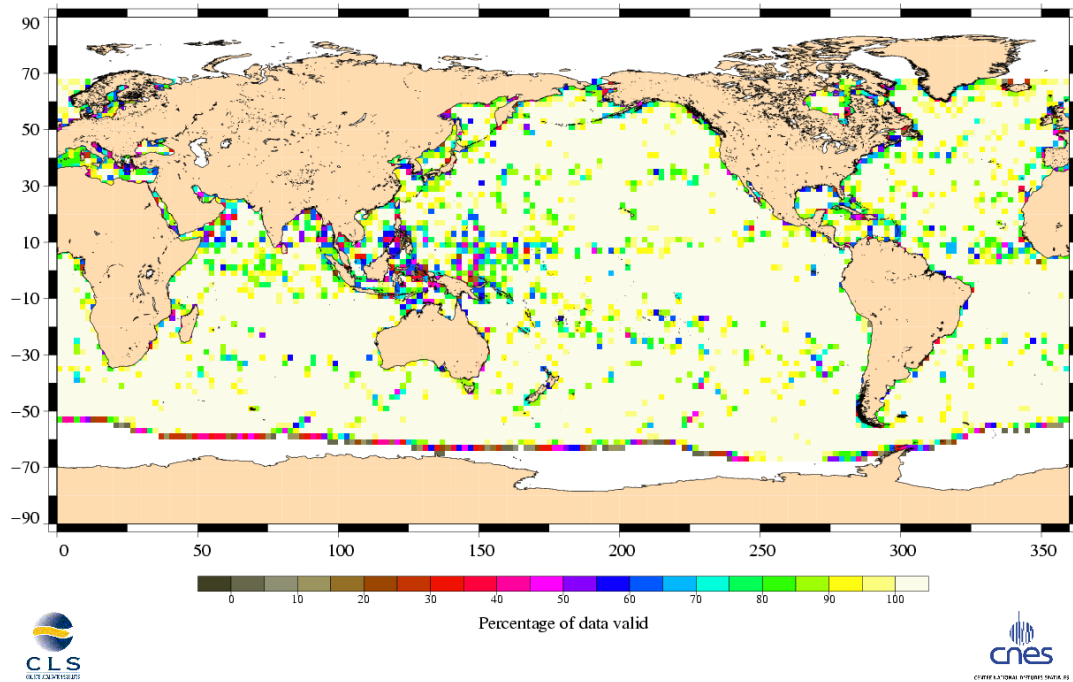
Percentage of valid data relative to the nominal pass Jason-1 Cycle 138 (04/10/2005 / 14/10/2005)
