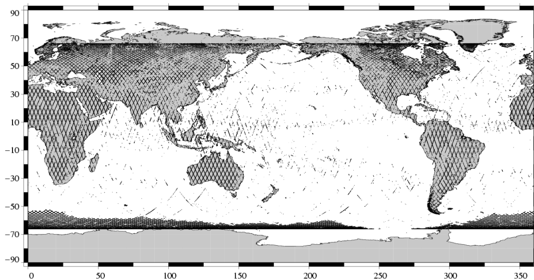
Edited measurements Jason-1 Cycle 138 (04/10/2005 / 14/10/2005)
