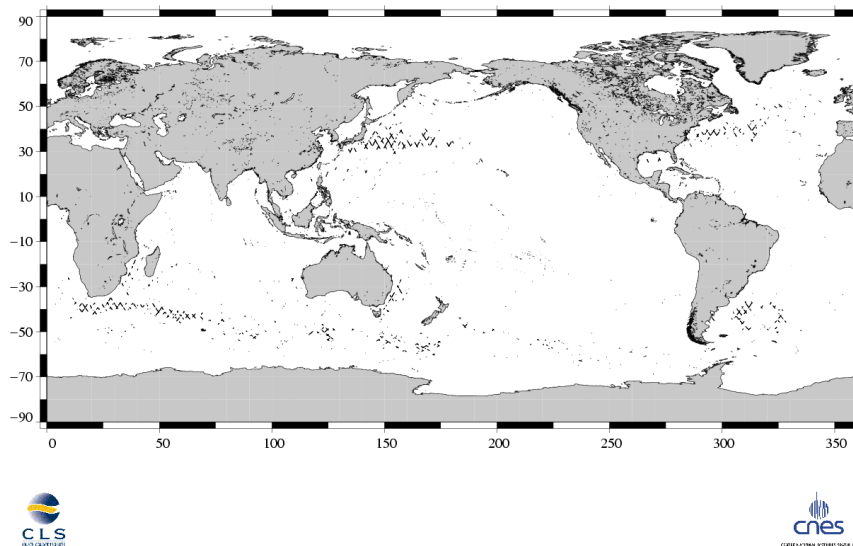
(SSH – MSS) differences greater than 30 cm Jason / Cycle 138
