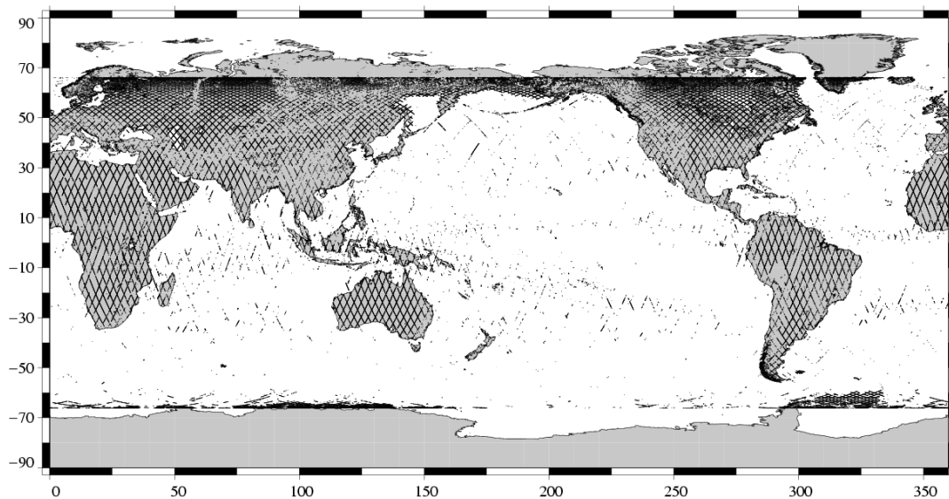
Edited measurements Jason-1 Cycle 148 (11/01/2006 / 21/01/2006)
