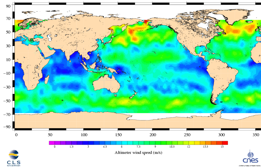
Jason-1 Cycle 148 11/01/2006 – 21/01/2006
