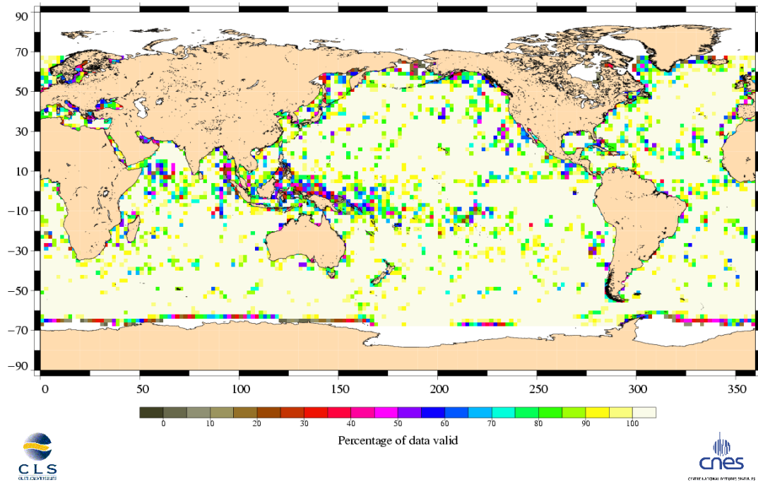
Percentage of valid data relative to the nominal pass Jason-1 Cycle 160 (10/05/2006 / 20/05/2006)
