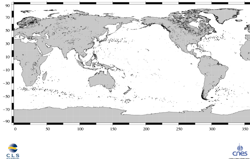
(SSH – MSS) differences greater than 30 cm Jason / Cycle 160
