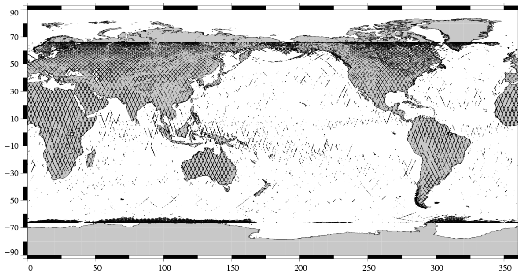
Edited measurements Jason-1 Cycle 160 (10/05/2006 / 20/05/2006)
