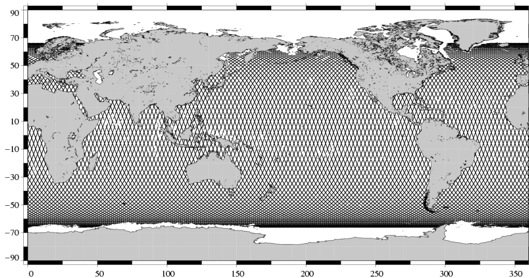
Valid data Jason-1 Cycle 160 (10/05/2006 / 20/05/2006)
