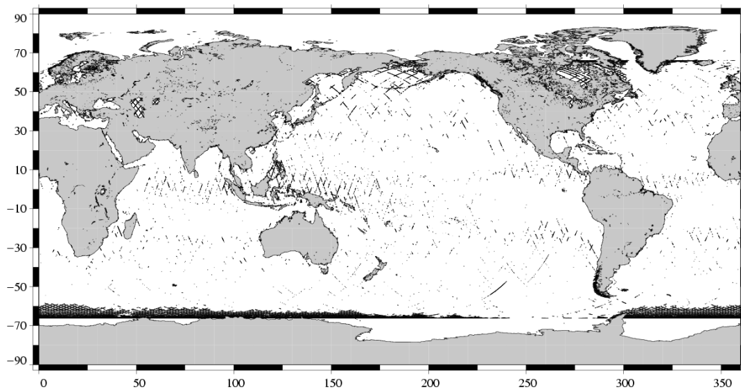
Edited measurements Jason-1 Cycle 163 (09/06/2006 / 19/06/2006)
