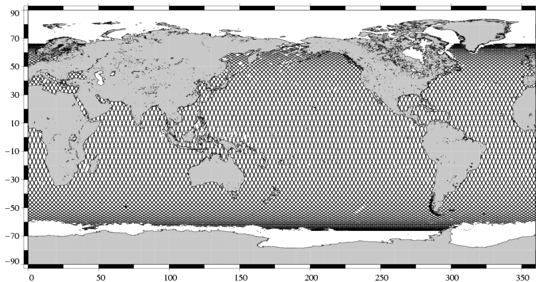
Valid data Jason-1 Cycle 163 (09/06/2006 / 19/06/2006)
