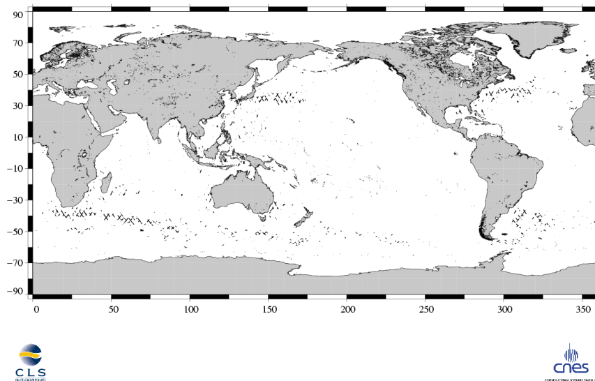
(SSH – MSS) differences greater than 30 cm Jason / Cycle 163
