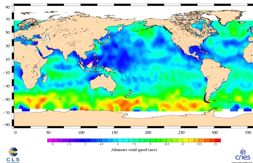
Jason-1 Cycle 172 06/09/2006 - 16/09/2006
