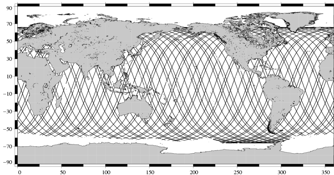
Valid data Jason-1 Cycle 177 (26/10/2006 / 30/10/2006)
