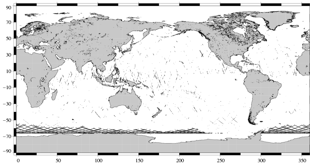
Edited measurements Jason-1 Cycle 177 (26/10/2006 / 30/10/2006)
