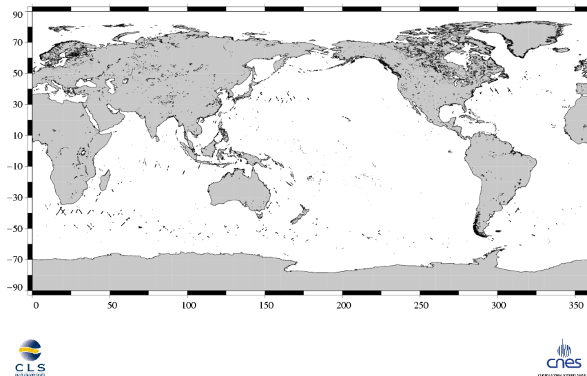
(SSH – MSS) differences greater than 30 cm Jason / Cycle 177
