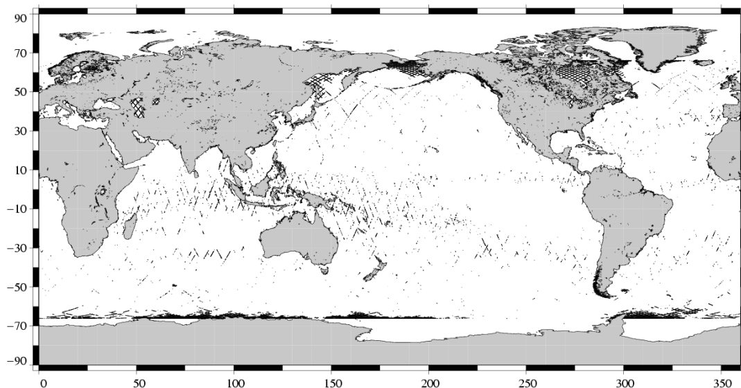
Edited measurements Jason-1 Cycle 184 (03/01/2007 / 13/01/2007)
