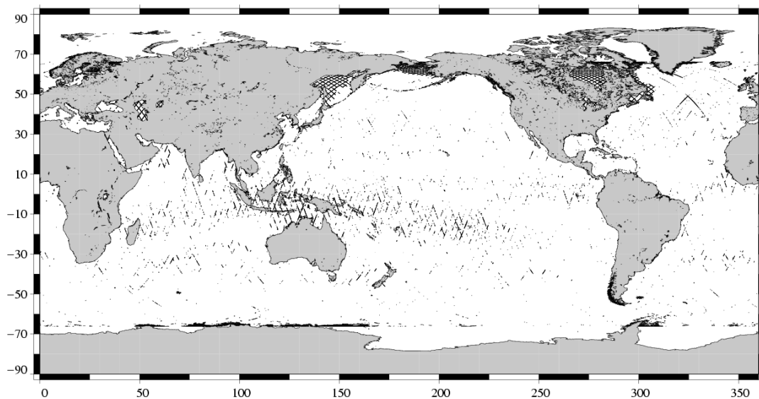
Edited measurements Jason-1 Cycle 188 (12/02/2007 / 22/02/2007)
