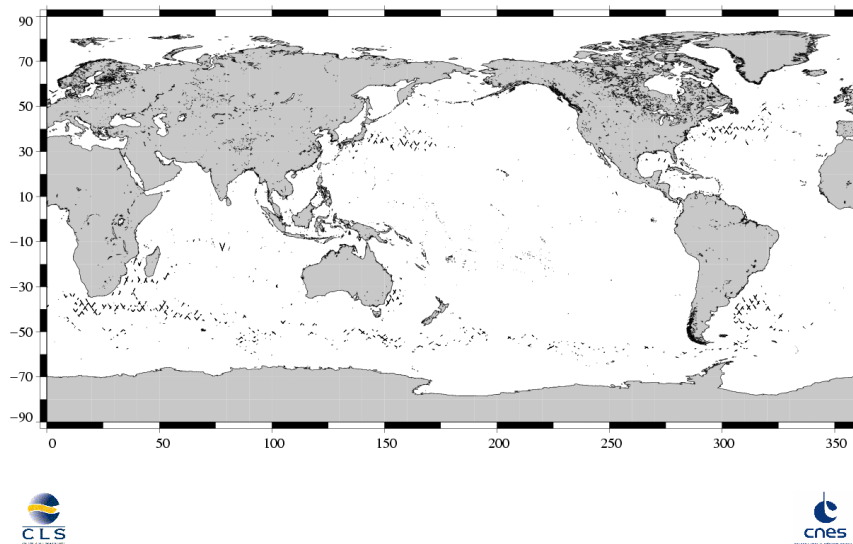
(SSH – MSS) differences greater than 30 cm Jason / Cycle 188
