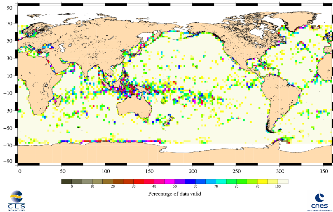
Percentage of valid data relative to the nominal pass Jason-1 Cycle 188 (12/02/2007 / 22/02/2007)
