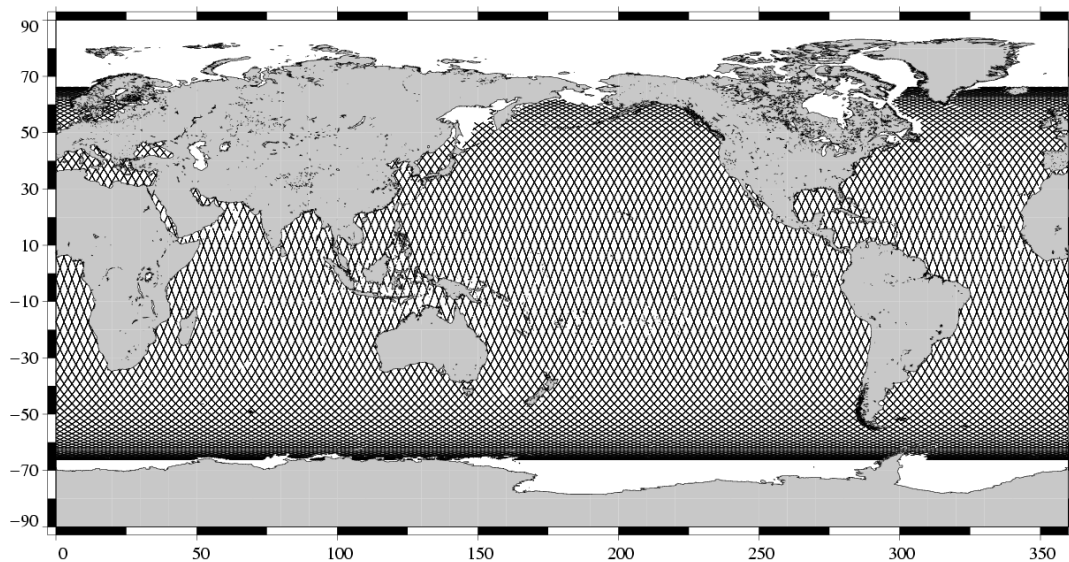
Valid data Jason-1 Cycle 188 (12/02/2007 / 22/02/2007)
