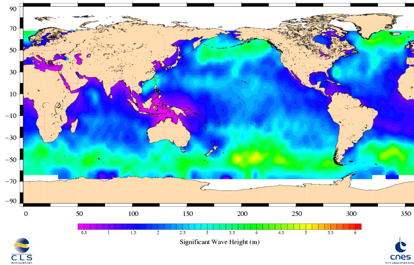
Jason-1 Cycle 214 28/10/2007 - 07/11/2007
