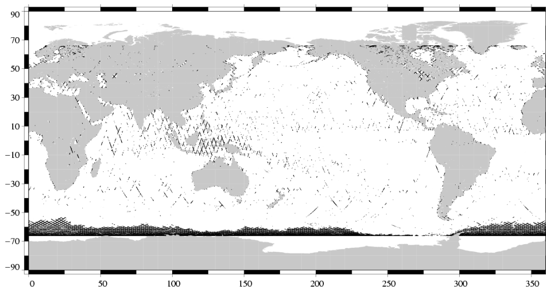
Edited measurements Jason-1 Cycle 214 (28/10/2007 / 07/11/2007)
