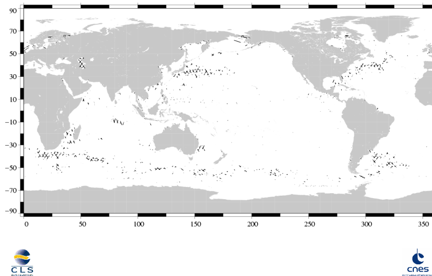
(SSH - MSS) differences greater than 30 cm Jason / Cycle 214
