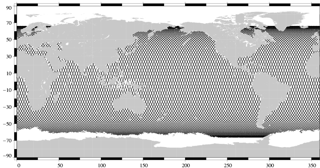
Valid data Jason-1 Cycle 214 (28/10/2007 / 07/11/2007)
