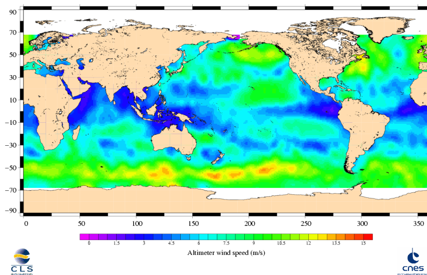
Jason-1 Cycle 228 15/03/2008 – 24/03/2008
