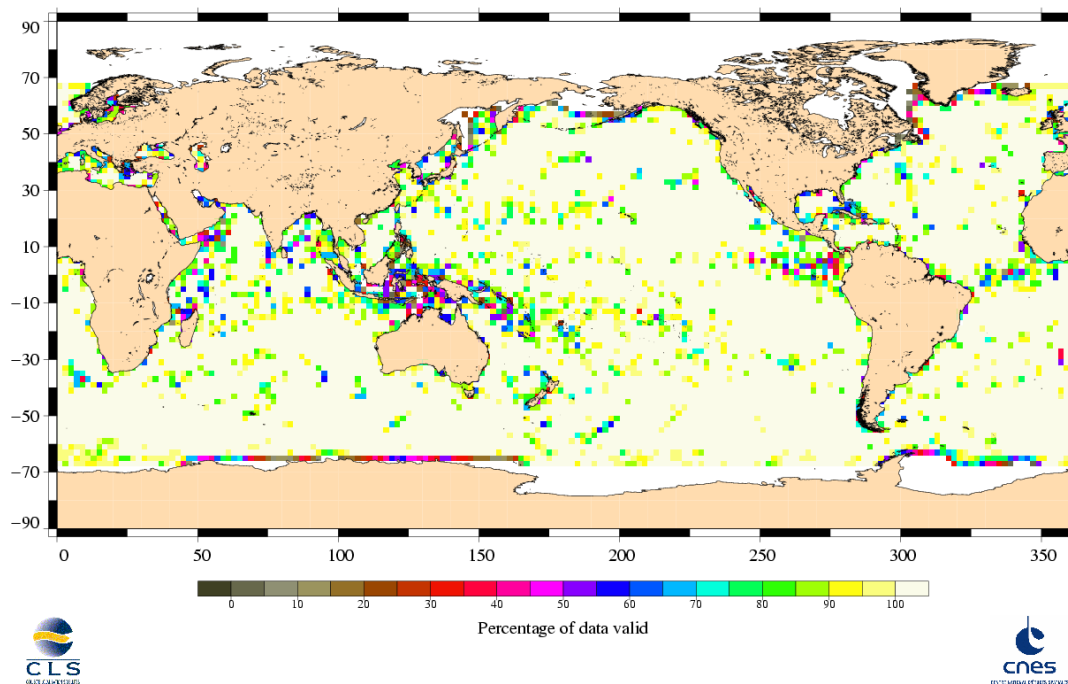
Percentage of valid data relative to the nominal pass Jason-1 Cycle 228 (15/03/2008 / 24/03/2008)
