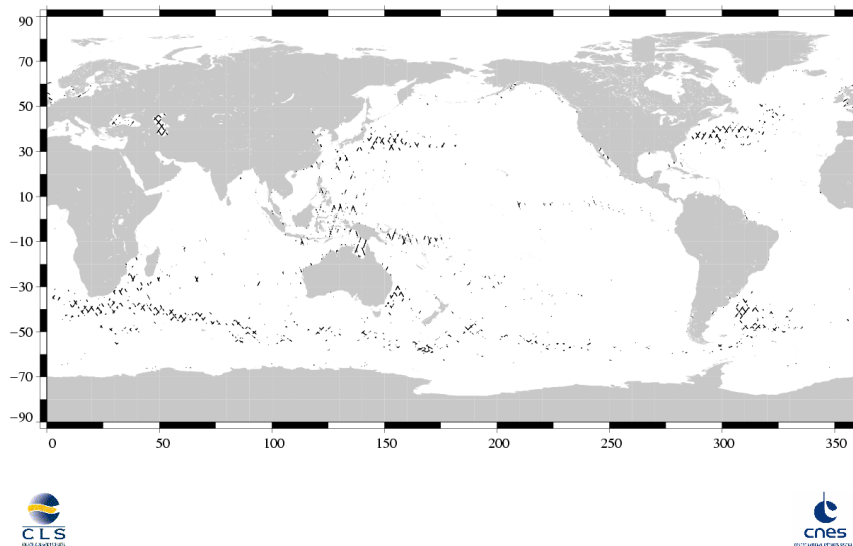
(SSH – MSS) differences greater than 30 cm Jason / Cycle 228
