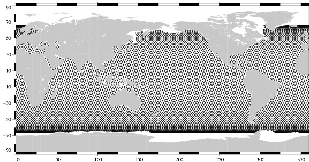
Valid data Jason-1 Cycle 228 (15/03/2008 / 24/03/2008)
