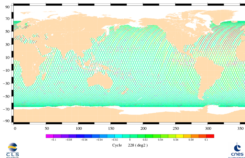
Square of the off nadir angle from waveforms Jason-1 Cycle 228 (15/03/2008 / 24/03/2008)
