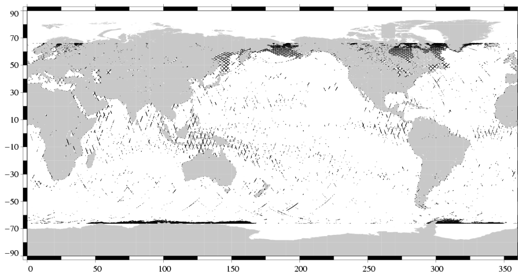
Edited measurements Jason-1 Cycle 228 (15/03/2008 / 24/03/2008)
