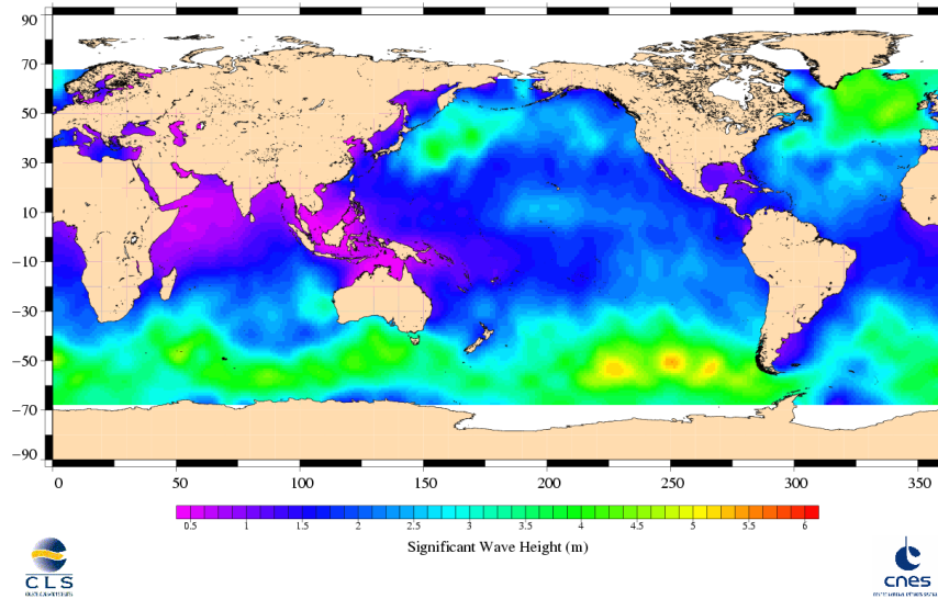
Jason-1 Cycle 229 24/03/2008 – 03/04/2008
