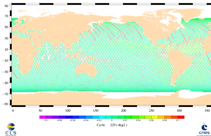
Square of the off nadir angle from waveforms Jason-1 Cycle 229 (24/03/2008 / 03/04/2008)
