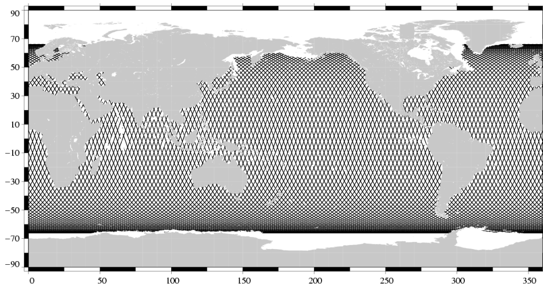
Valid data Jason-1 Cycle 229 (24/03/2008 / 03/04/2008)
