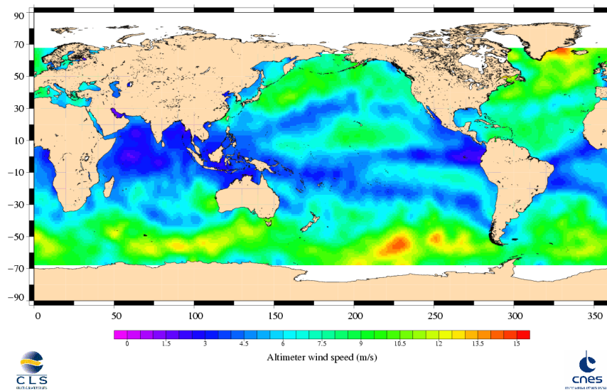
Jason-1 Cycle 229 24/03/2008 – 03/04/2008
