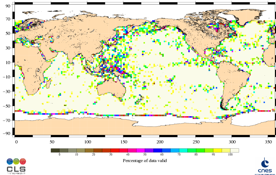
Percentage of valid data relative to the nominal pass Jason-1 Cycle 241 (21/07/2008 / 31/07/2008)
