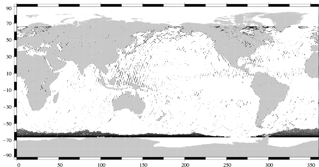
Edited measurements Jason-1 Cycle 241 (21/07/2008 / 31/07/2008)
