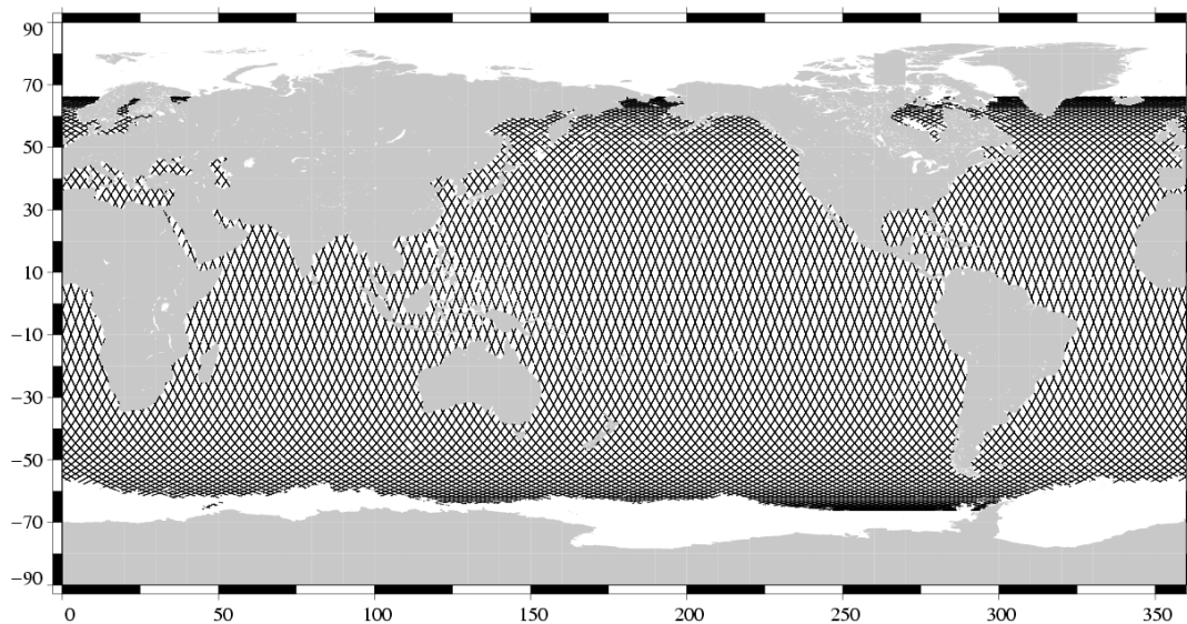
Valid data Jason-1 Cycle 241 (21/07/2008 / 31/07/2008)
