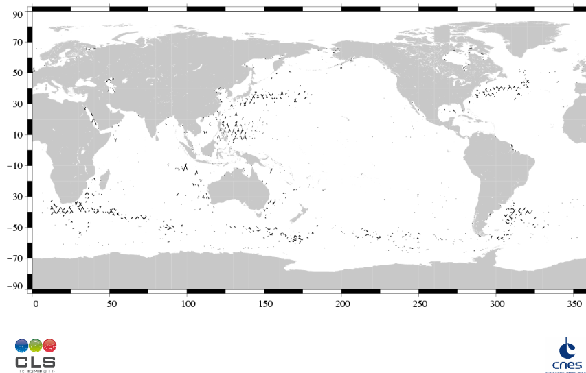
(SSH – MSS) differences greater than 30 cm Jason / Cycle 241
