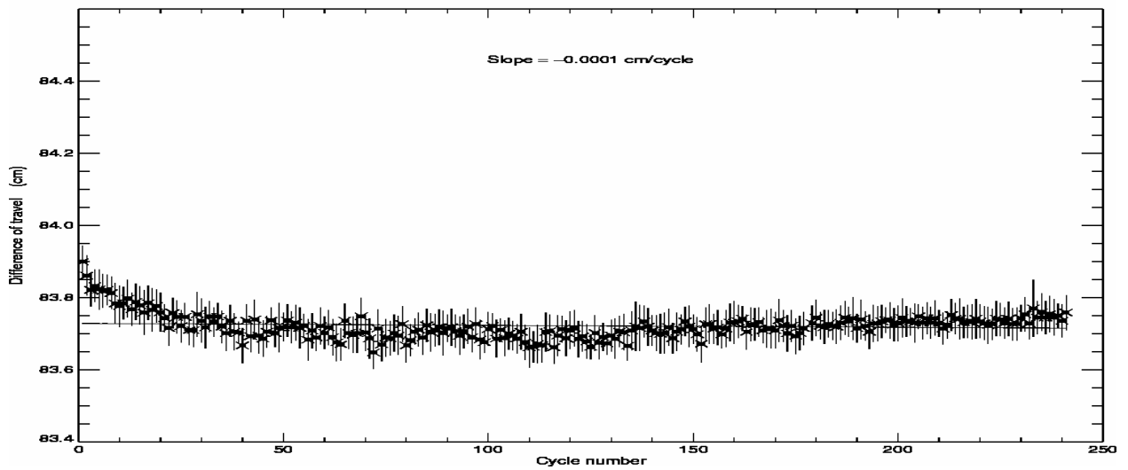
POSEIDON2 – Cycle 241 Difference of travel between E and R lines of the PTR in C band
