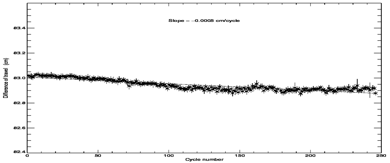
POSEIDON2 – Cycle 246 Difference of travel between E and R lines of the PTR in C band
