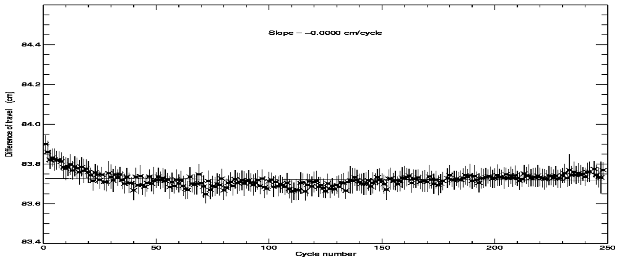
POSEIDON2 – Cycle 248 Difference of travel between E and R lines of the PTR in C band
