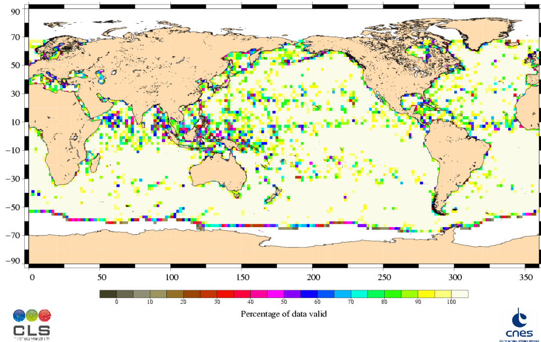
Percentage of valid data relative to the nominal pass Jason-1 Cycle 248 (29/09/2008 / 09/10/2008)
