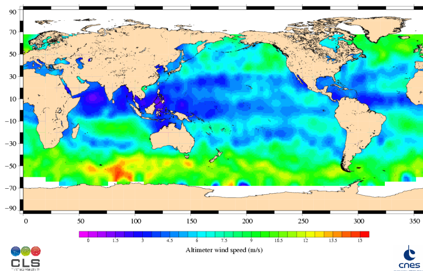
Jason-1 Cycle 248 29/09/2008 - 09/10/2008
