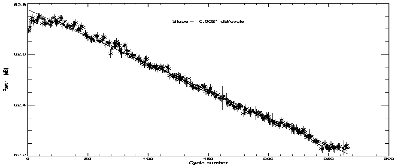
POSEIDON2 – Cycle 266 Total power of the PTR in C band
