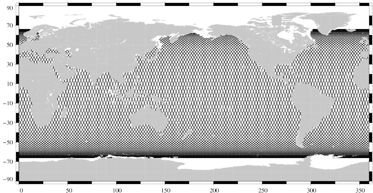
Valid data Jason-1 Cycle 297 (23/01/2010 / 02/02/2010)
