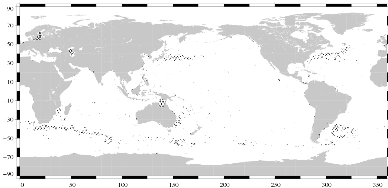
Valid data: (SSH – MSS) differences greater than 30 cm Jason-1 Cycle 297 (23/01/2010 / 02/02/2010)
