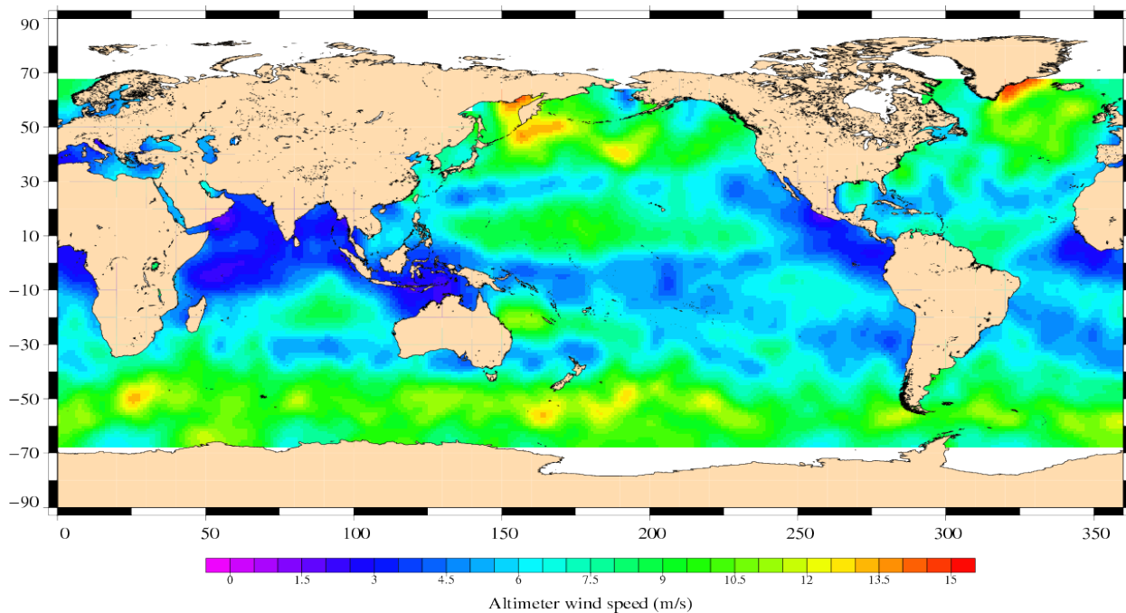
Jason-1 Cycle 302 13/03/2010 – 23/03/2010
