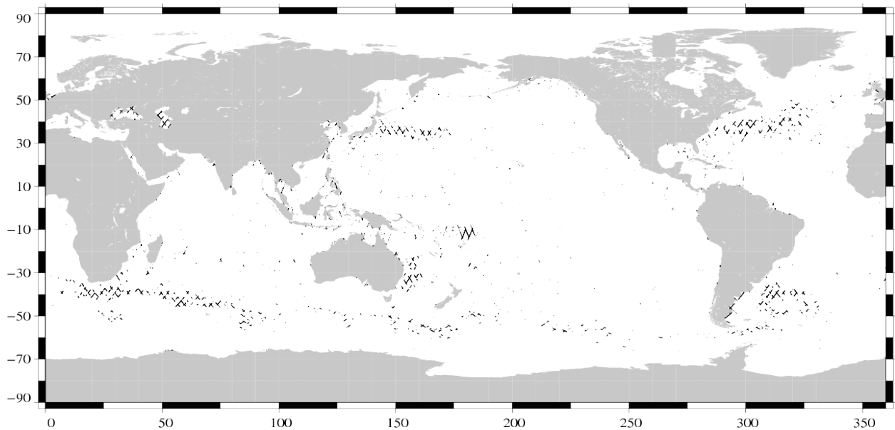
Valid data: (SSH – MSS) differences greater than 30 cm Jason-1 Cycle 302 (13/03/2010 / 23/03/2010)
