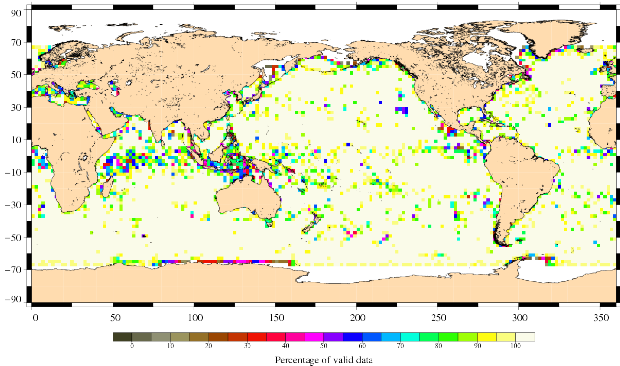
Percentage of valid data relative to the nominal pass Jason-1 Cycle 302 (13/03/2010 / 23/03/2010)
