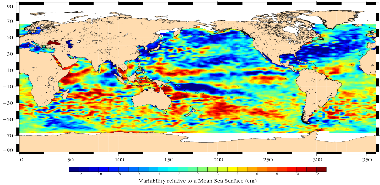
Jason-1 Cycle 302 13/03/2010 – 23/03/2010
