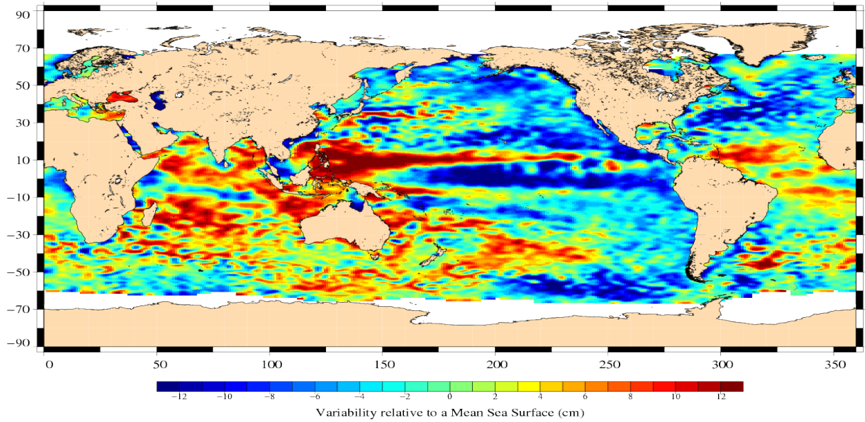
Jason-1 Cycle 312 21/06/2010 – 30/06/2010
