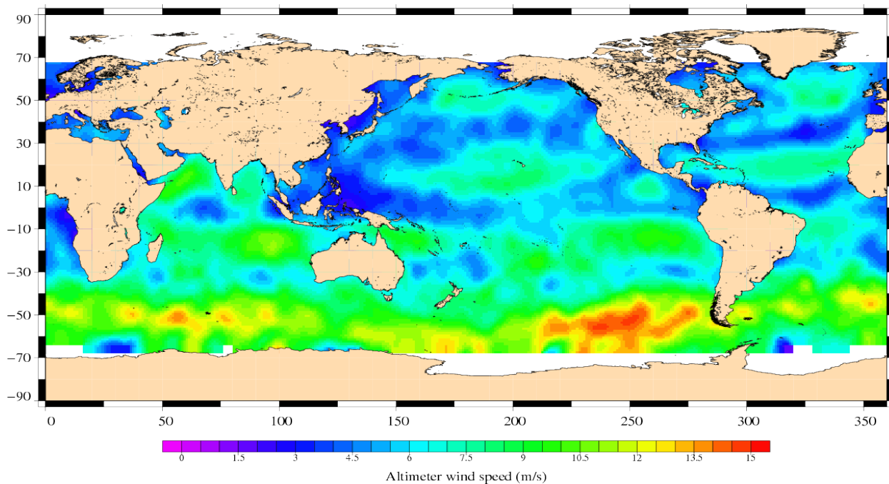
Jason-1 Cycle 312 21/06/2010 – 30/06/2010
