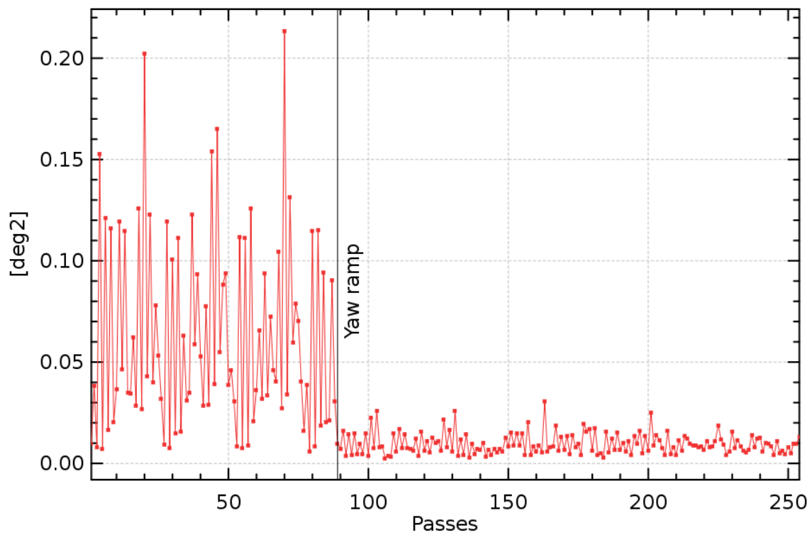
GDR Jason-1 Cycle 322: Mean by pass of apparent squared mispointing
