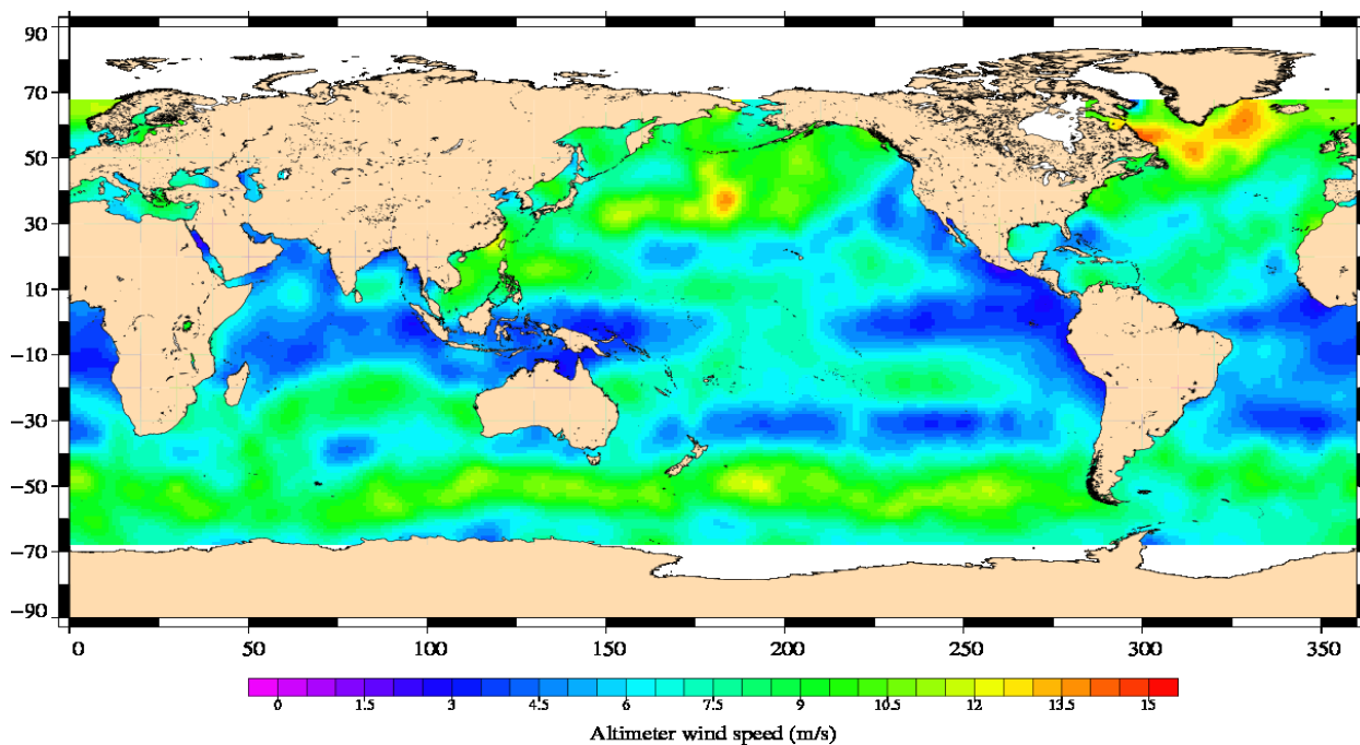
Jason-1 Cycle 334 25/01/2011 - 04/02/2011
